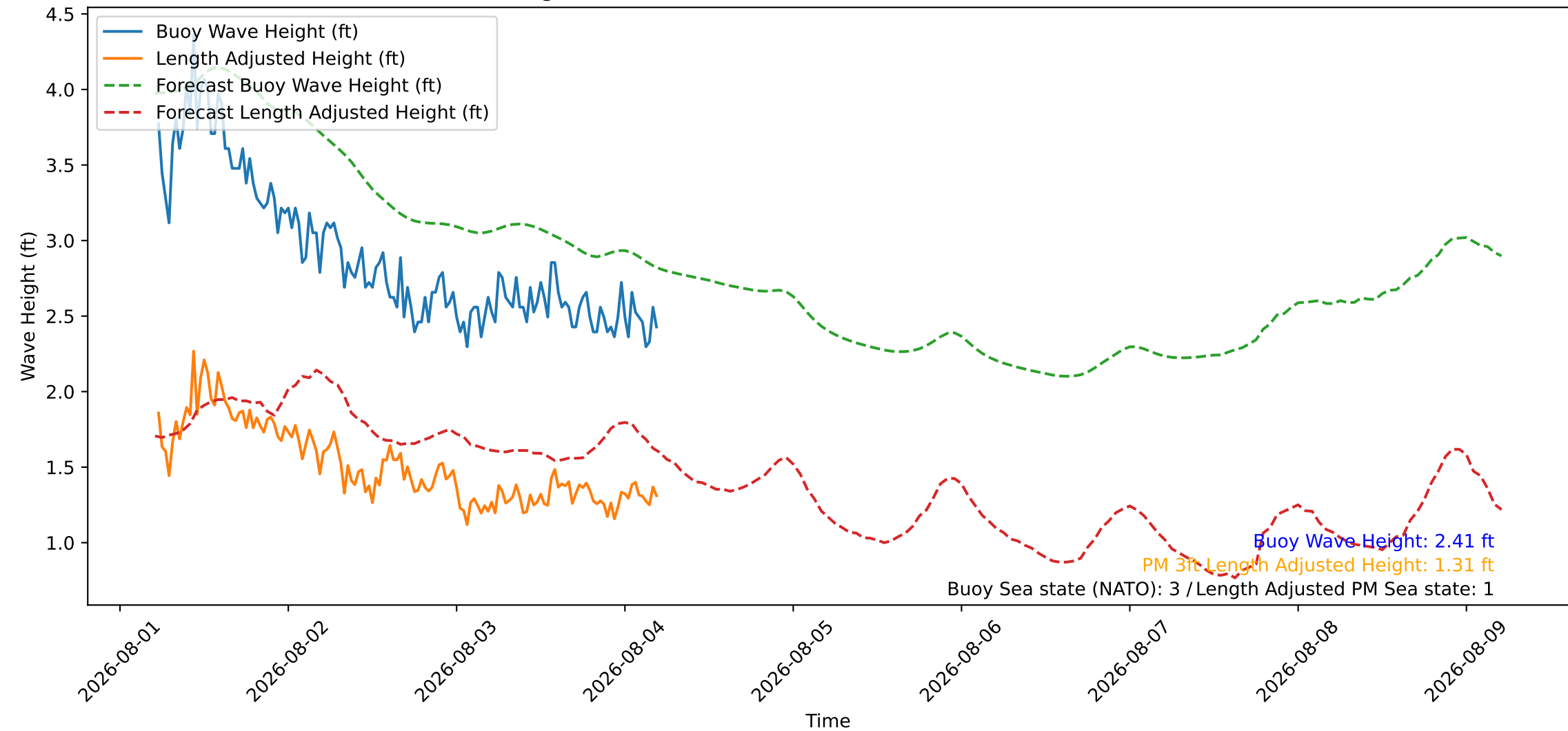
Wave Heights over Time for Oceanside Harbor at 2026-08-04 05:20:26
