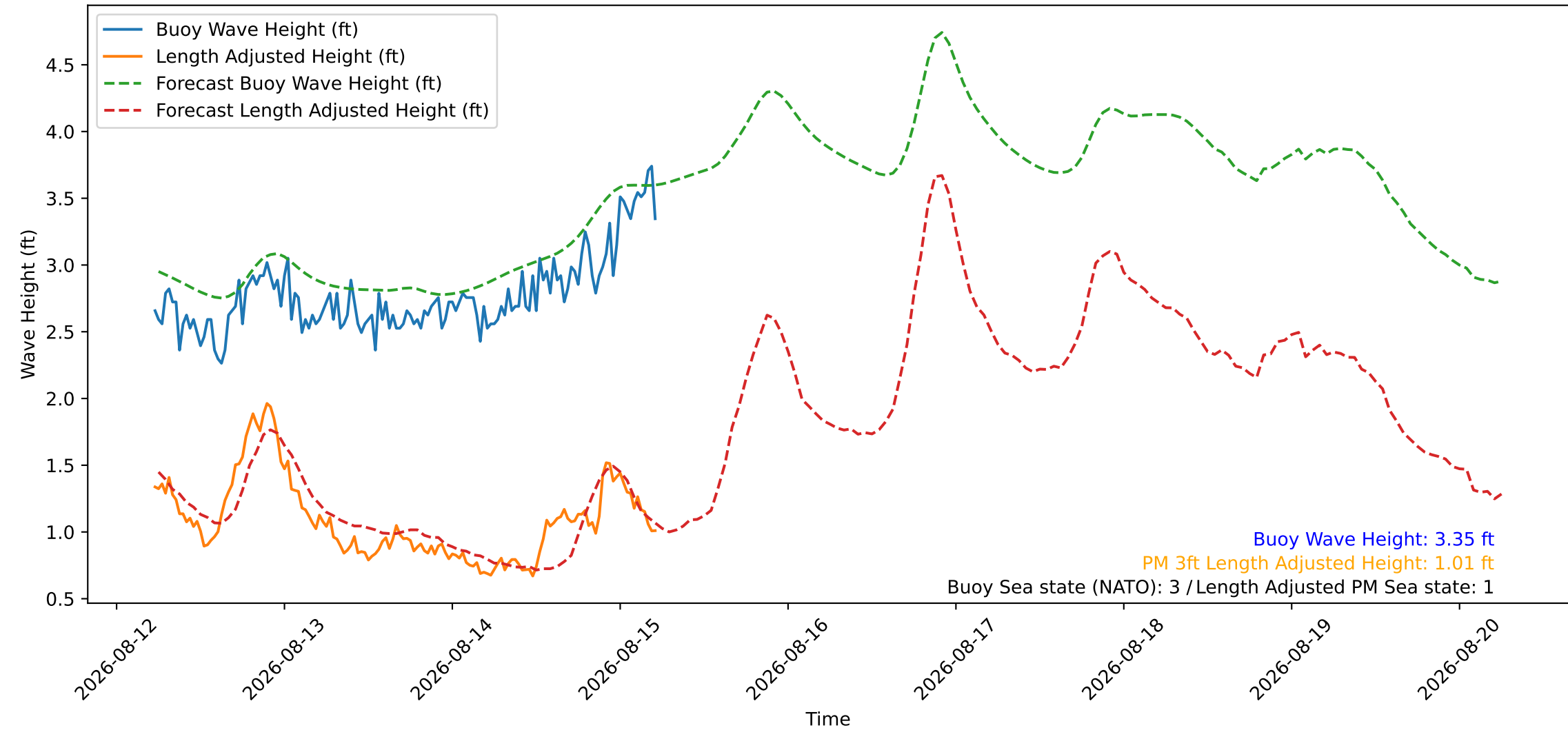
Wave Heights over Time for Green Beach at 2026-08-15 05:41:09
