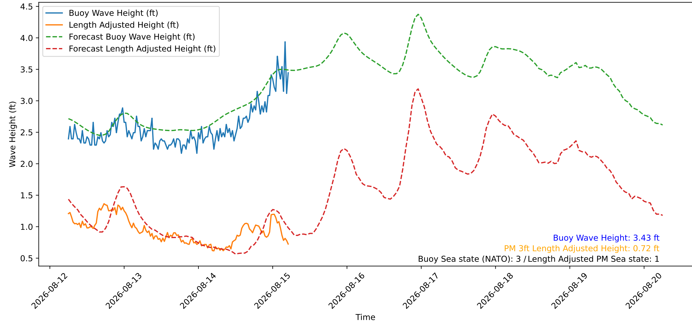
Wave Heights over Time for Red Beach at 2026-08-15 05:40:46
