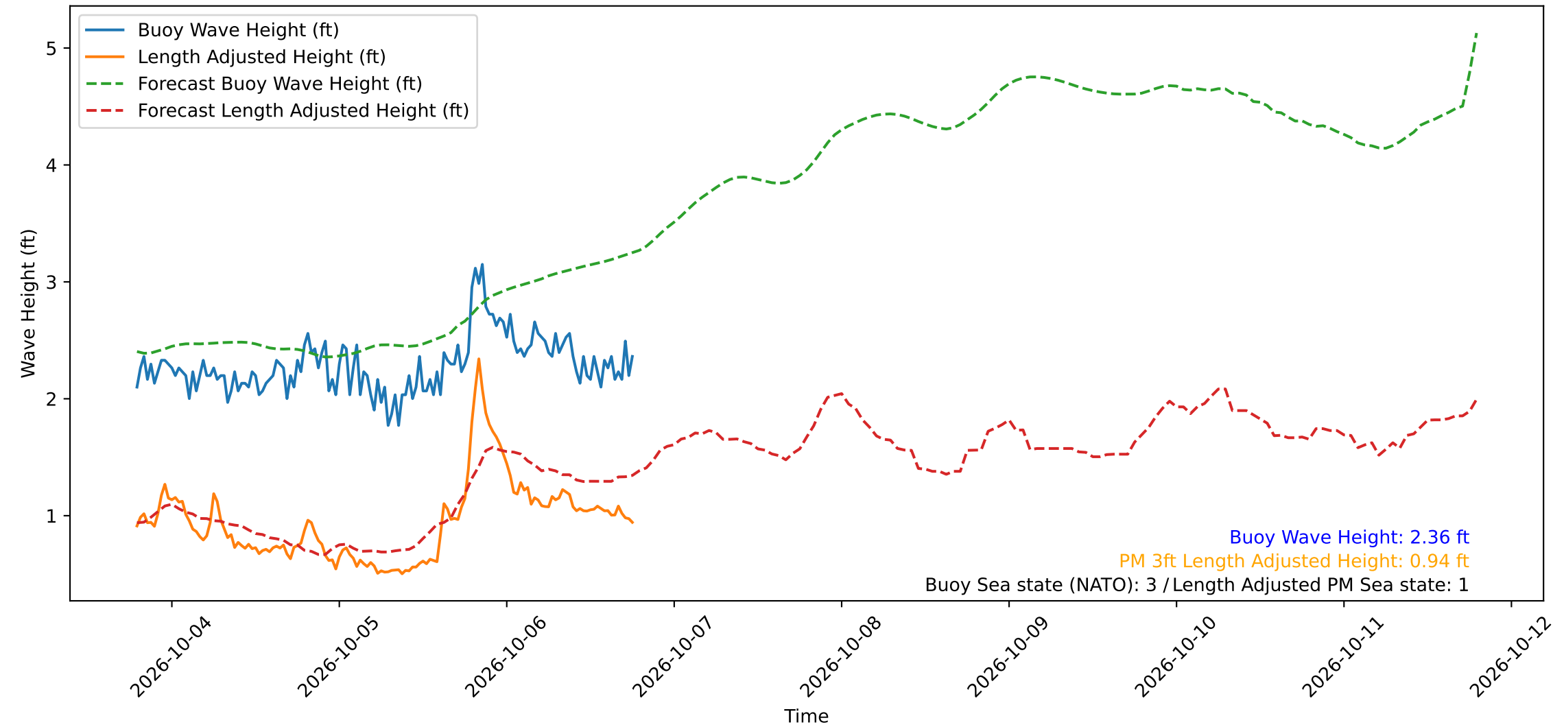
Wave Heights over Time for Green Beach at 2026-10-06 18:41:12
