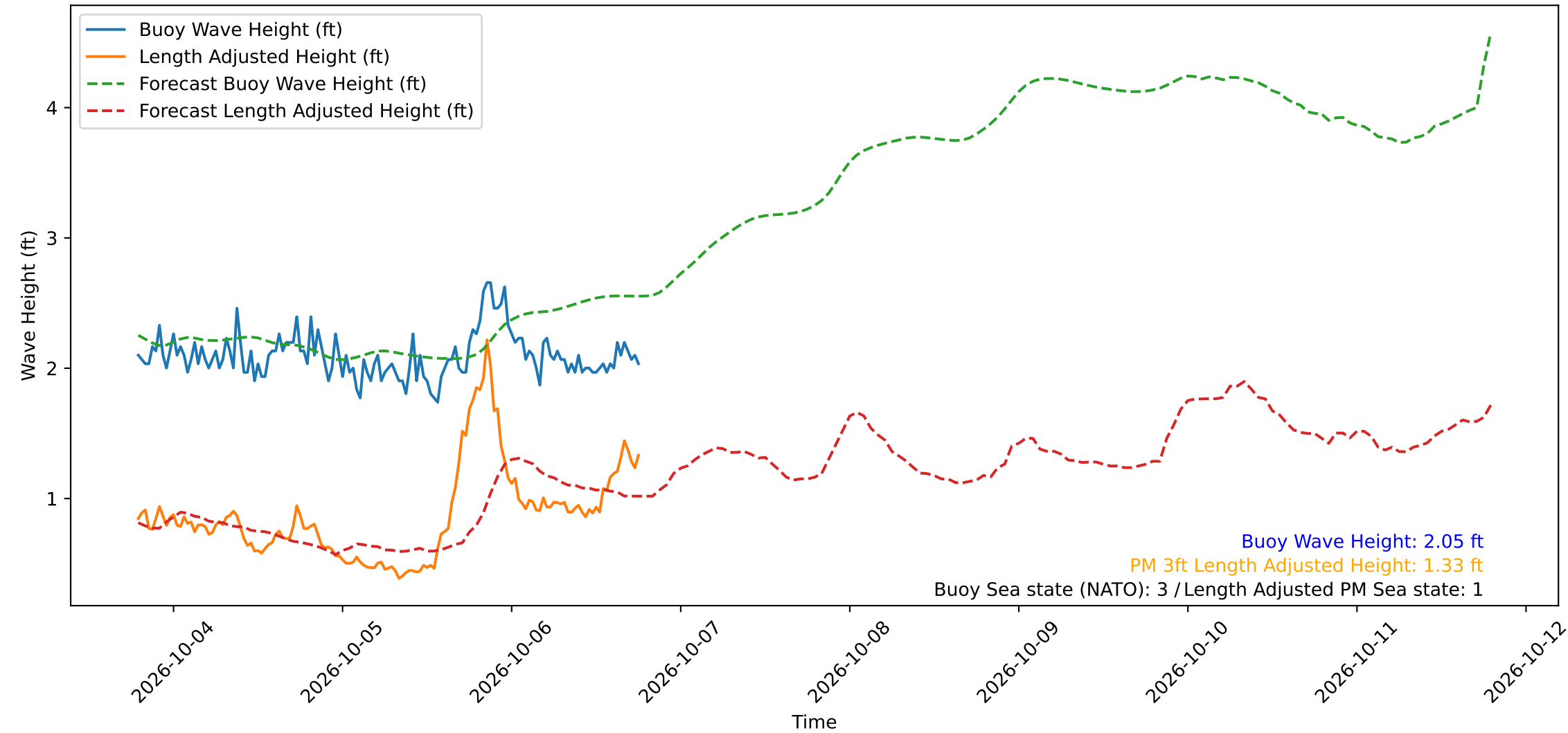
Wave Heights over Time for Red Beach at 2026-10-06 18:40:50
