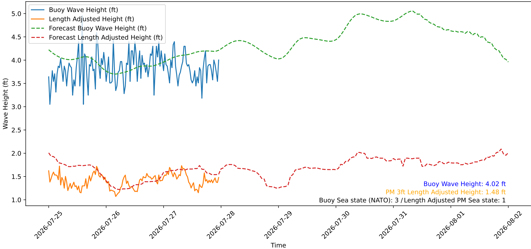
Wave Heights over Time for Oceanside Harbor at 2026-07-28 00:10:26
