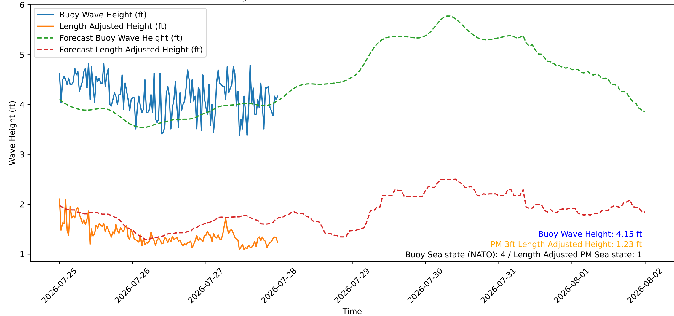
Wave Heights over Time for Green Beach at 2026-07-28 00:11:08
