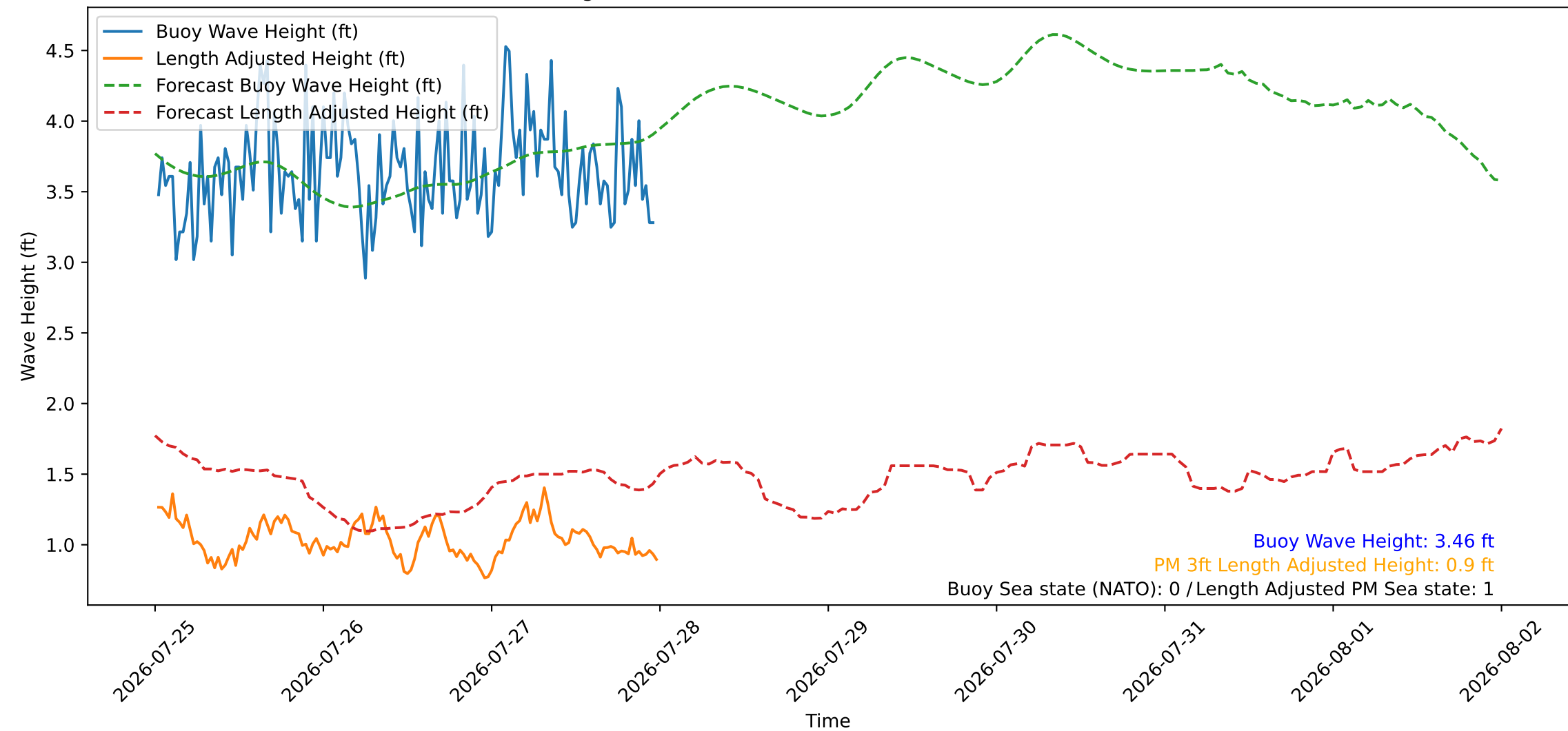
Wave Heights over Time for Red Beach at 2026-07-28 00:10:45
