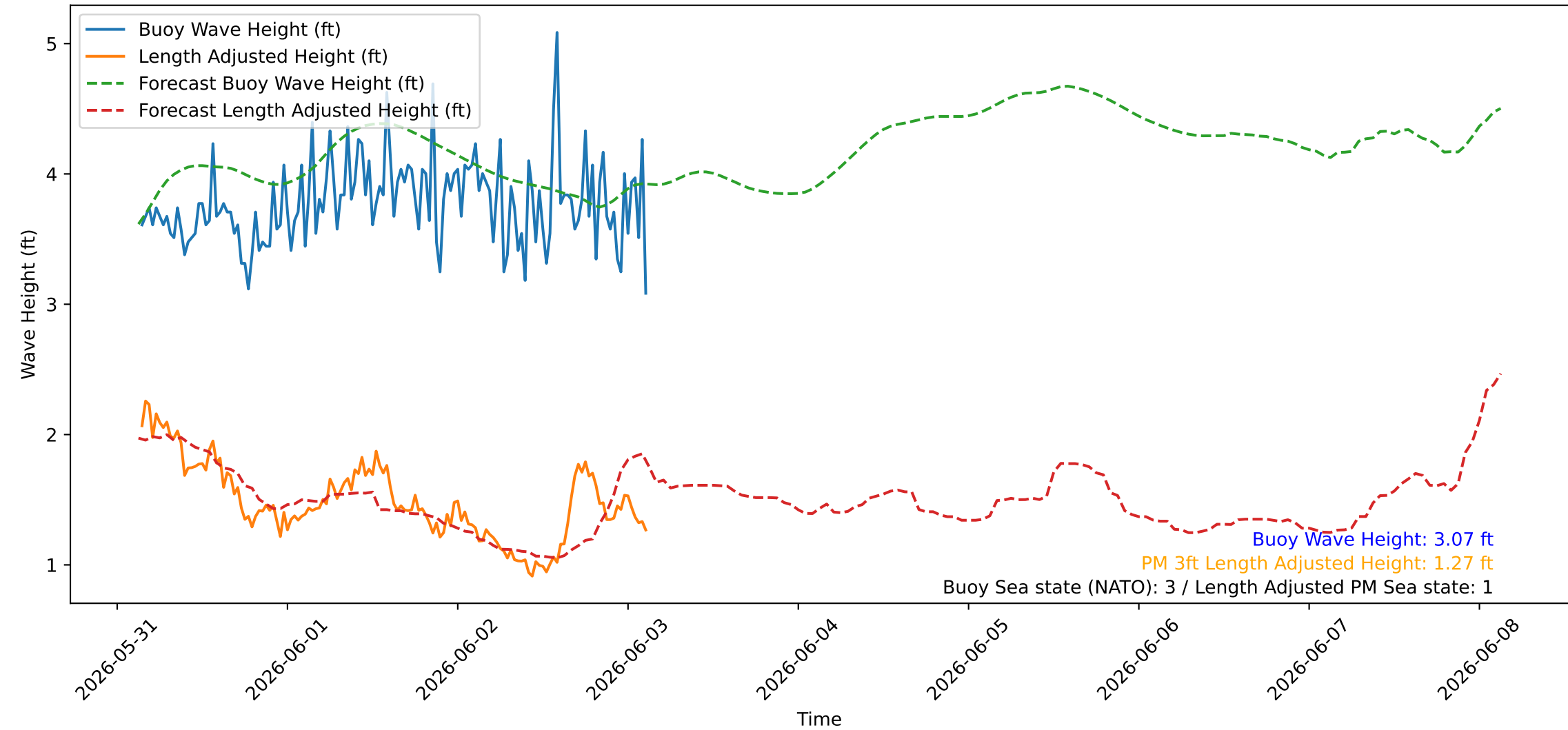
Wave Heights over Time for Oceanside Harbor at 2026-06-03 03:20:26
