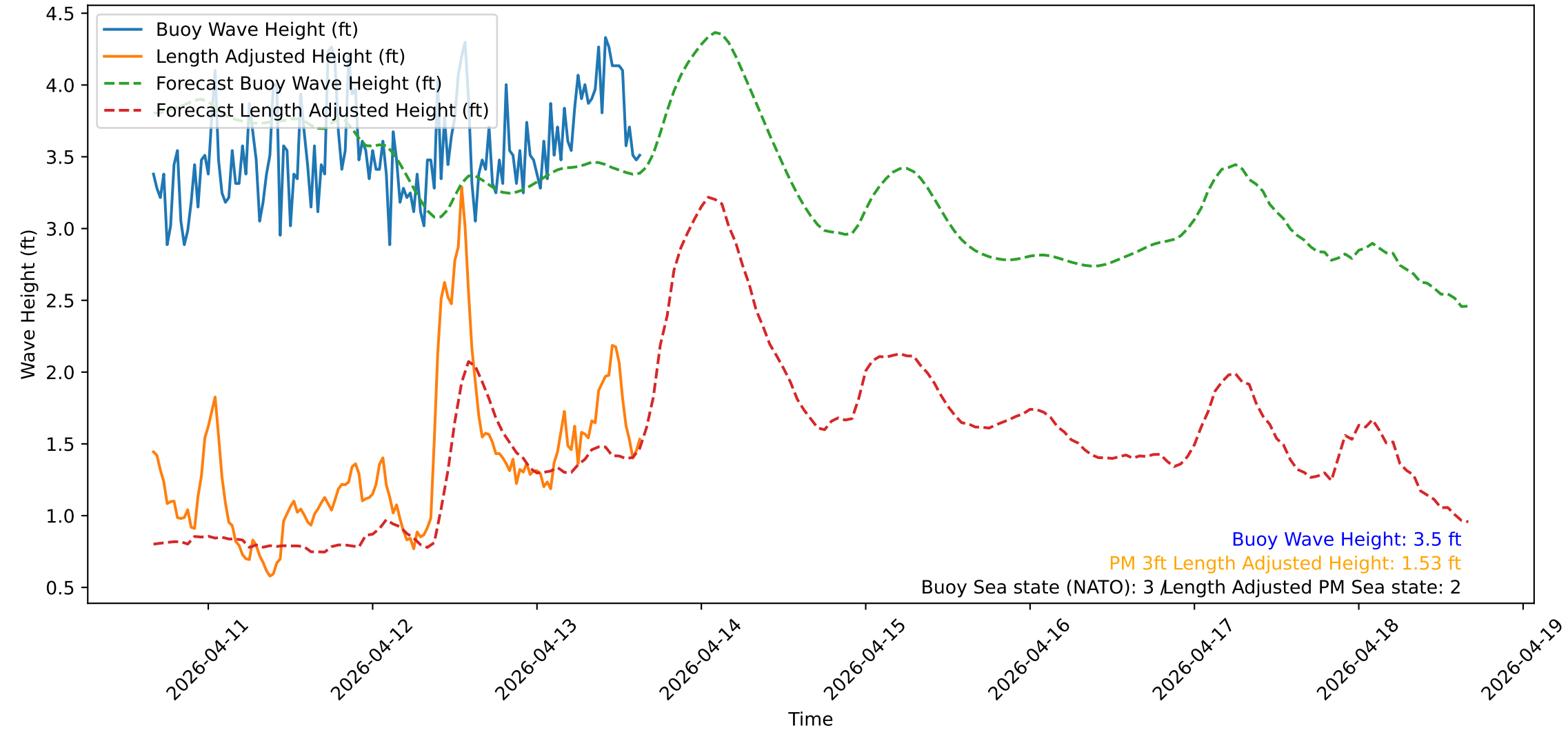
Wave Heights over Time for Red Beach at 2026-04-13 15:50:51
