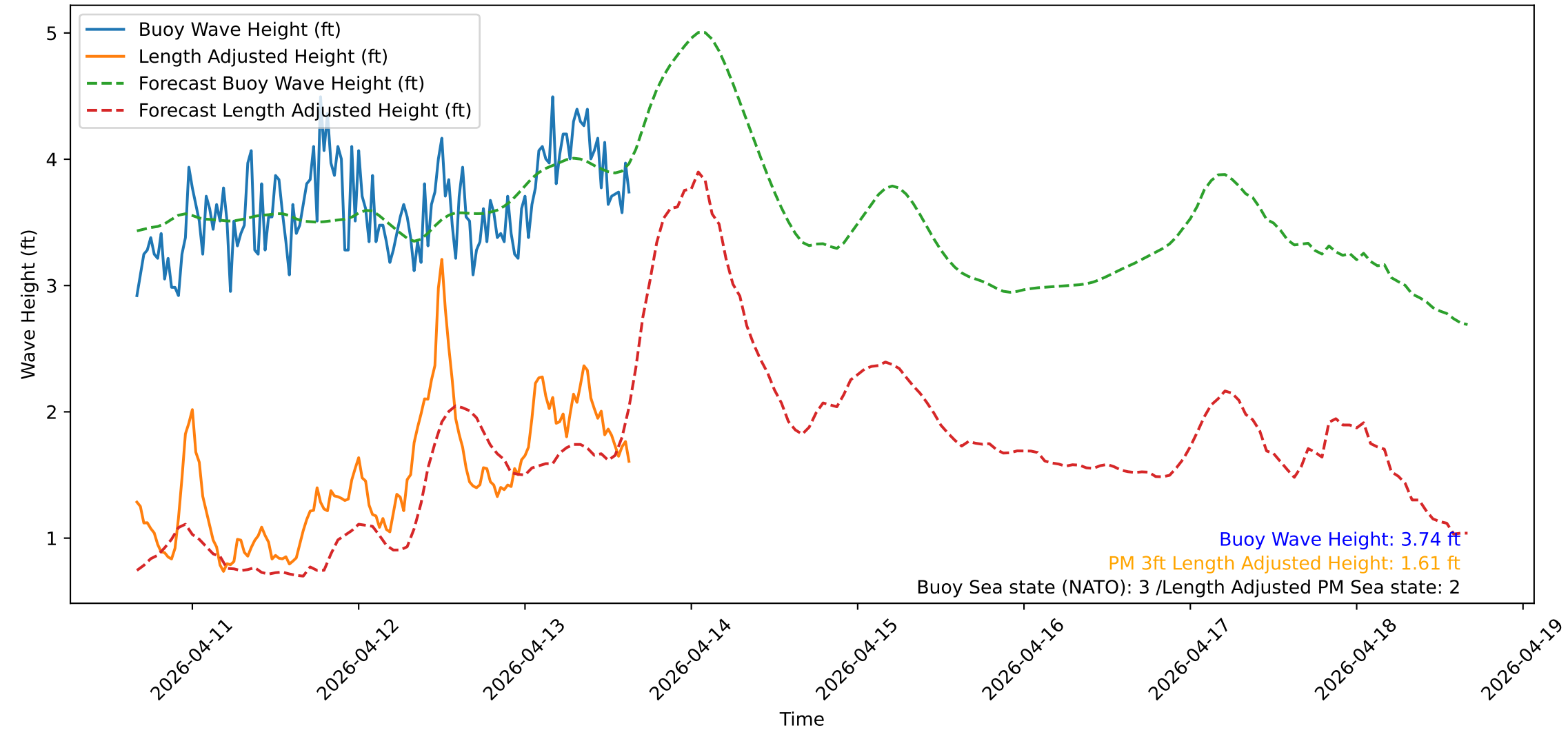
Wave Heights over Time for Green Beach at 2026-04-13 15:51:13
