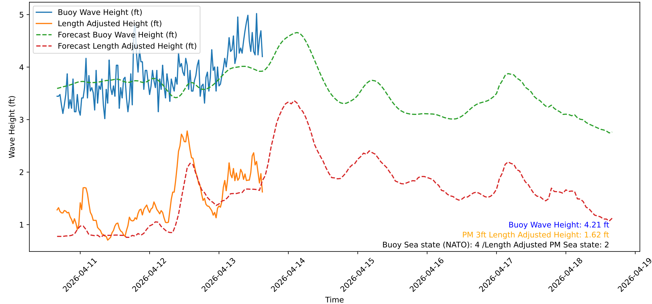
Wave Heights over Time for Oceanside Harbor at 2026-04-13 15:50:31
