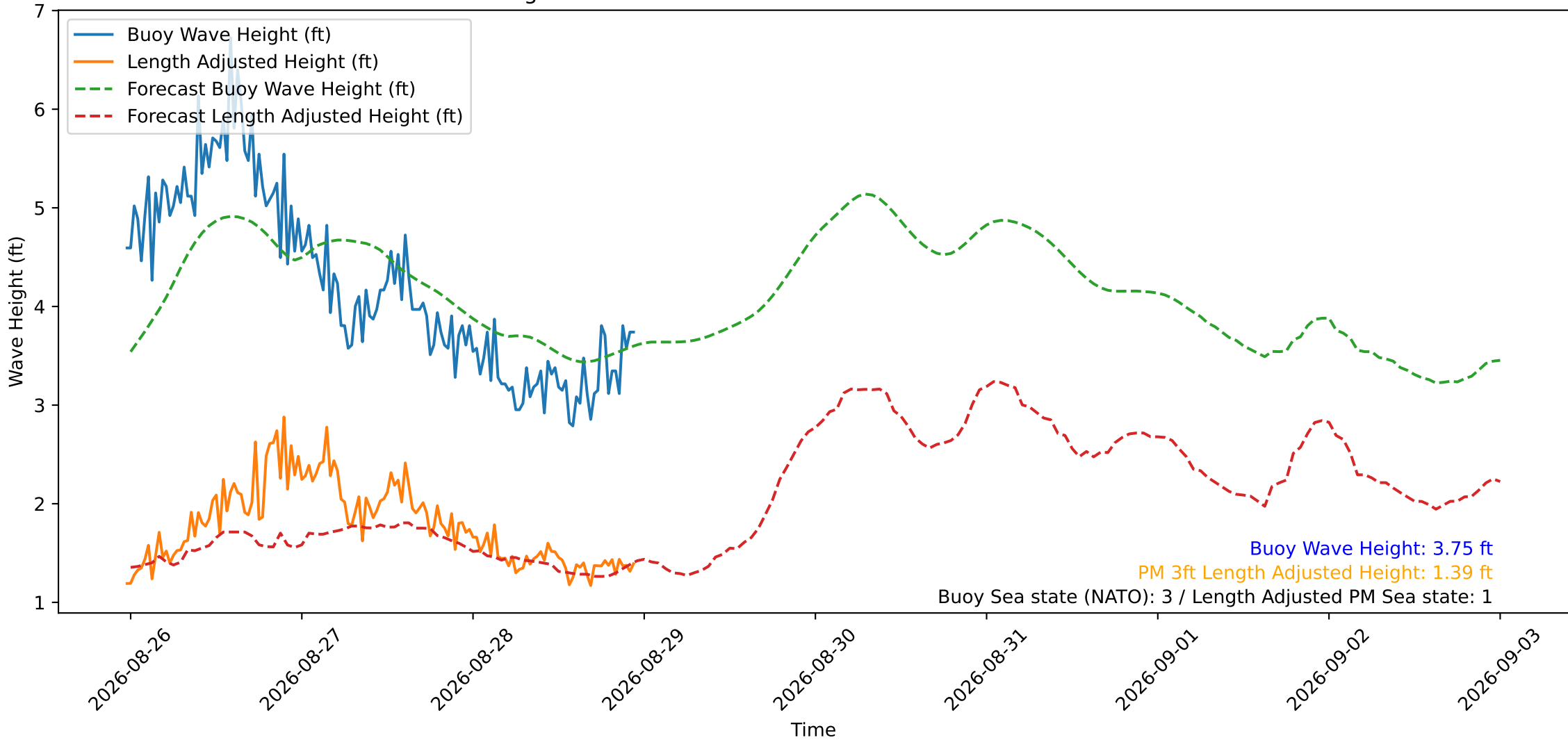
Wave Heights over Time for Oceanside Harbor at 2026-08-28 23:40:29
