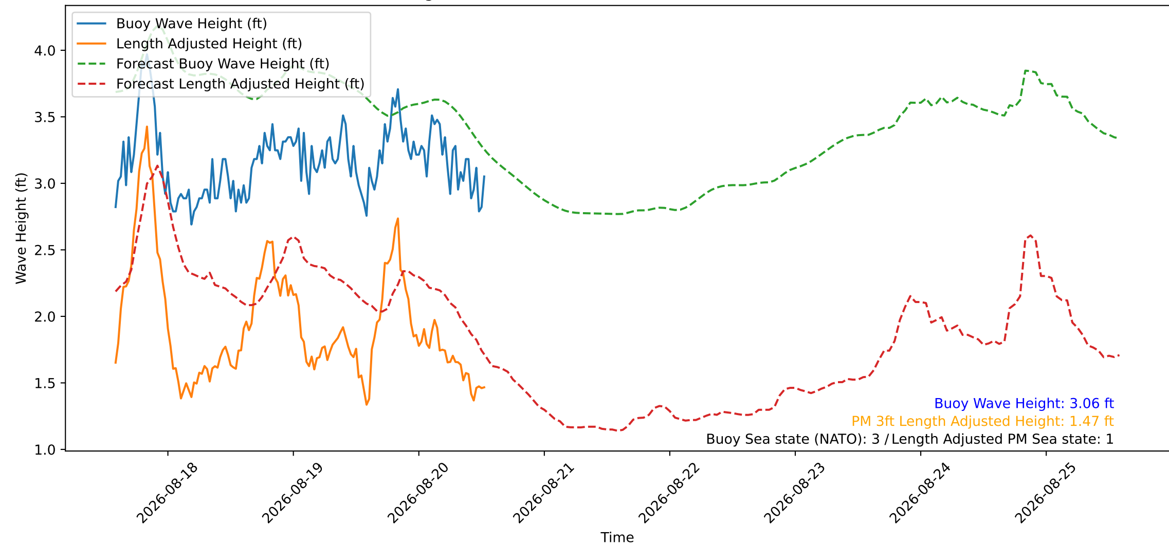
Wave Heights over Time for Green Beach at 2026-08-20 13:51:11
