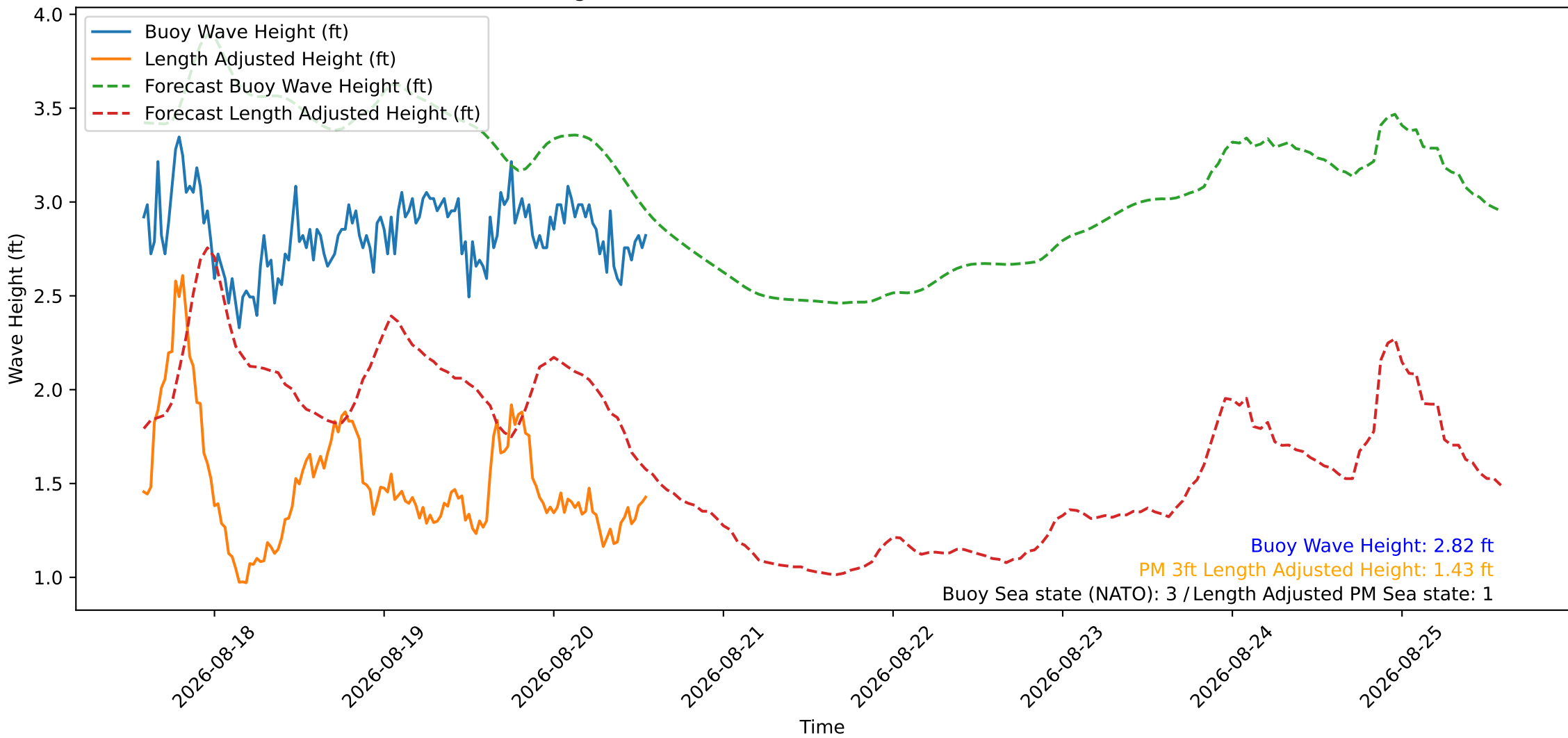
Wave Heights over Time for Red Beach at 2026-08-20 13:50:47
