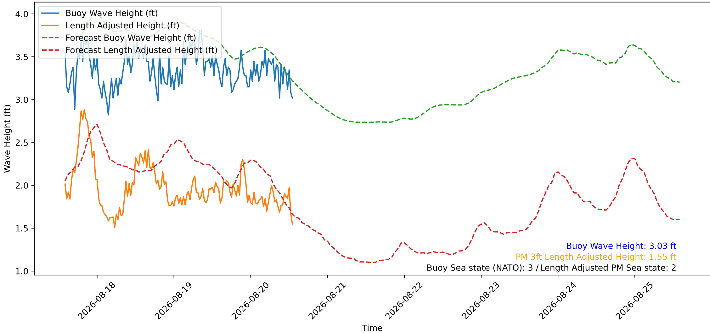
Wave Heights over Time for Oceanside Harbor at 2026-08-20 13:50:27
