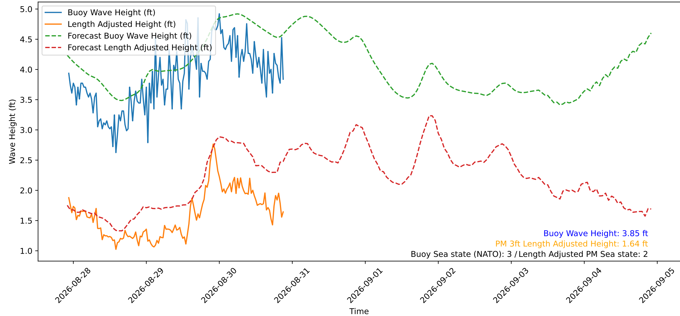
Wave Heights over Time for Green Beach at 2026-08-30 22:01:12
