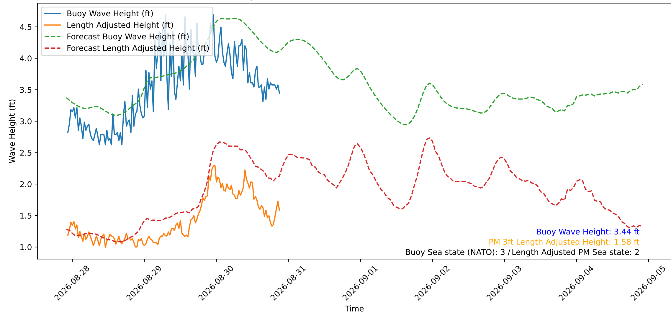
Wave Heights over Time for Red Beach at 2026-08-30 22:00:49
