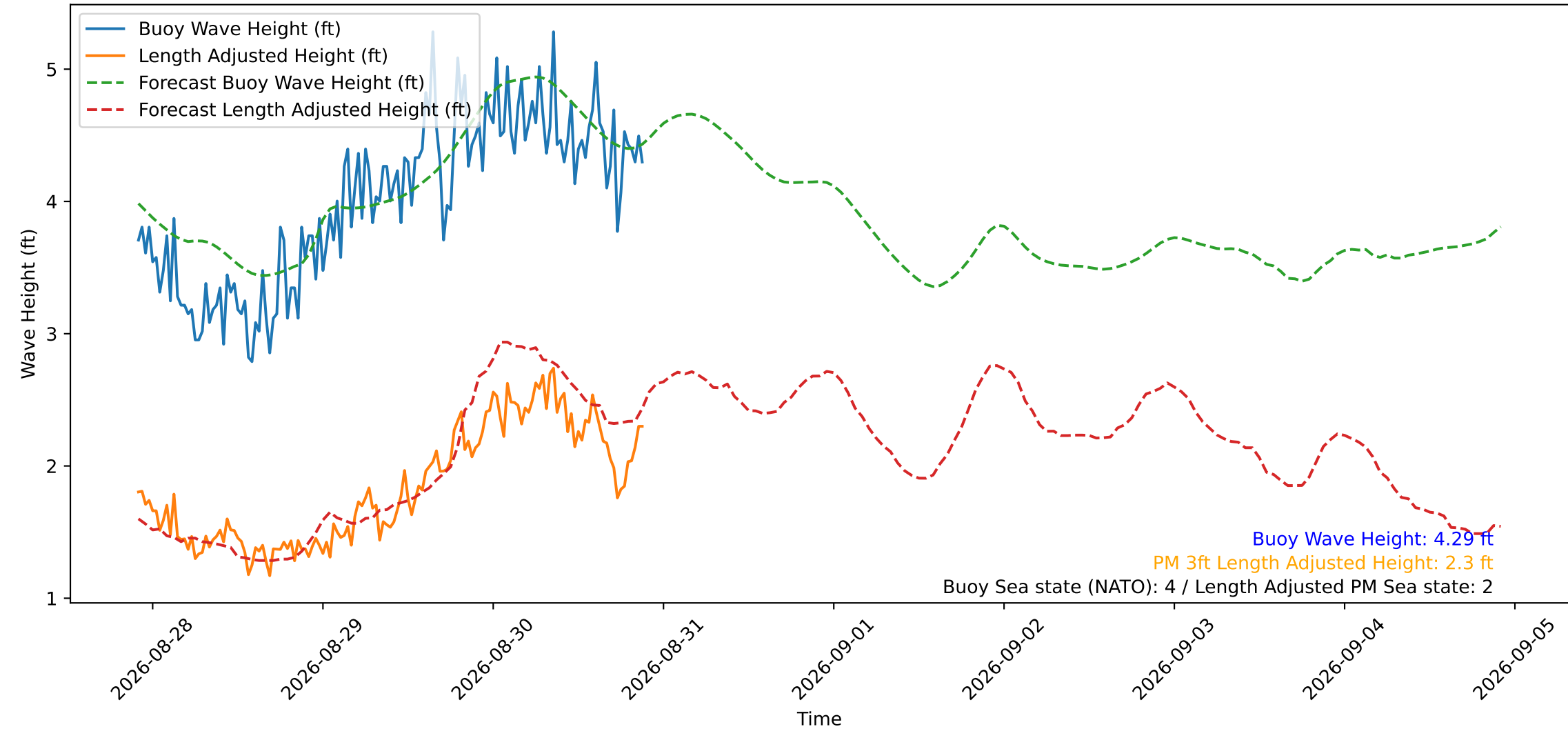
Wave Heights over Time for Oceanside Harbor at 2026-08-30 22:00:29
