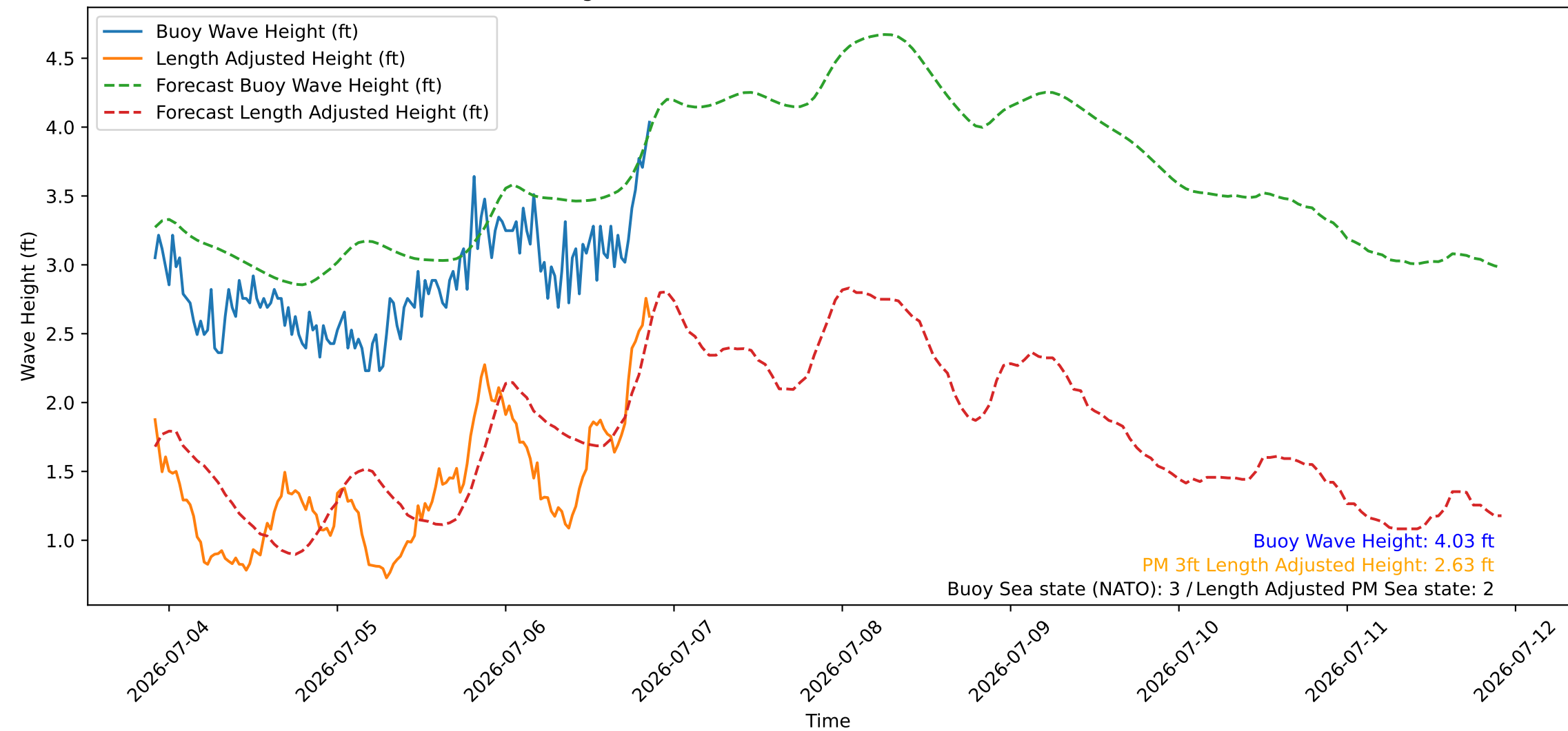
Wave Heights over Time for Red Beach at 2026-07-06 21:30:46
