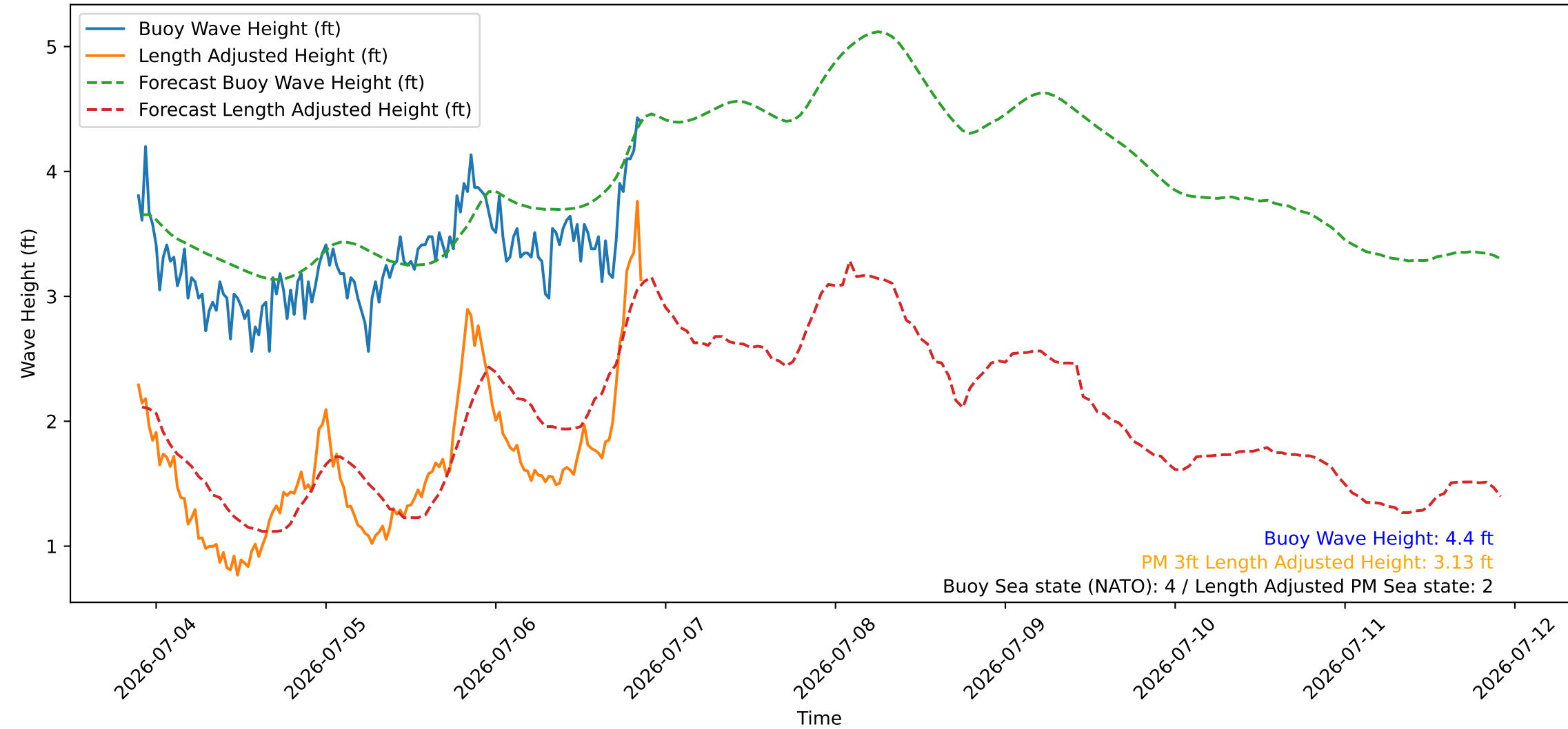
Wave Heights over Time for Green Beach at 2026-07-06 21:31:09
