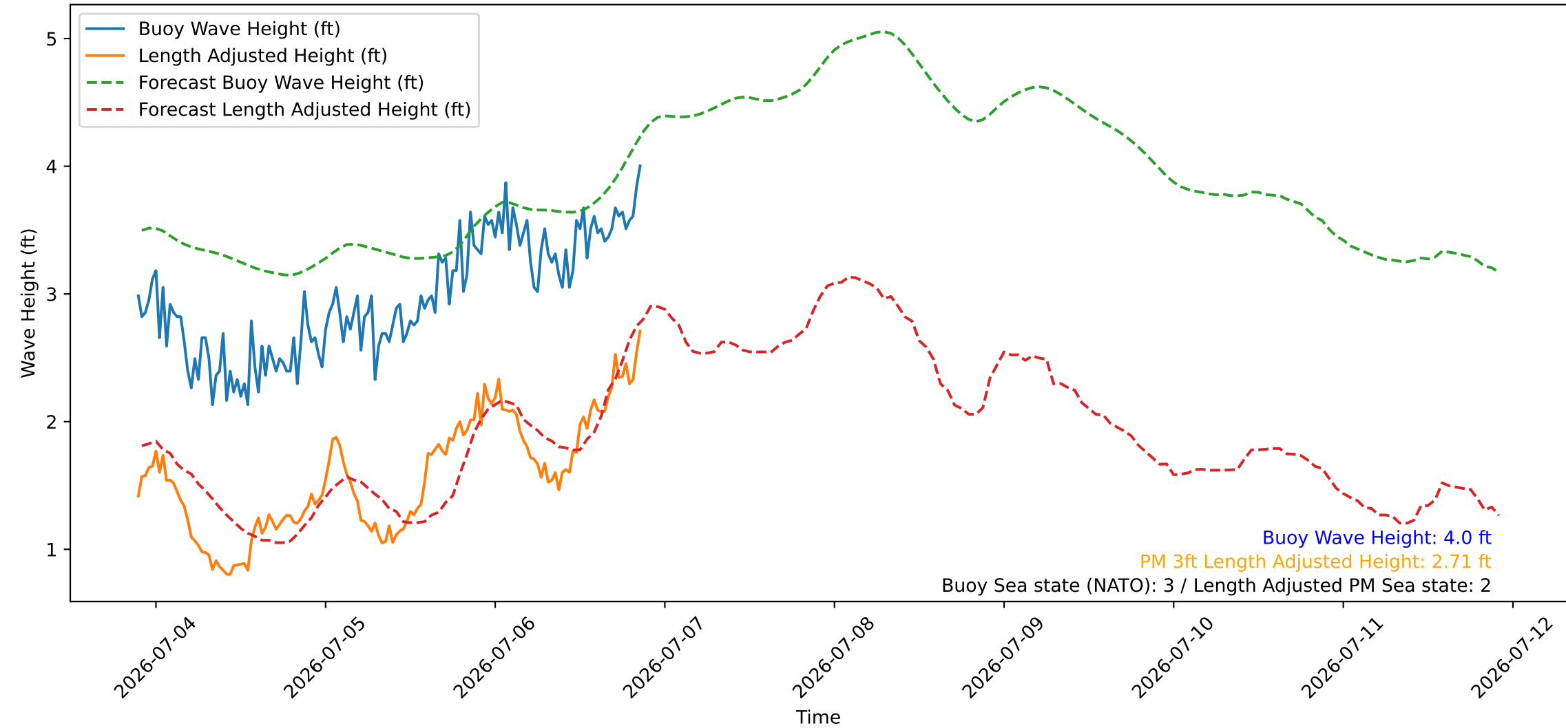
Wave Heights over Time for Oceanside Harbor at 2026-07-06 21:30:27
