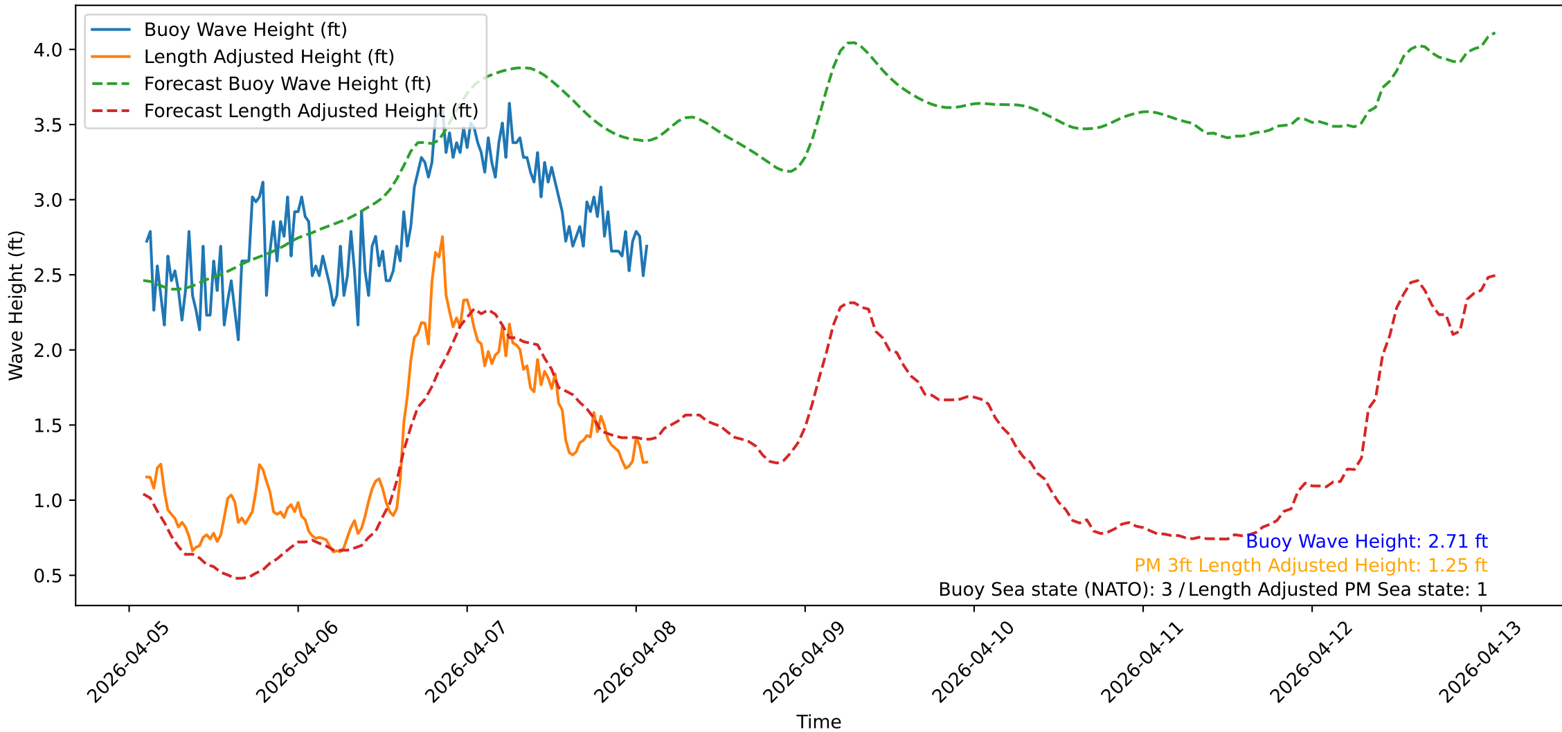
Wave Heights over Time for Oceanside Harbor at 2026-04-08 02:20:31
