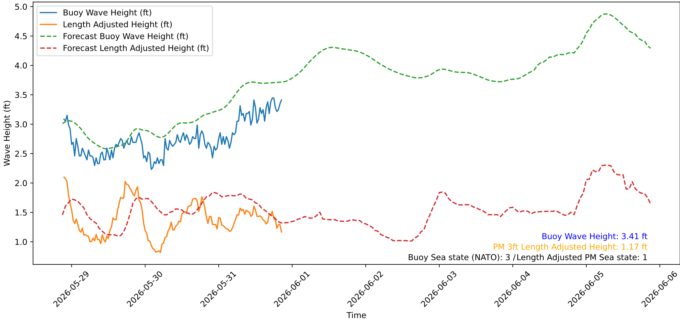
Wave Heights over Time for Red Beach at 2026-05-31 21:10:45
