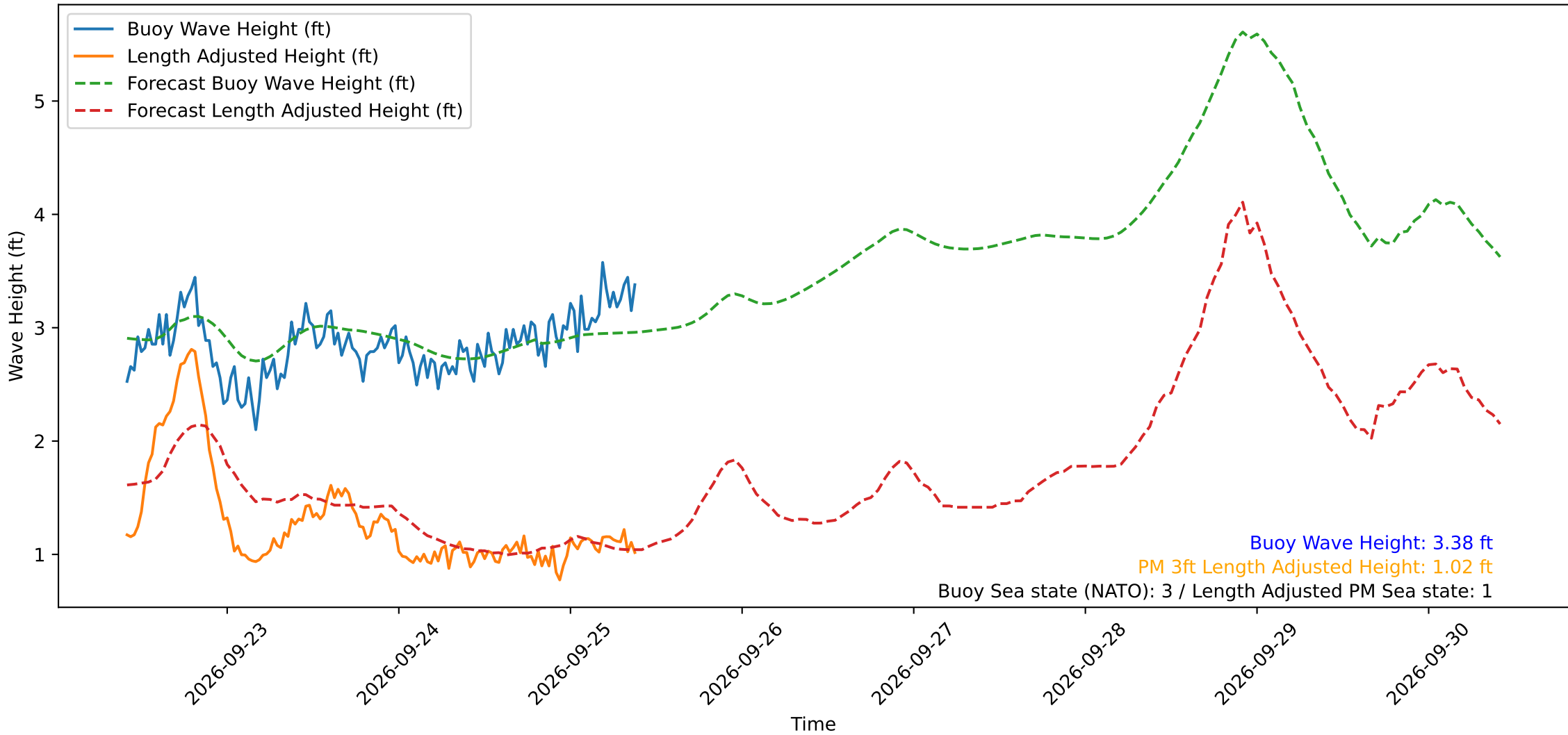
Wave Heights over Time for Green Beach at 2026-09-25 09:41:11
