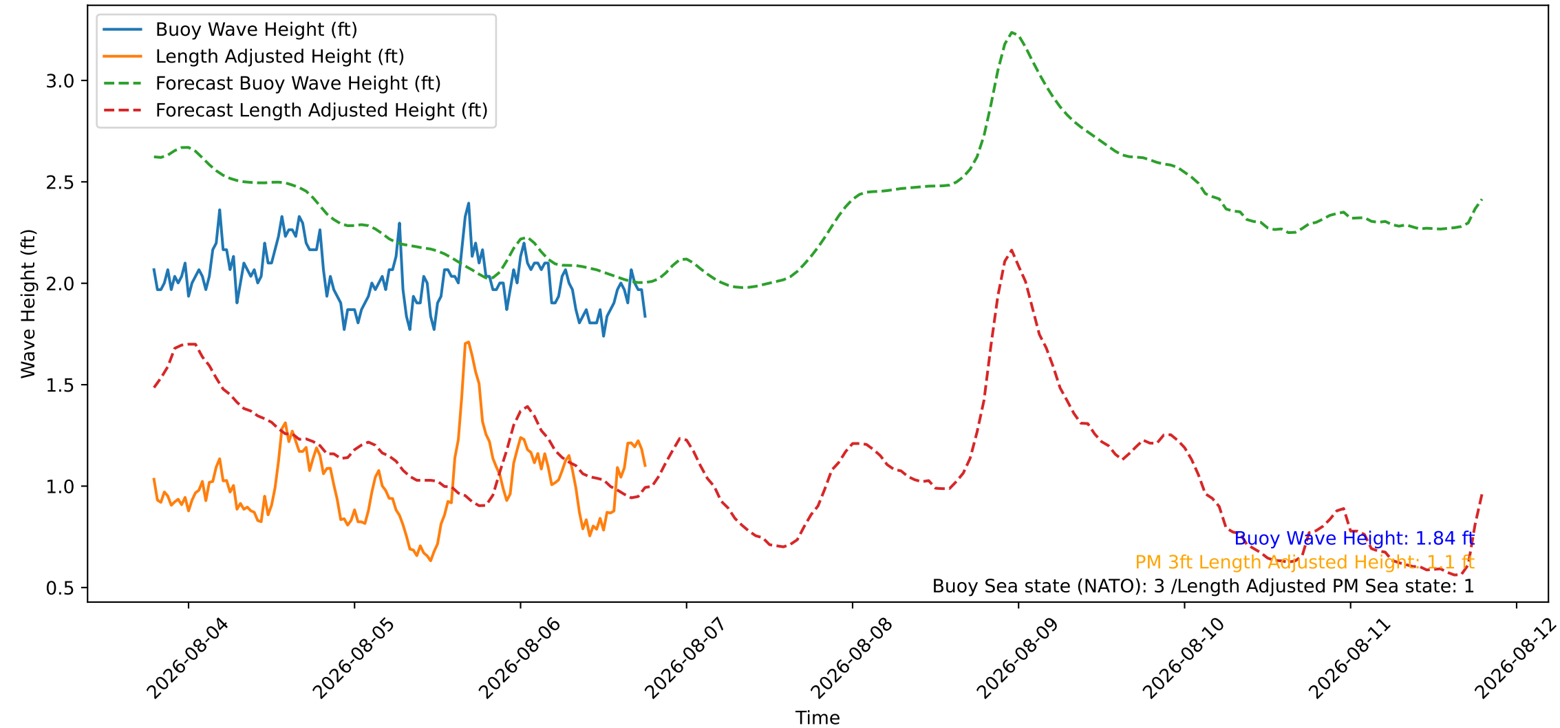
Wave Heights over Time for Red Beach at 2026-08-06 18:50:47
