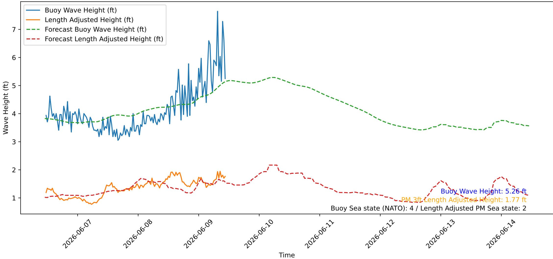
Wave Heights over Time for Red Beach at 2026-06-09 11:10:45
