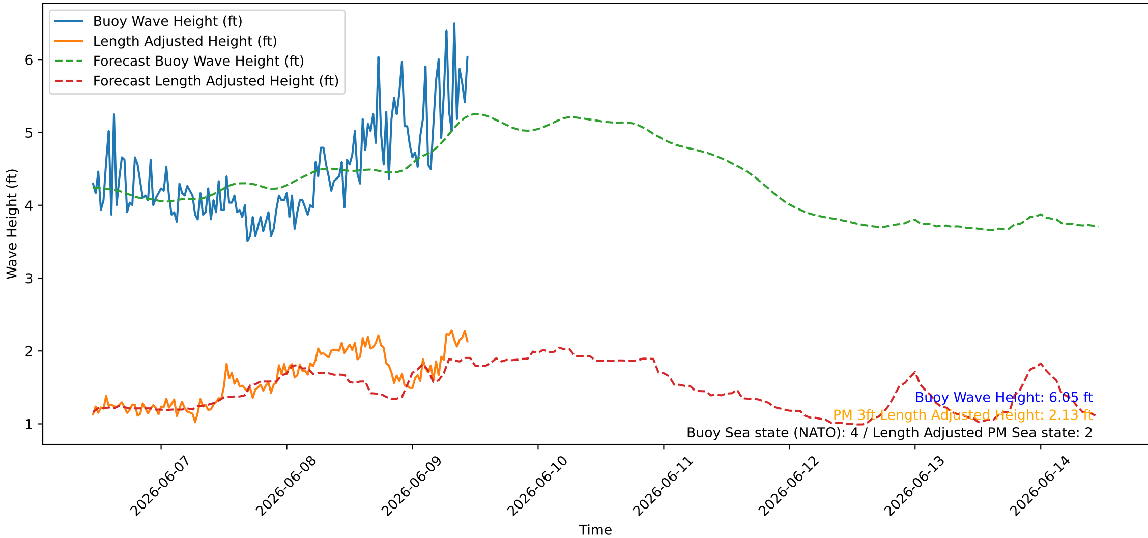
Wave Heights over Time for Oceanside Harbor at 2026-06-09 11:10:25
