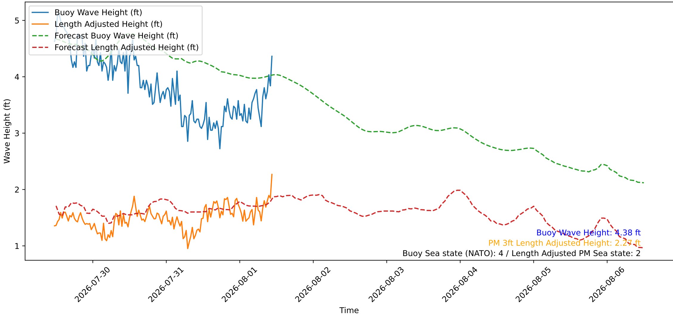
Wave Heights over Time for Oceanside Harbor at 2026-08-01 11:30:26
