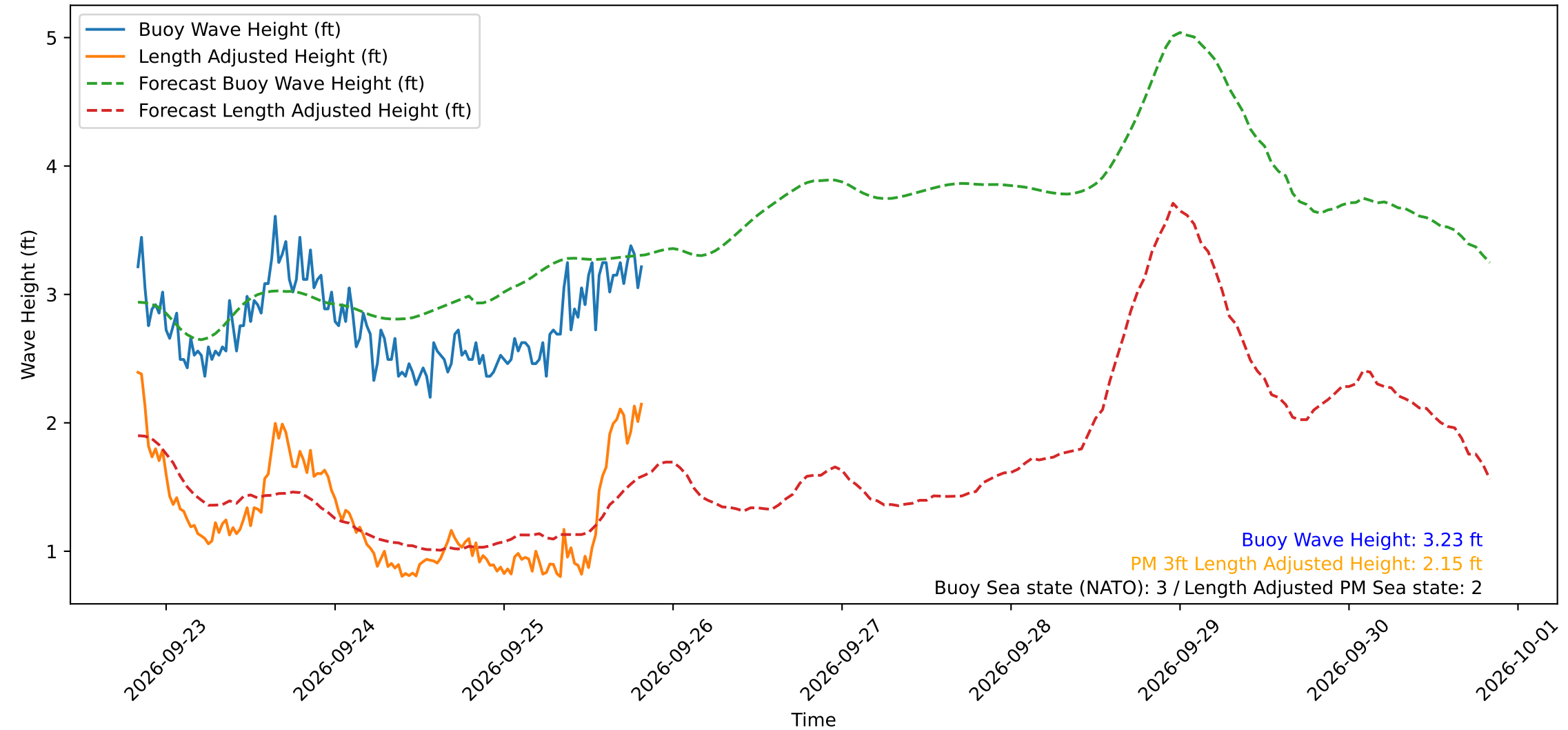
Wave Heights over Time for Oceanside Harbor at 2026-09-25 20:00:29
