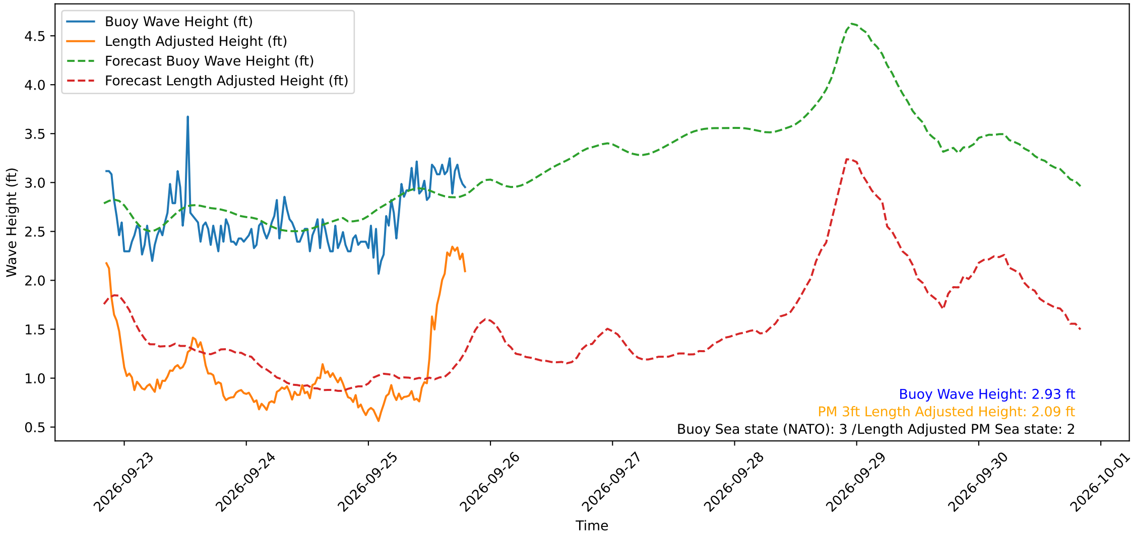
Wave Heights over Time for Red Beach at 2026-09-25 20:00:48
