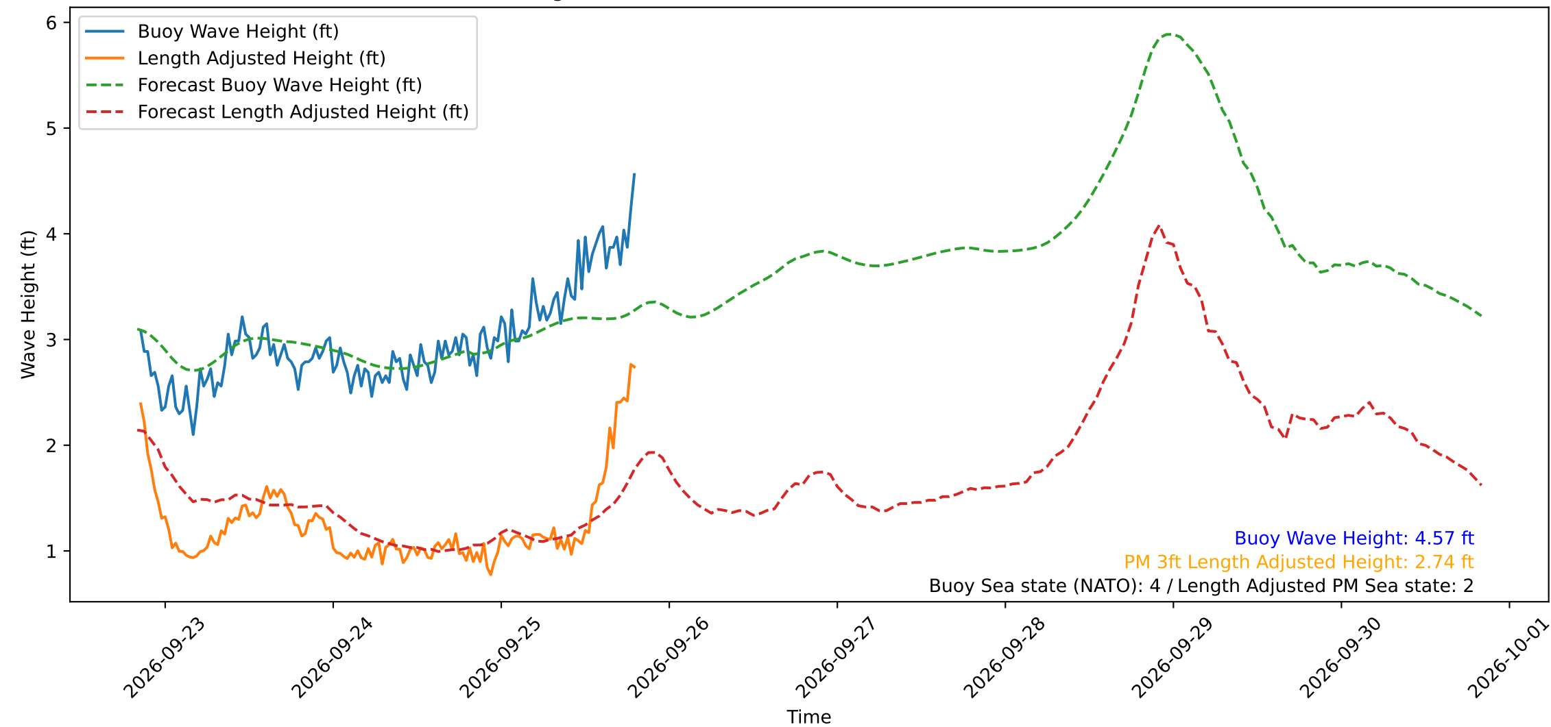
Wave Heights over Time for Green Beach at 2026-09-25 20:01:11
