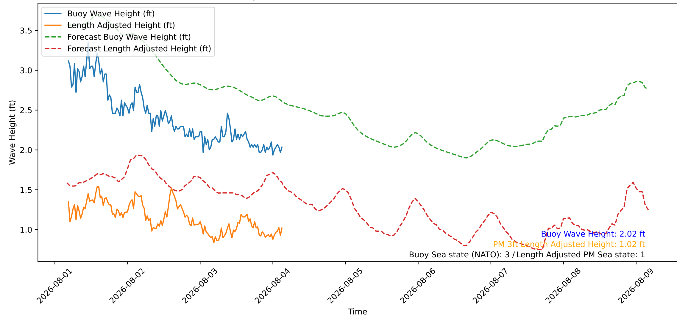
Wave Heights over Time for Red Beach at 2026-08-04 04:00:45
