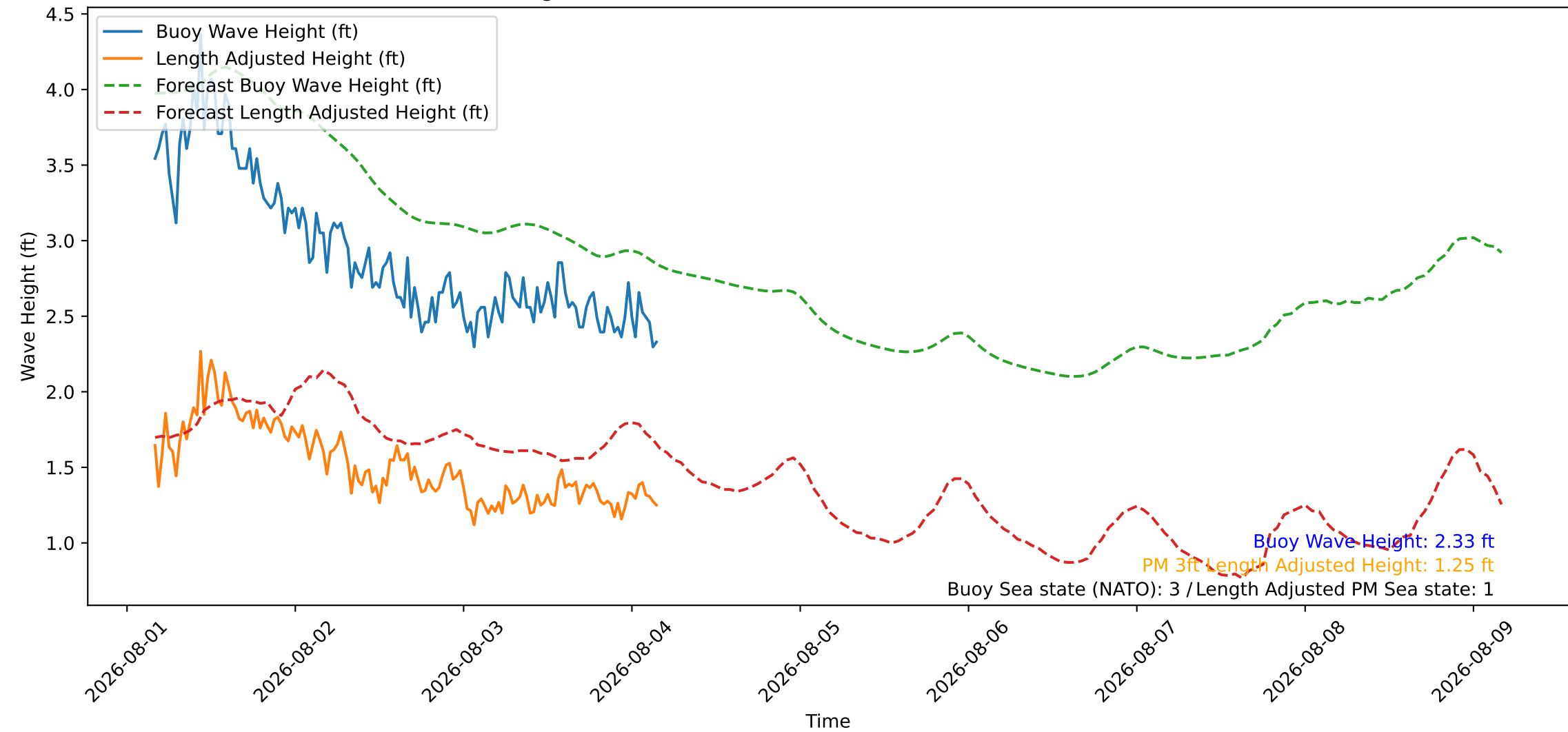
Wave Heights over Time for Oceanside Harbor at 2026-08-04 04:00:26
