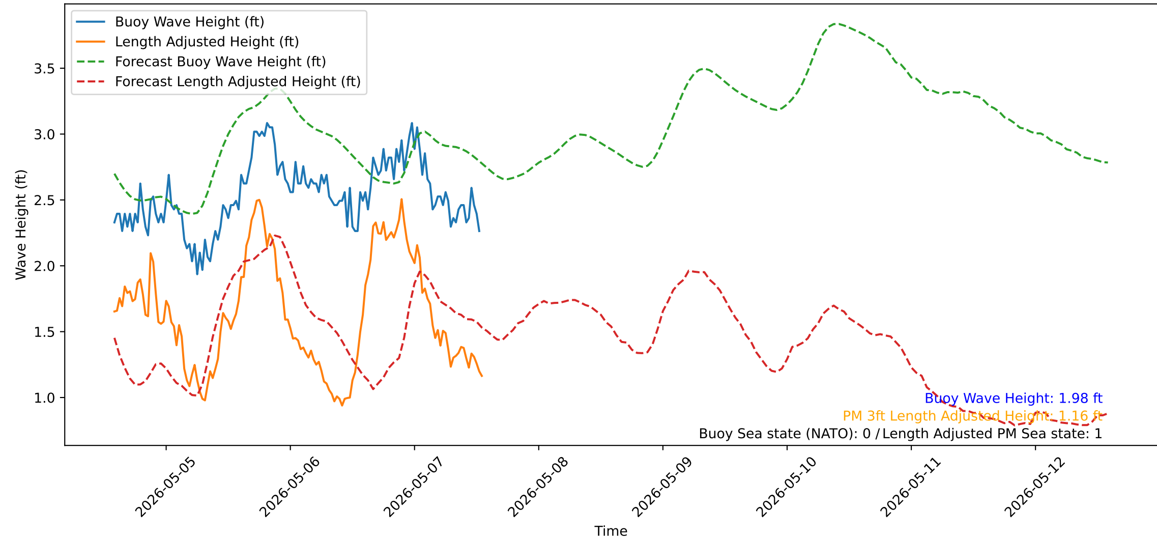
Wave Heights over Time for Red Beach at 2026-05-07 13:50:53
