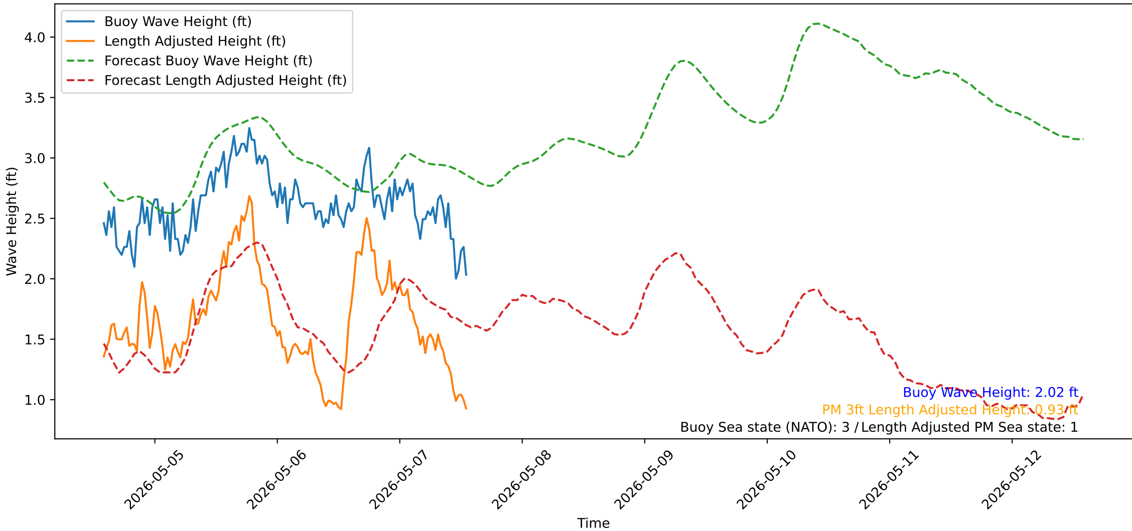
Wave Heights over Time for Oceanside Harbor at 2026-05-07 13:50:31
