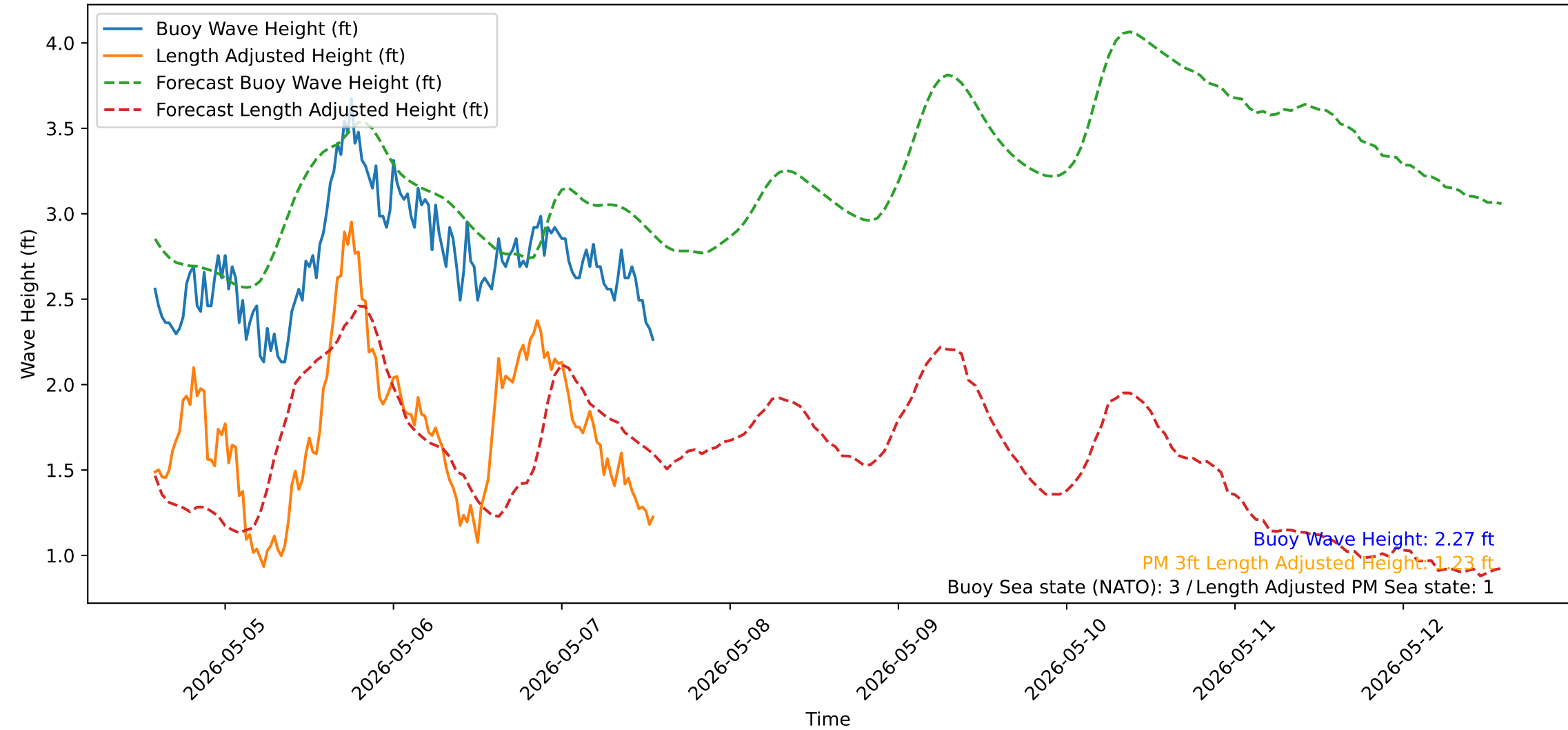
Wave Heights over Time for Green Beach at 2026-05-07 13:51:16
