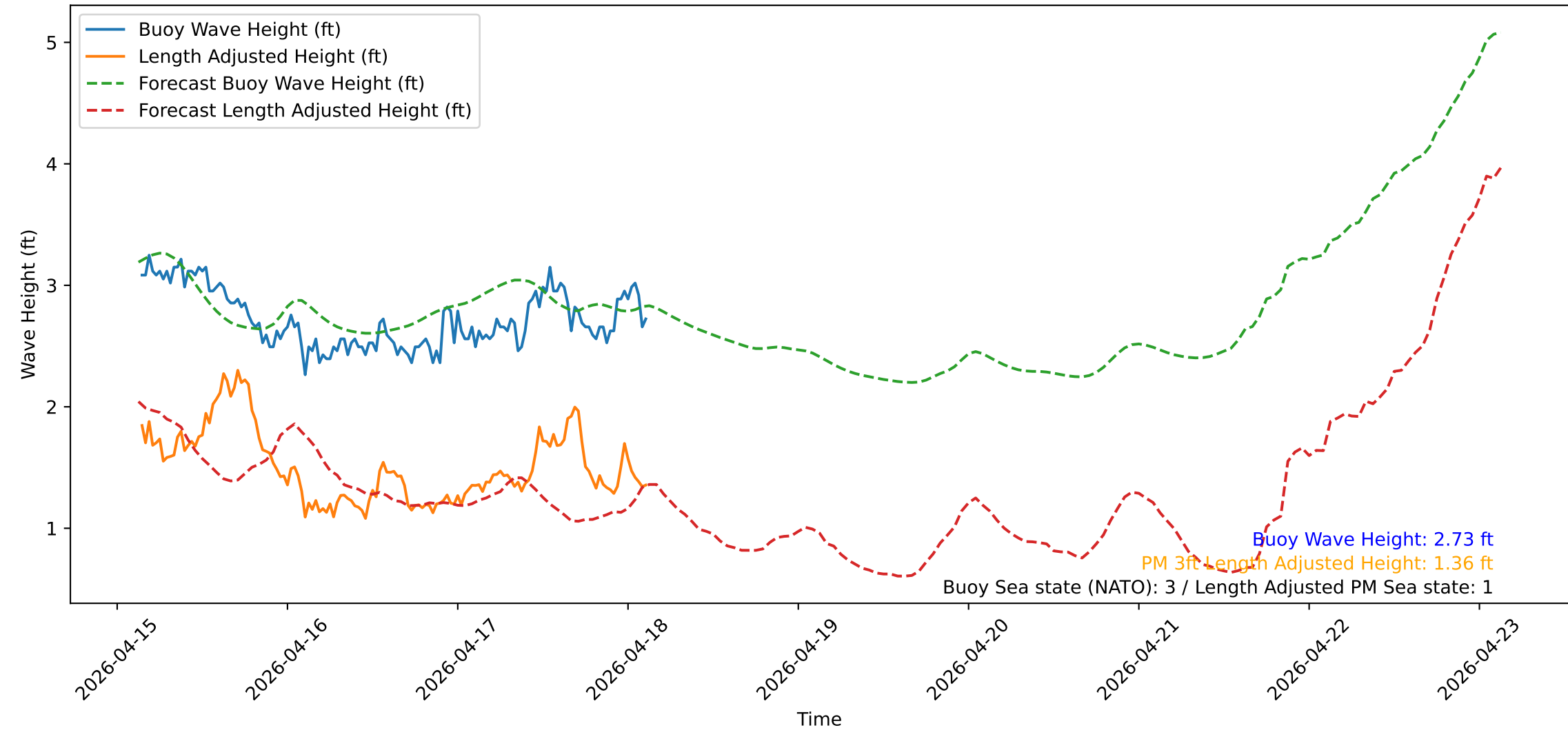
Wave Heights over Time for Red Beach at 2026-04-18 03:10:50
