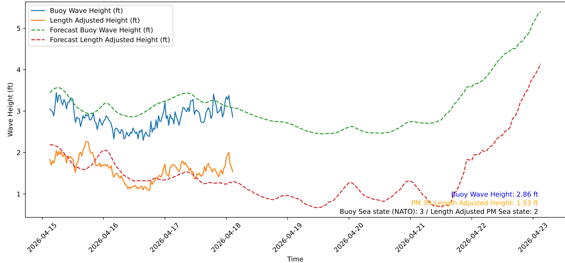
Wave Heights over Time for Oceanside Harbor at 2026-04-18 03:10:31
