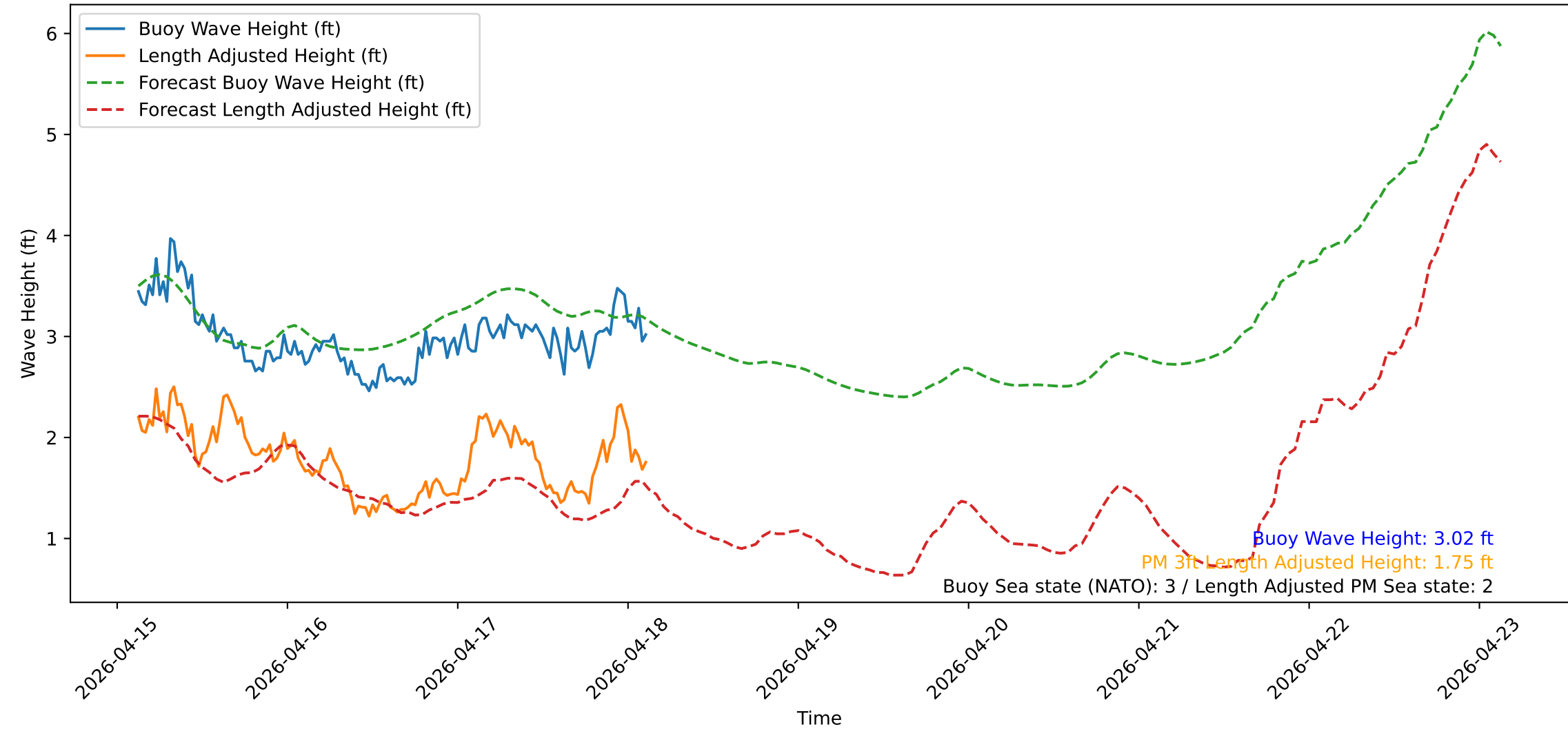
Wave Heights over Time for Green Beach at 2026-04-18 03:11:12
