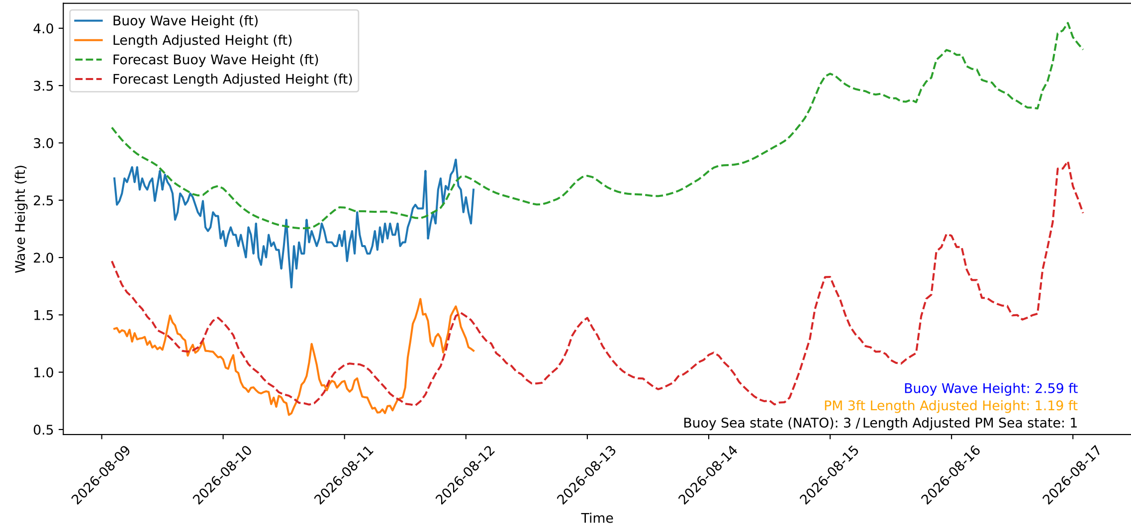
Wave Heights over Time for Red Beach at 2026-08-12 02:10:46
