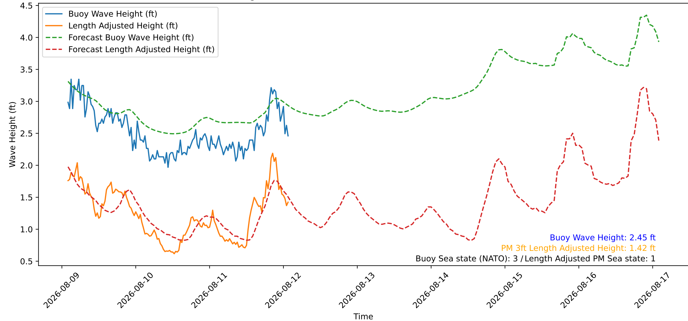
Wave Heights over Time for Green Beach at 2026-08-12 02:11:08
