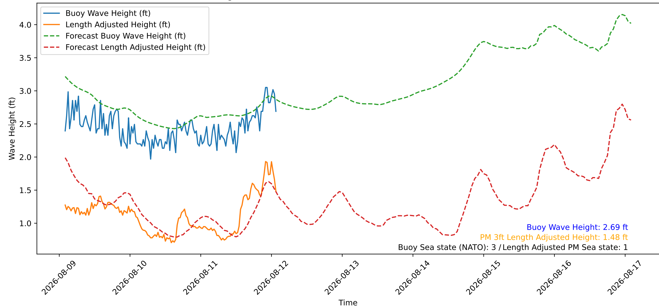
Wave Heights over Time for Oceanside Harbor at 2026-08-12 02:10:26
