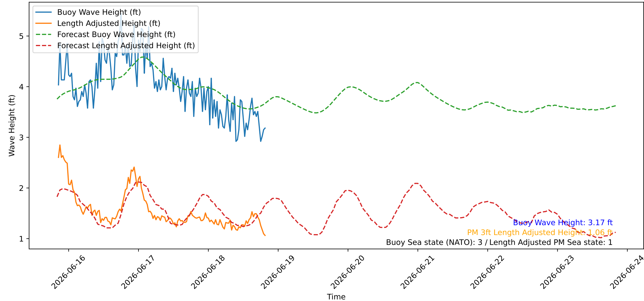
Wave Heights over Time for Oceanside Harbor at 2026-06-18 20:20:25
