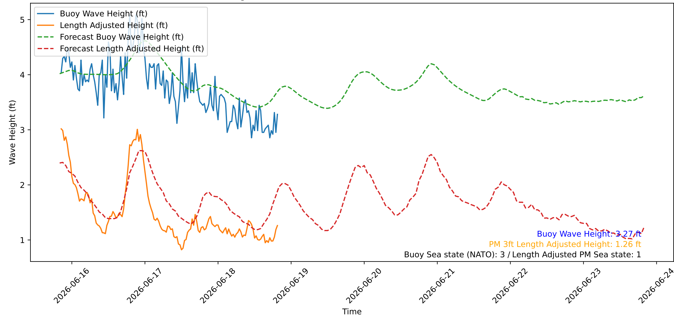
Wave Heights over Time for Green Beach at 2026-06-18 20:21:08
