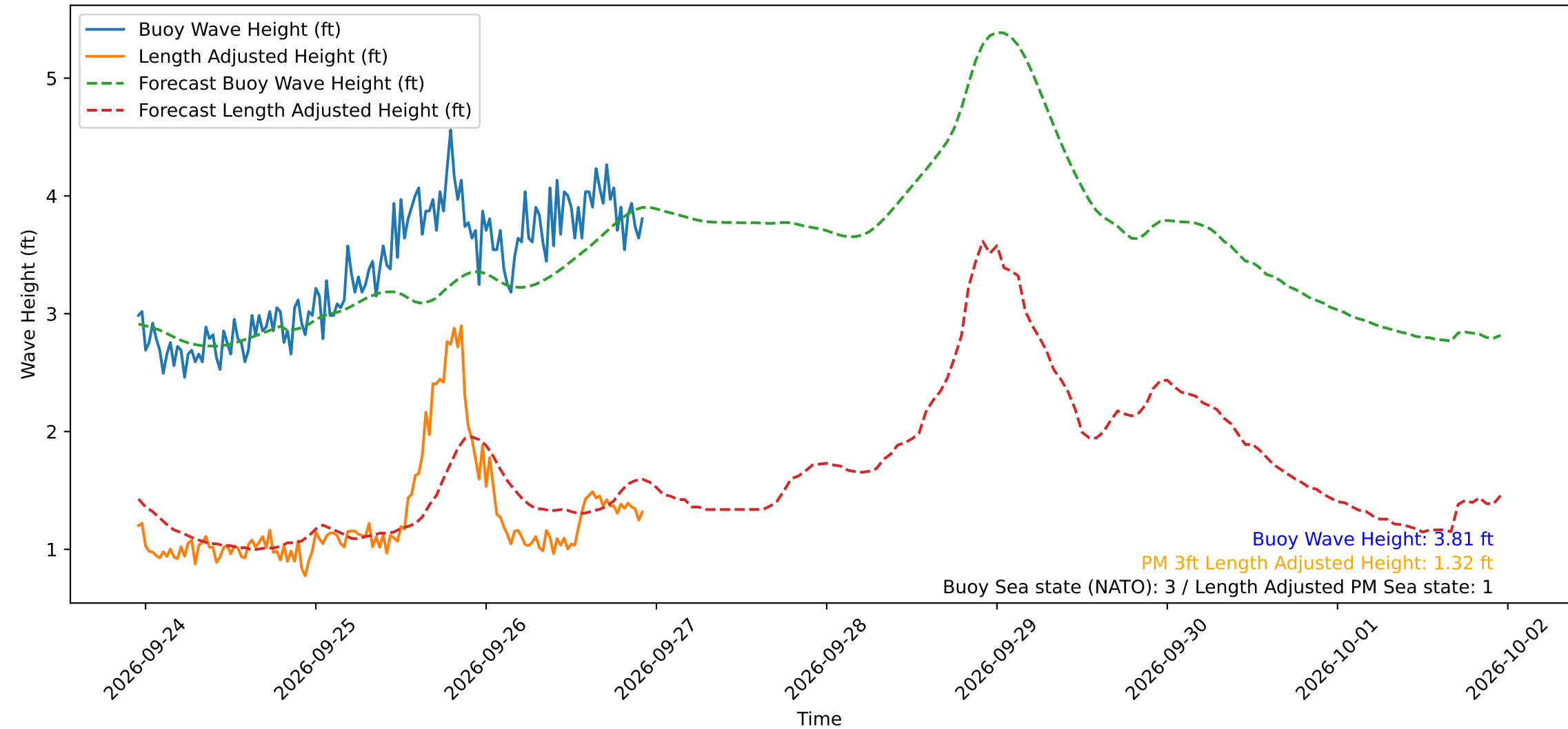
Wave Heights over Time for Green Beach at 2026-09-26 22:51:15
