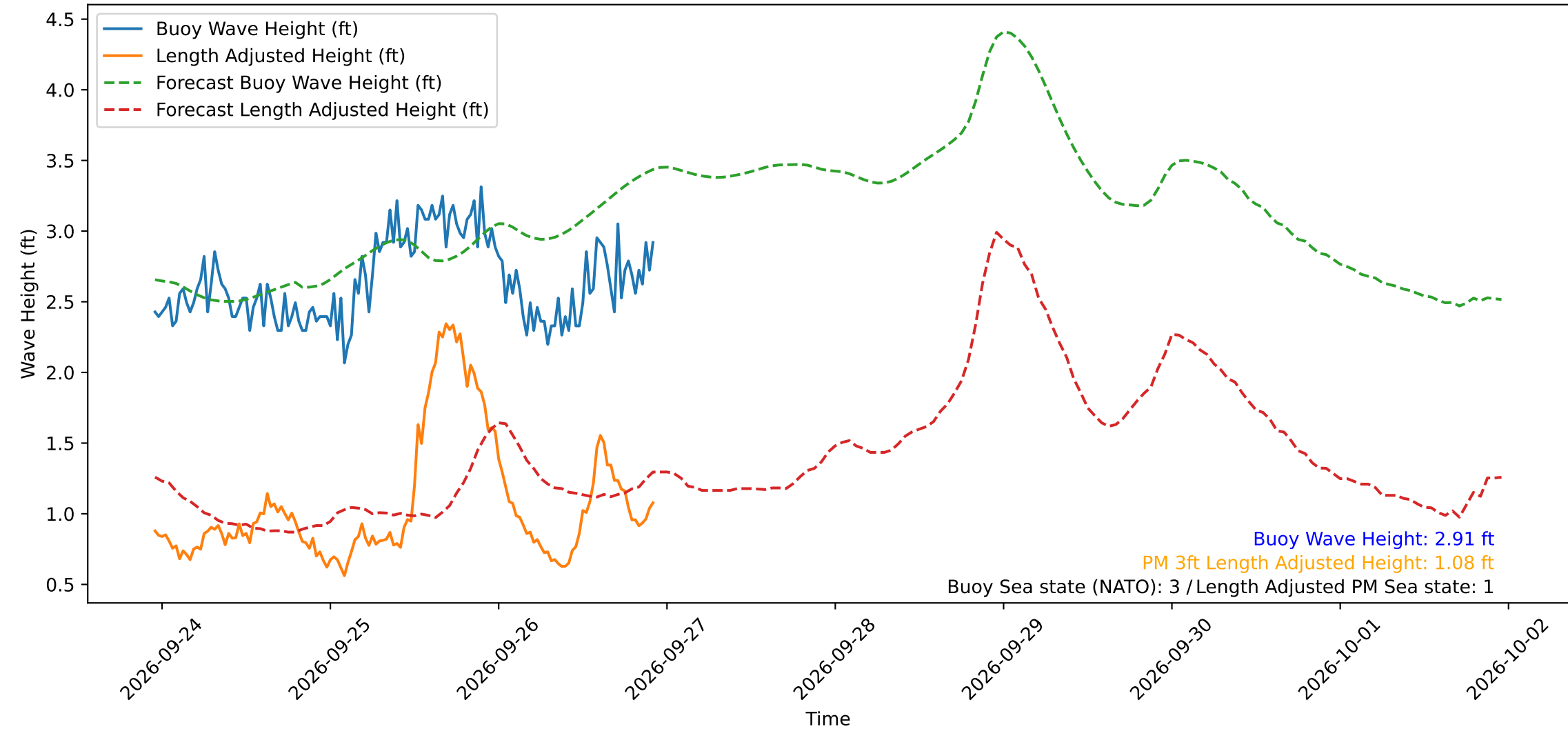
Wave Heights over Time for Red Beach at 2026-09-26 22:50:50
