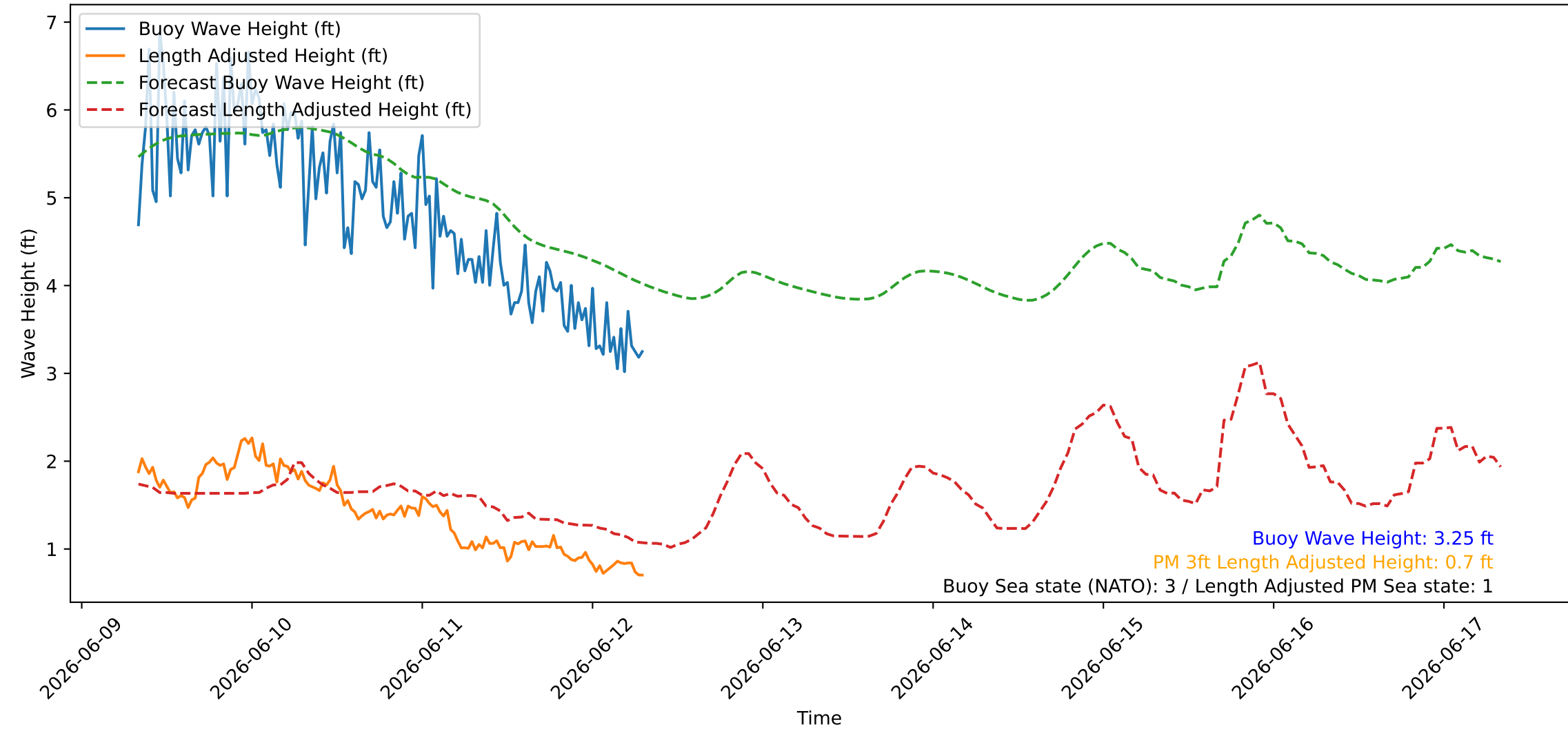
Wave Heights over Time for Green Beach at 2026-06-12 07:51:11
