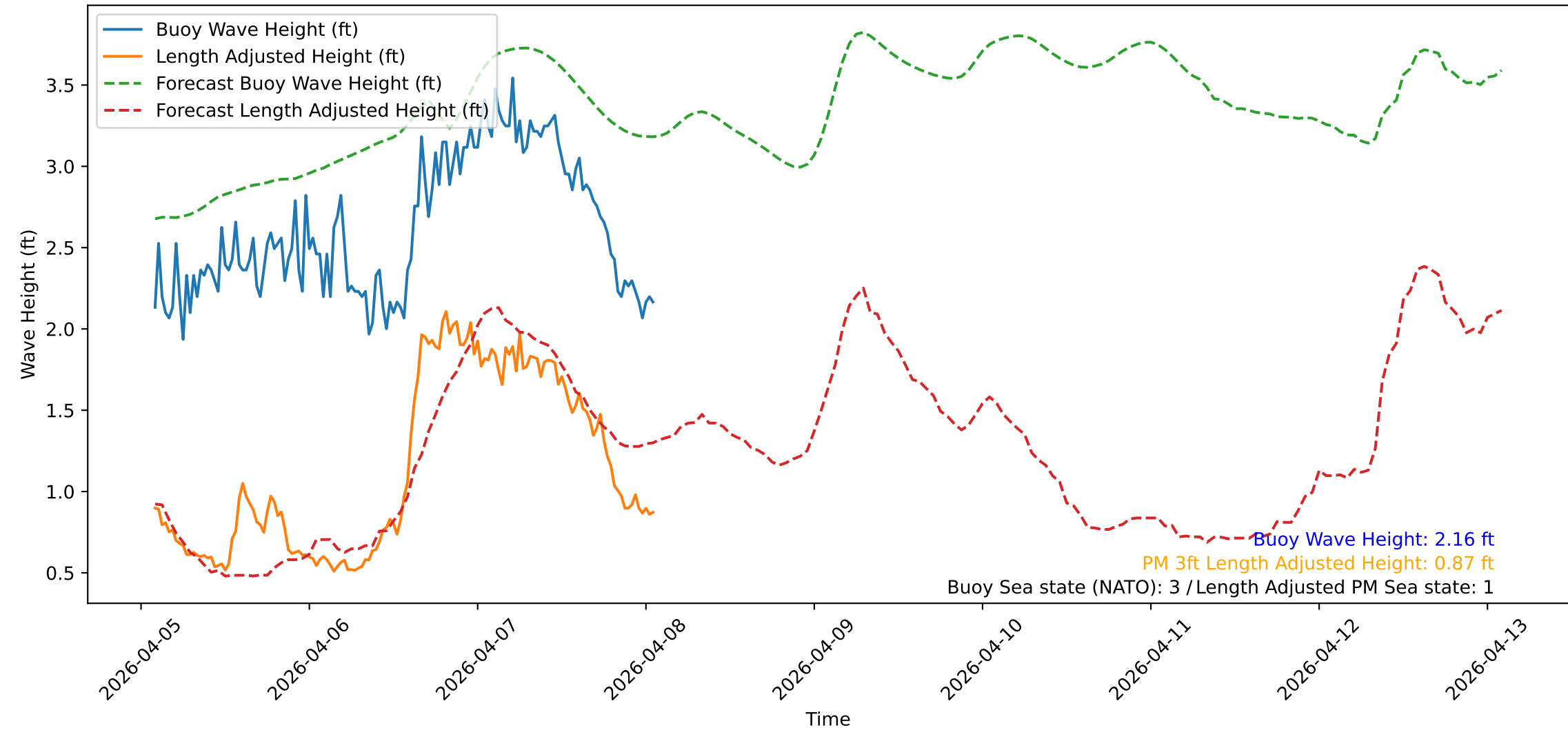
Wave Heights over Time for Red Beach at 2026-04-08 01:40:48
