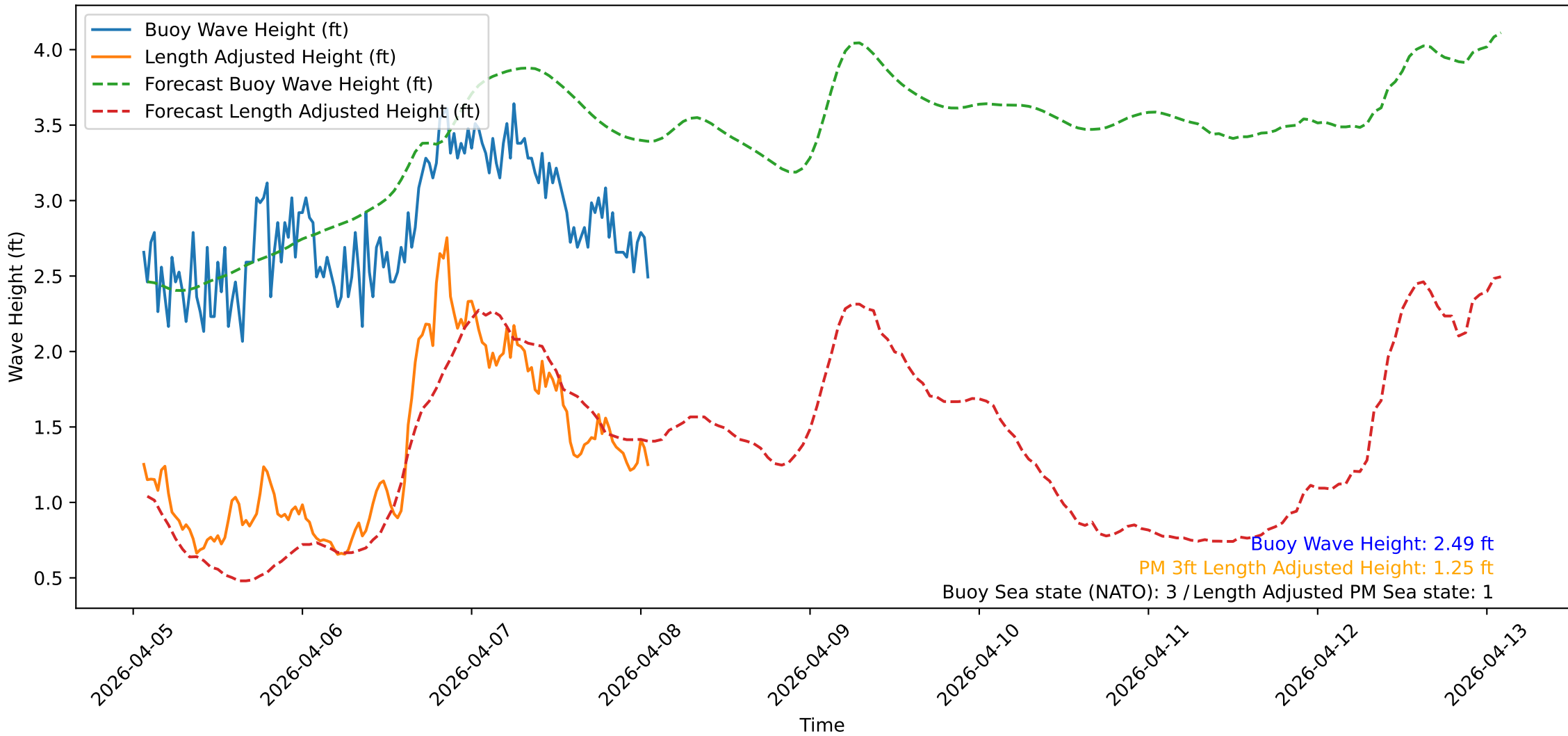
Wave Heights over Time for Oceanside Harbor at 2026-04-08 01:40:32
