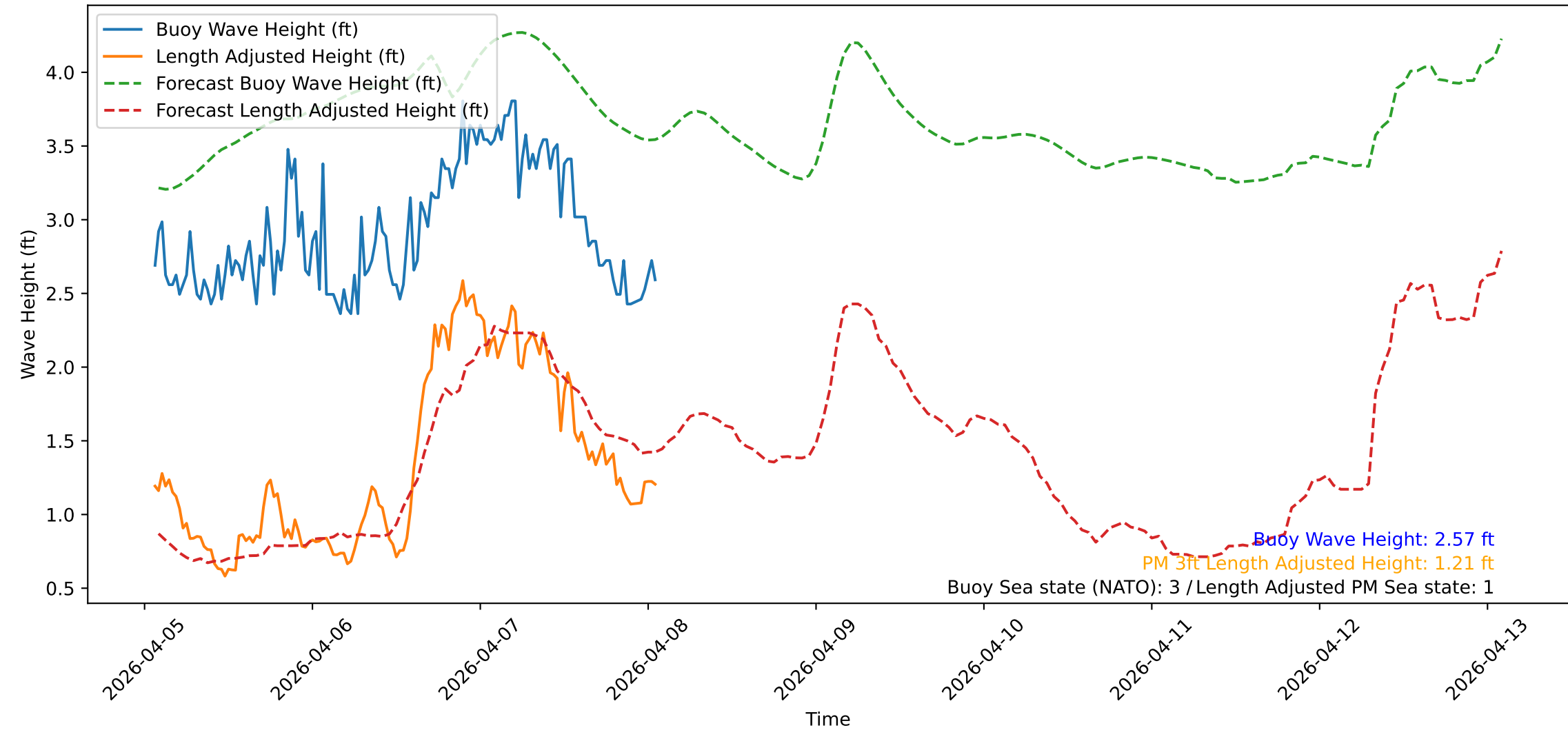
Wave Heights over Time for Green Beach at 2026-04-08 01:41:11
