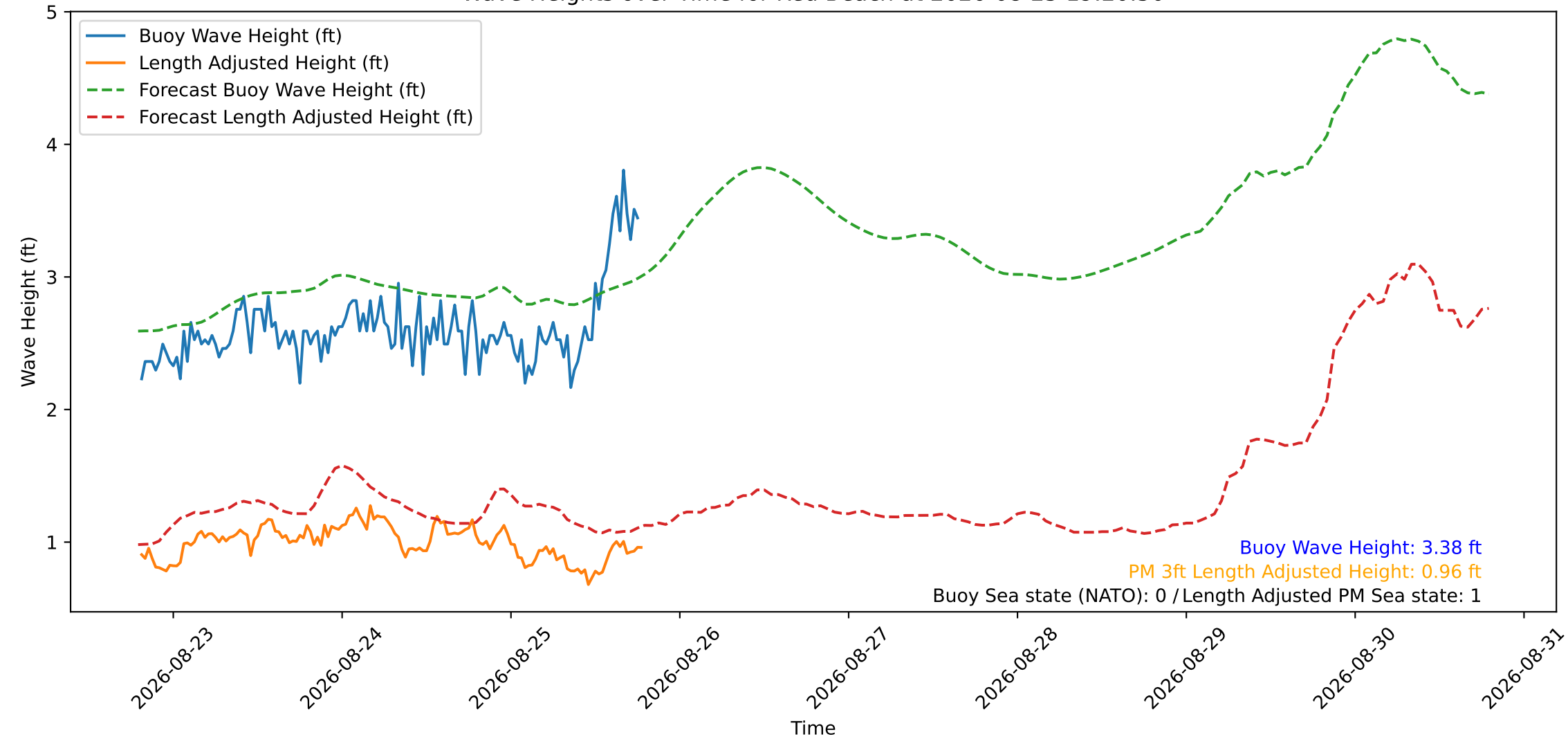
Wave Heights over Time for Red Beach at 2026-08-25 19:20:50
