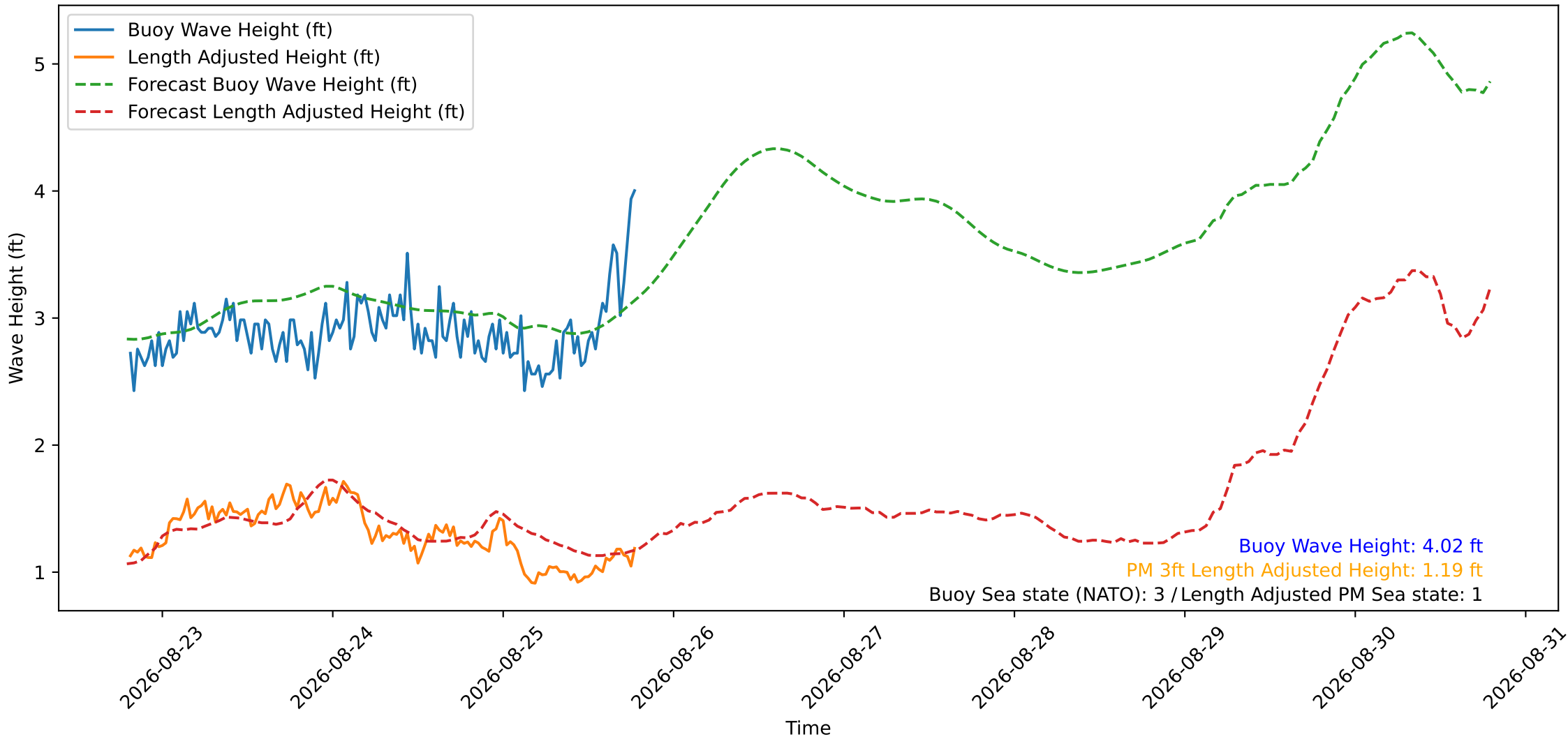
Wave Heights over Time for Oceanside Harbor at 2026-08-25 19:20:29
