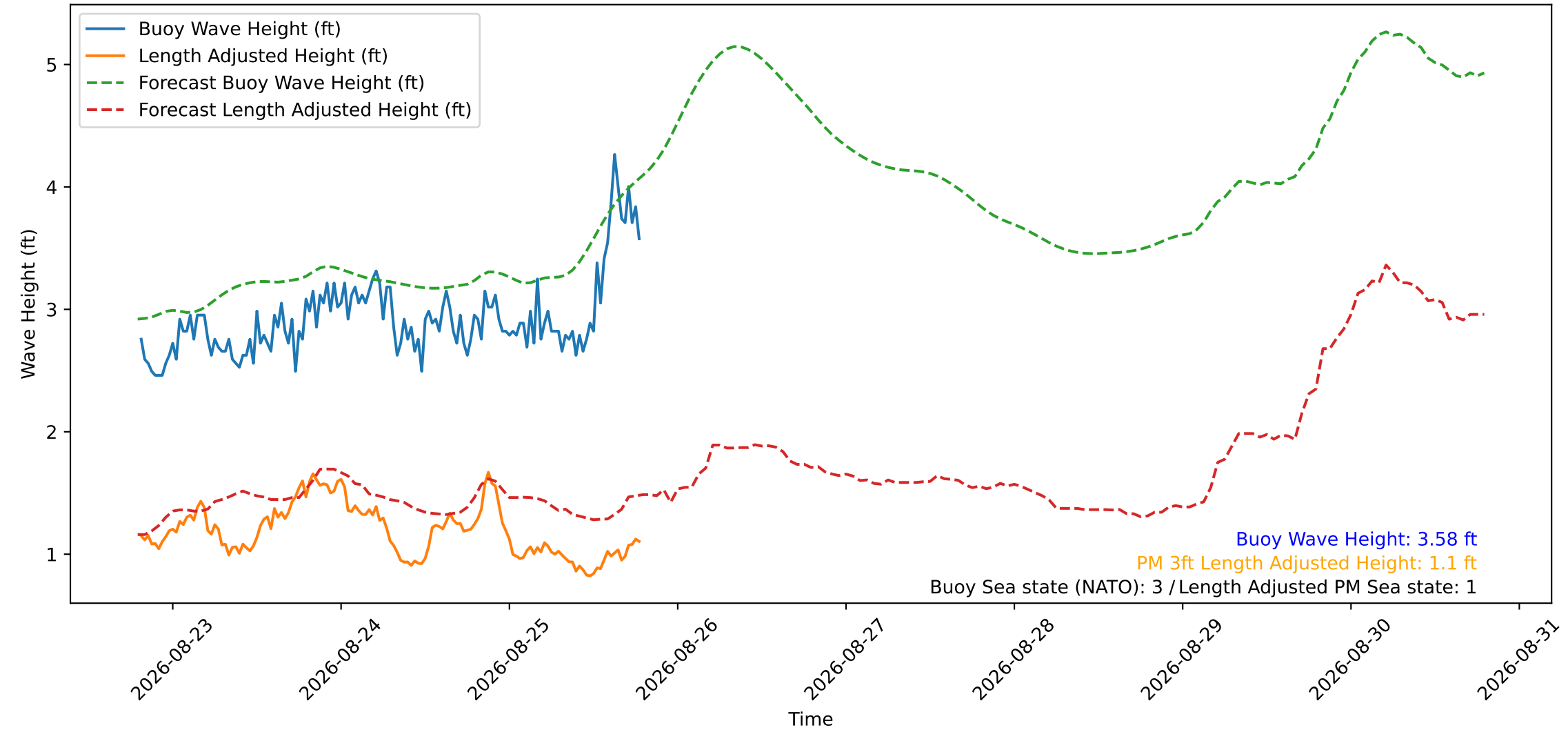
Wave Heights over Time for Green Beach at 2026-08-25 19:21:14
