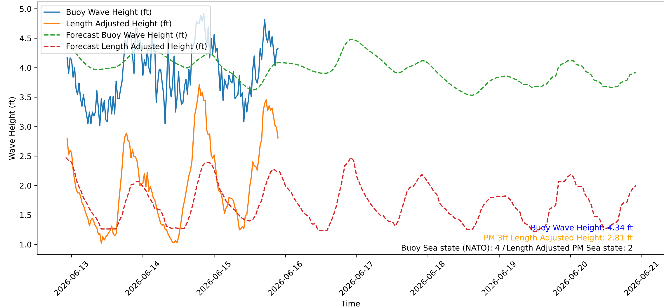
Wave Heights over Time for Green Beach at 2026-06-15 22:21:09
