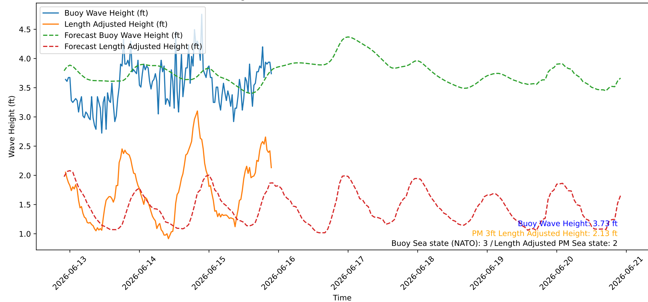
Wave Heights over Time for Red Beach at 2026-06-15 22:20:47
