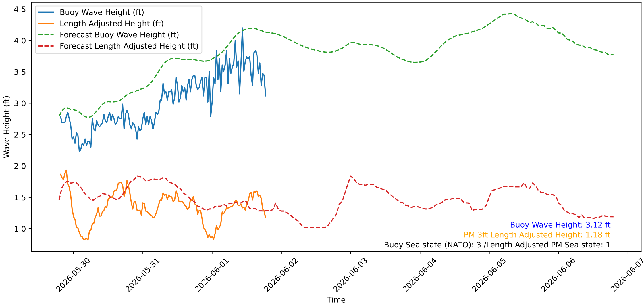
Wave Heights over Time for Red Beach at 2026-06-01 19:20:46
