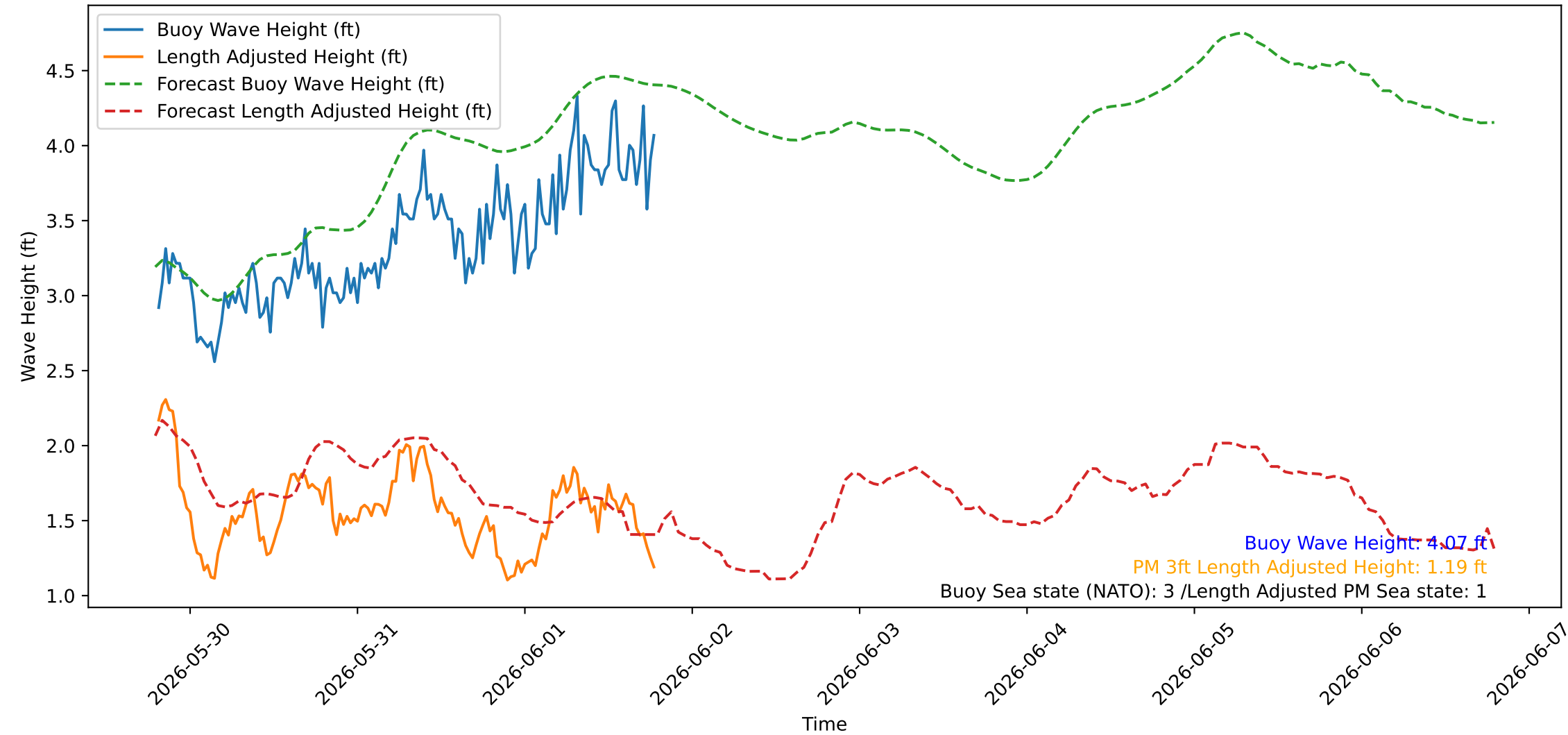
Wave Heights over Time for Green Beach at 2026-06-01 19:21:09
