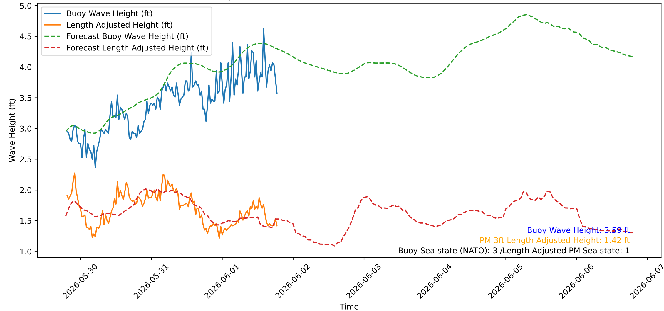
Wave Heights over Time for Oceanside Harbor at 2026-06-01 19:20:25
