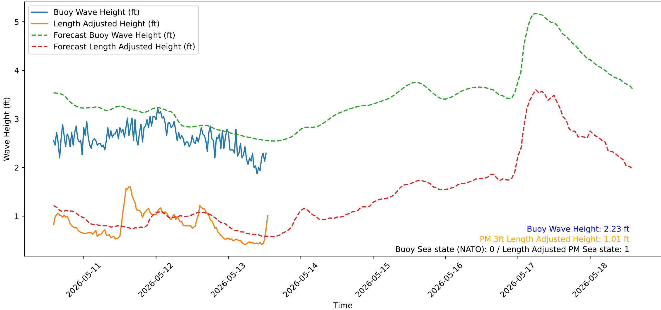
Wave Heights over Time for Red Beach at 2026-05-13 13:40:50
