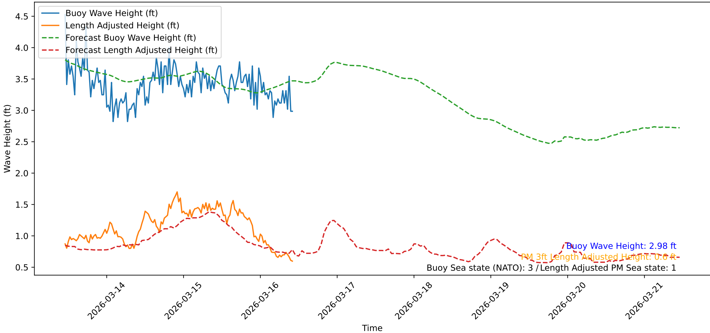
Wave Heights over Time for Green Beach at 2026-03-16 10:51:40
