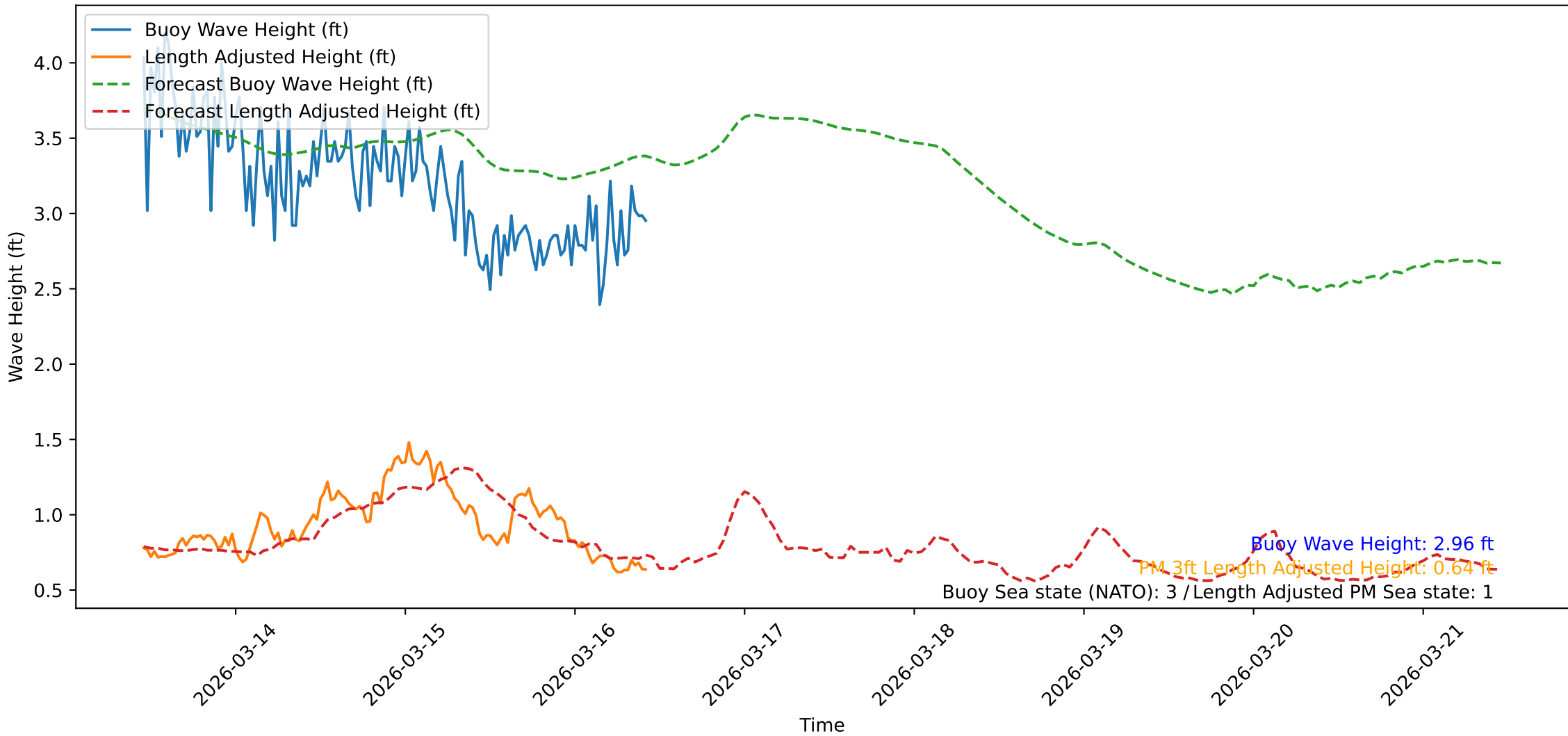
Wave Heights over Time for Oceanside Harbor at 2026-03-16 10:50:42
