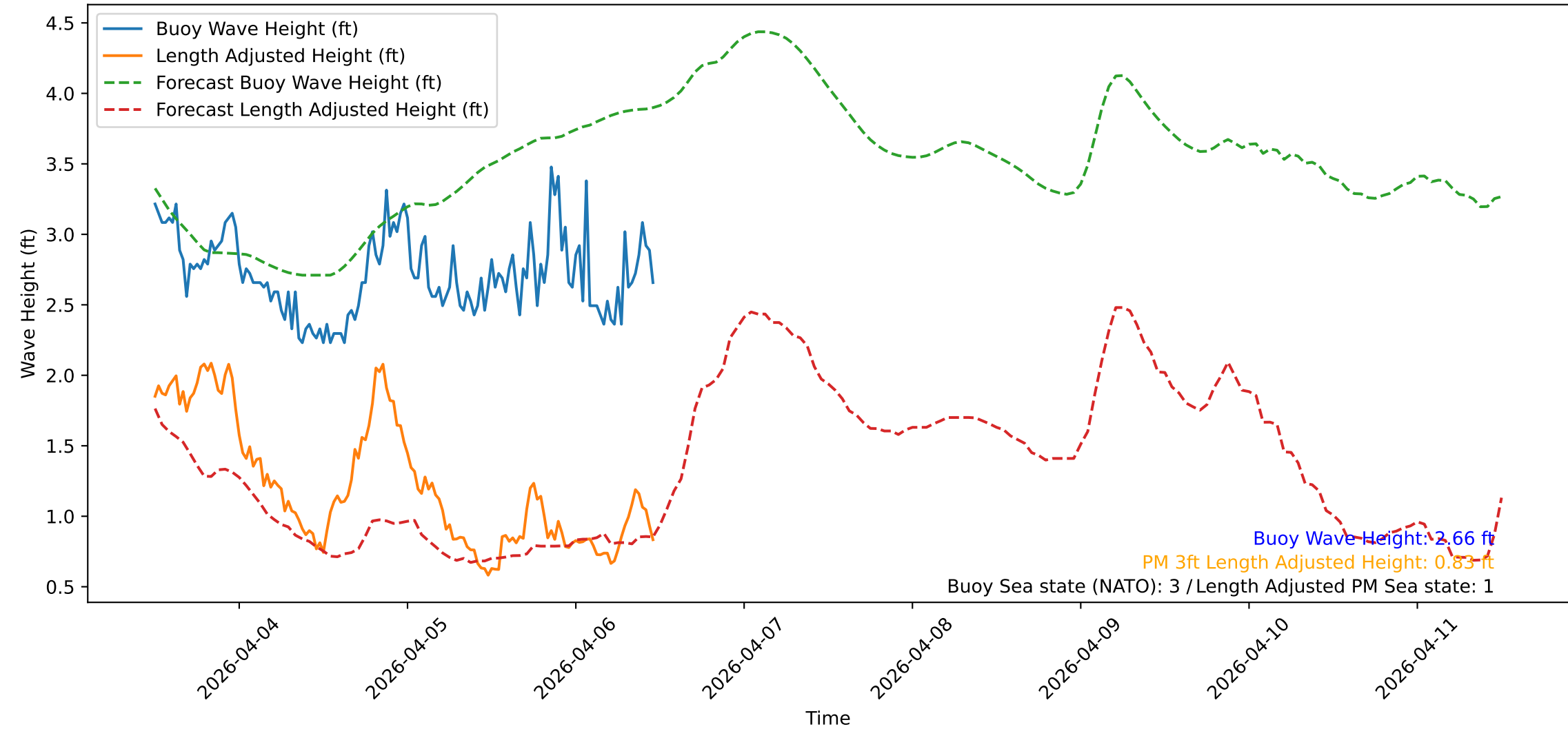
Wave Heights over Time for Green Beach at 2026-04-06 12:01:11
