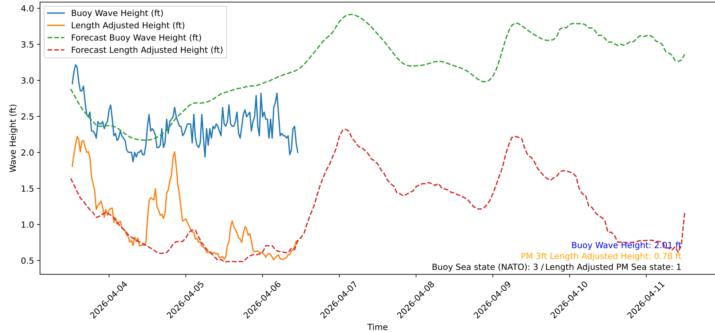
Wave Heights over Time for Red Beach at 2026-04-06 12:00:48
