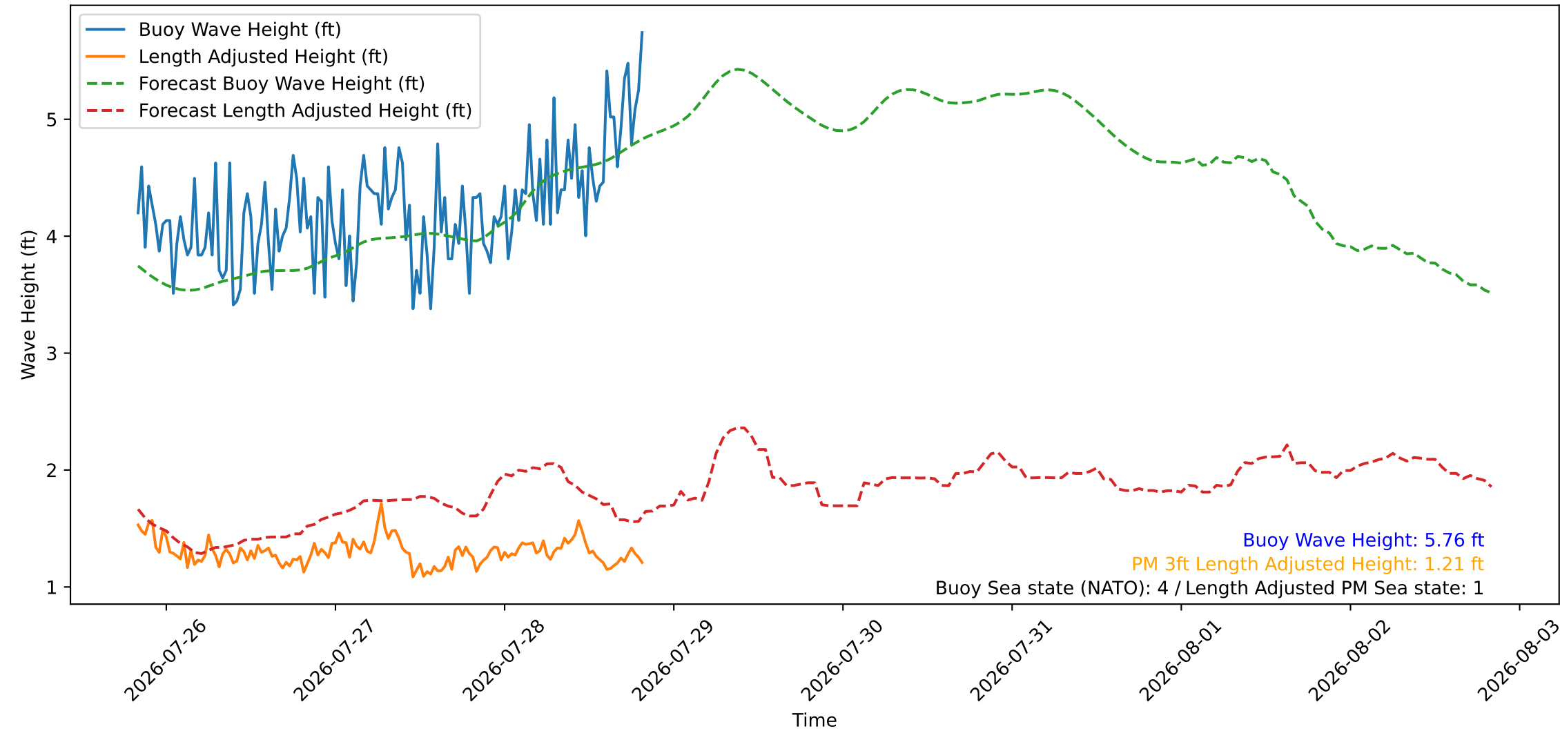
Wave Heights over Time for Green Beach at 2026-07-28 20:11:08
