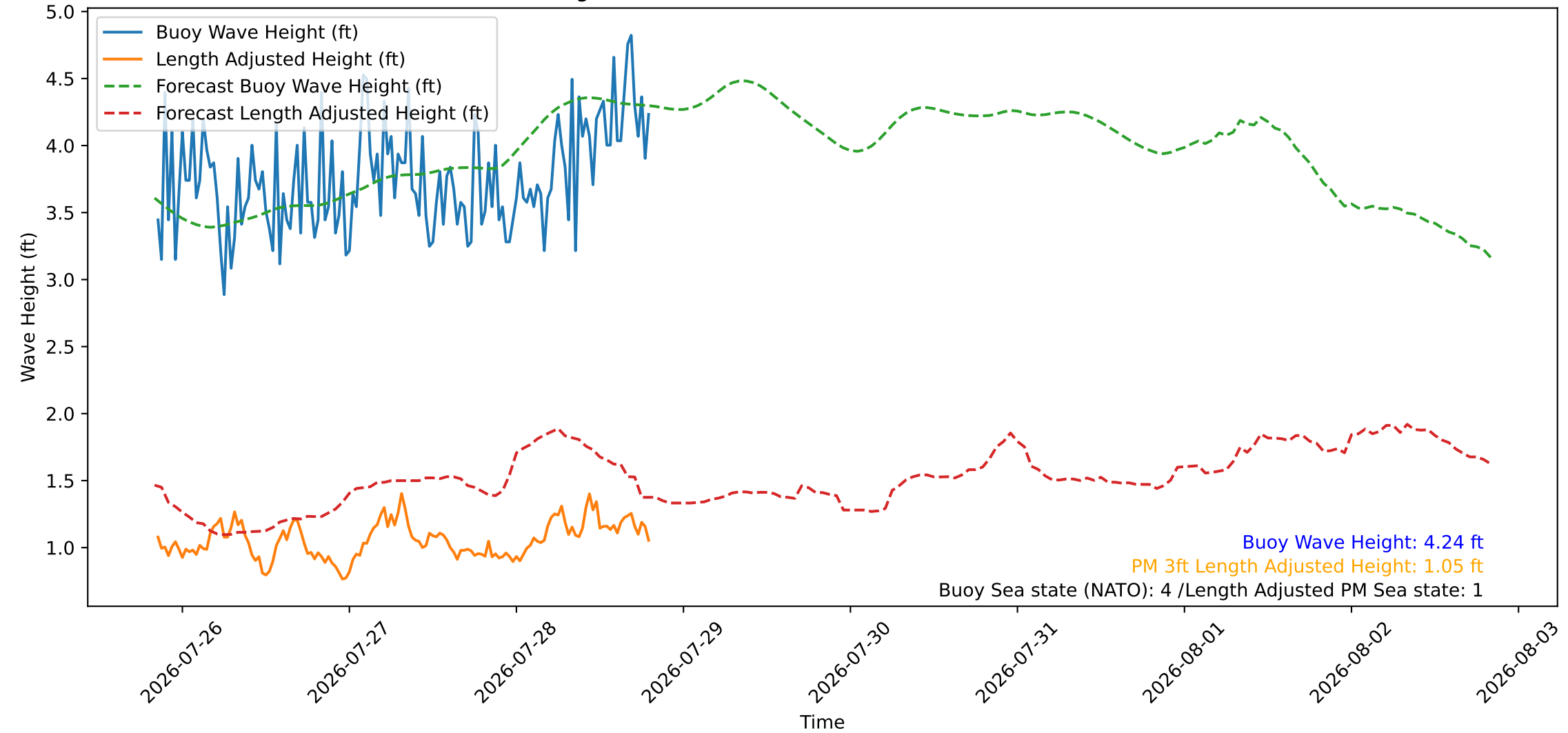
Wave Heights over Time for Red Beach at 2026-07-28 20:10:45
