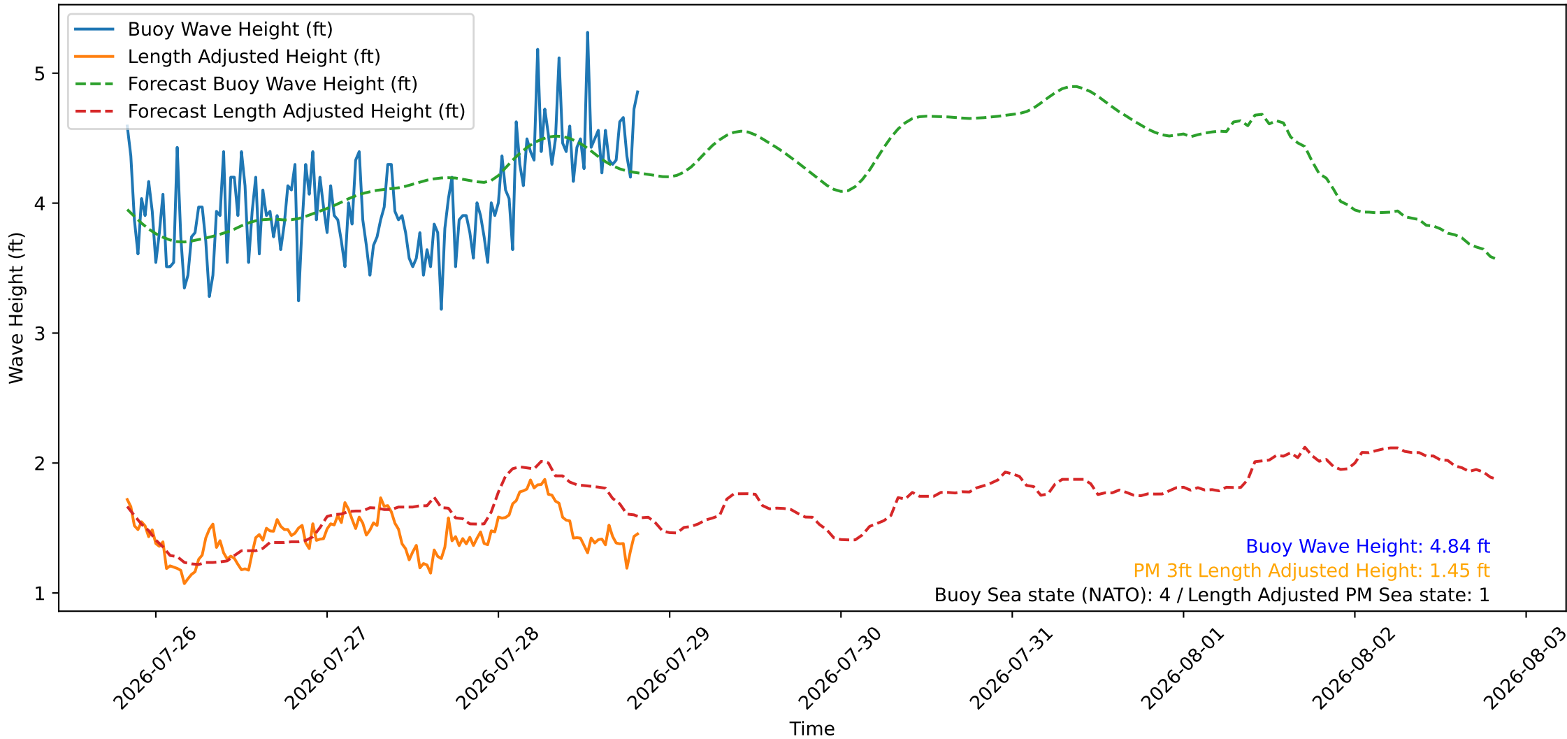
Wave Heights over Time for Oceanside Harbor at 2026-07-28 20:10:26
