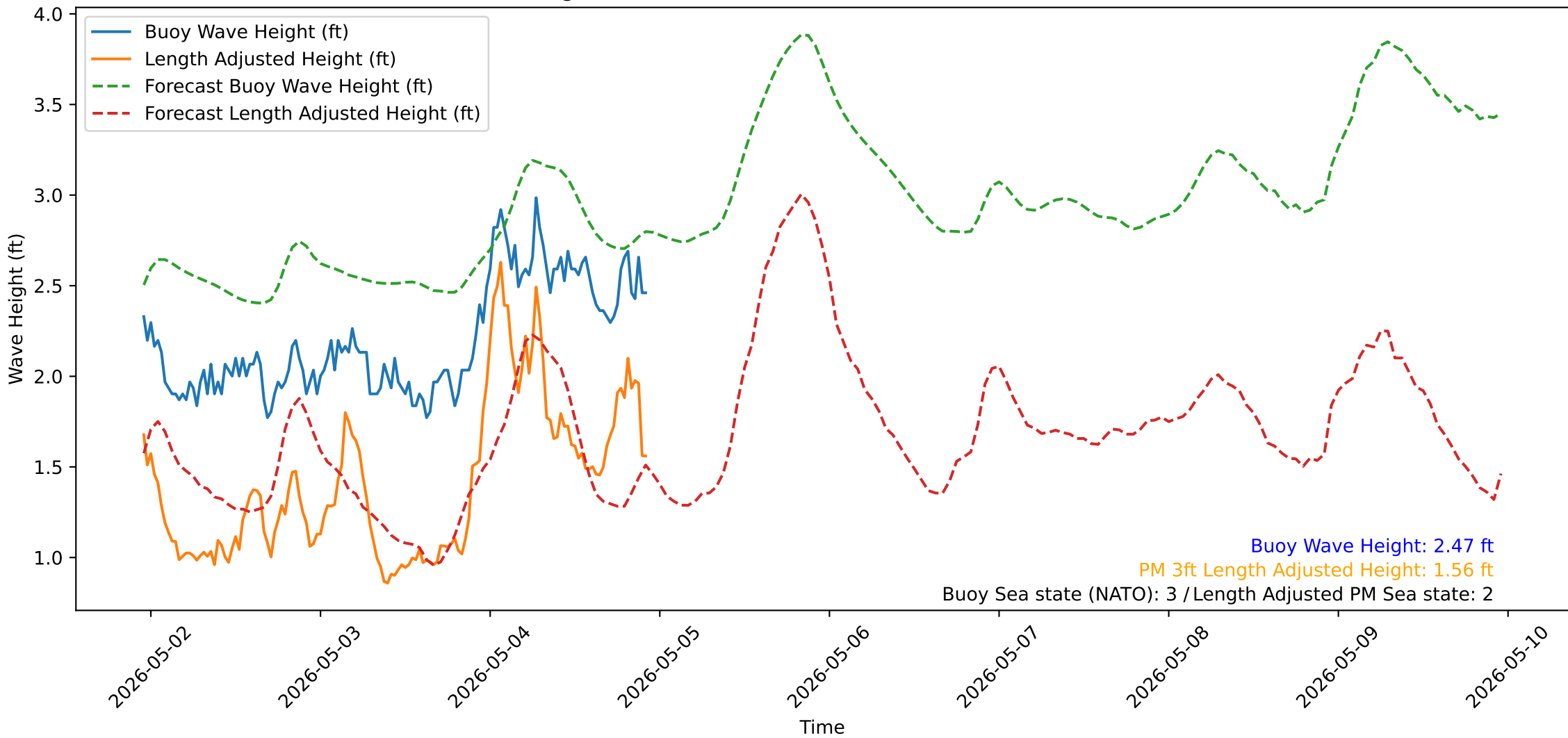
Wave Heights over Time for Green Beach at 2026-05-04 22:51:14
