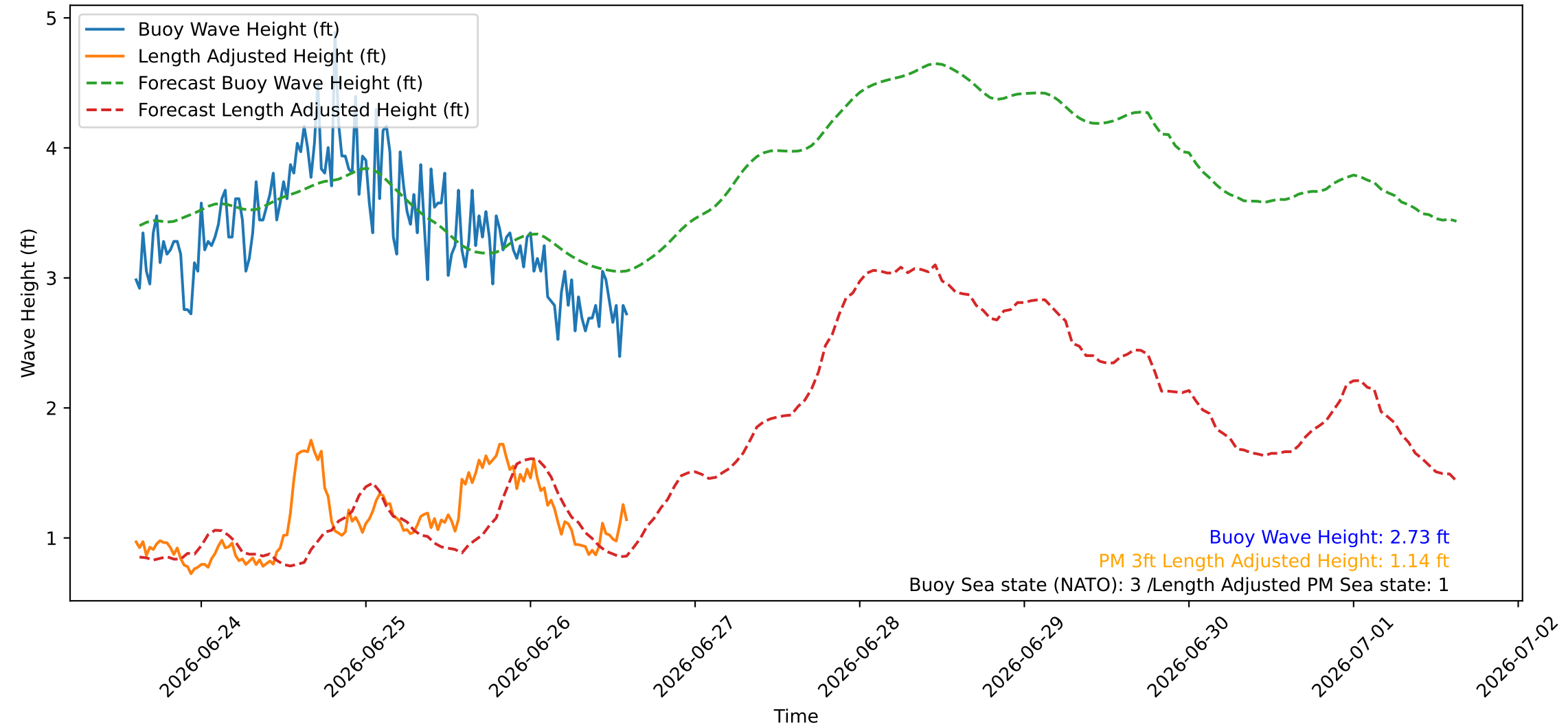
Wave Heights over Time for Oceanside Harbor at 2026-06-26 14:40:26
