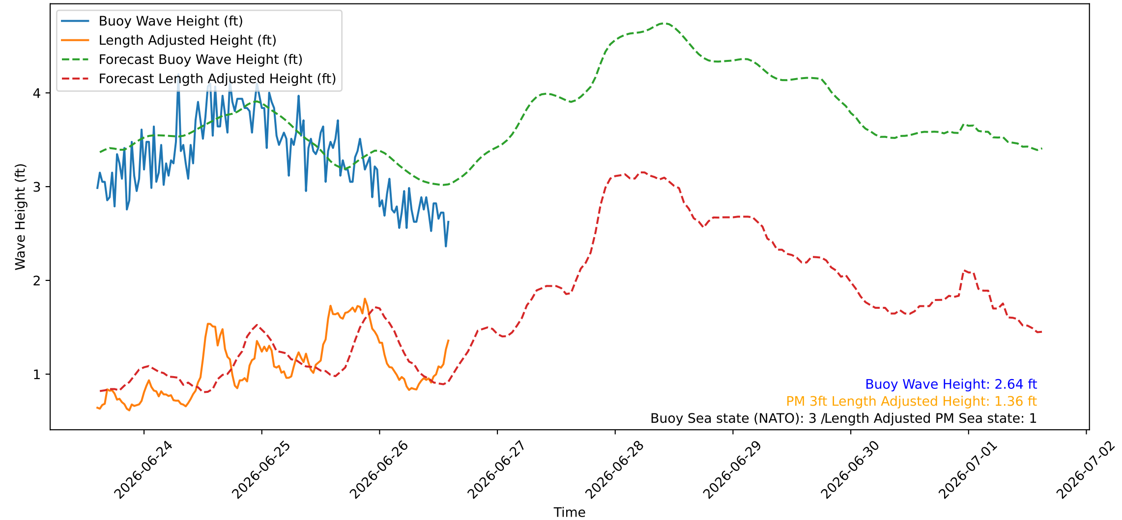
Wave Heights over Time for Green Beach at 2026-06-26 14:41:08
