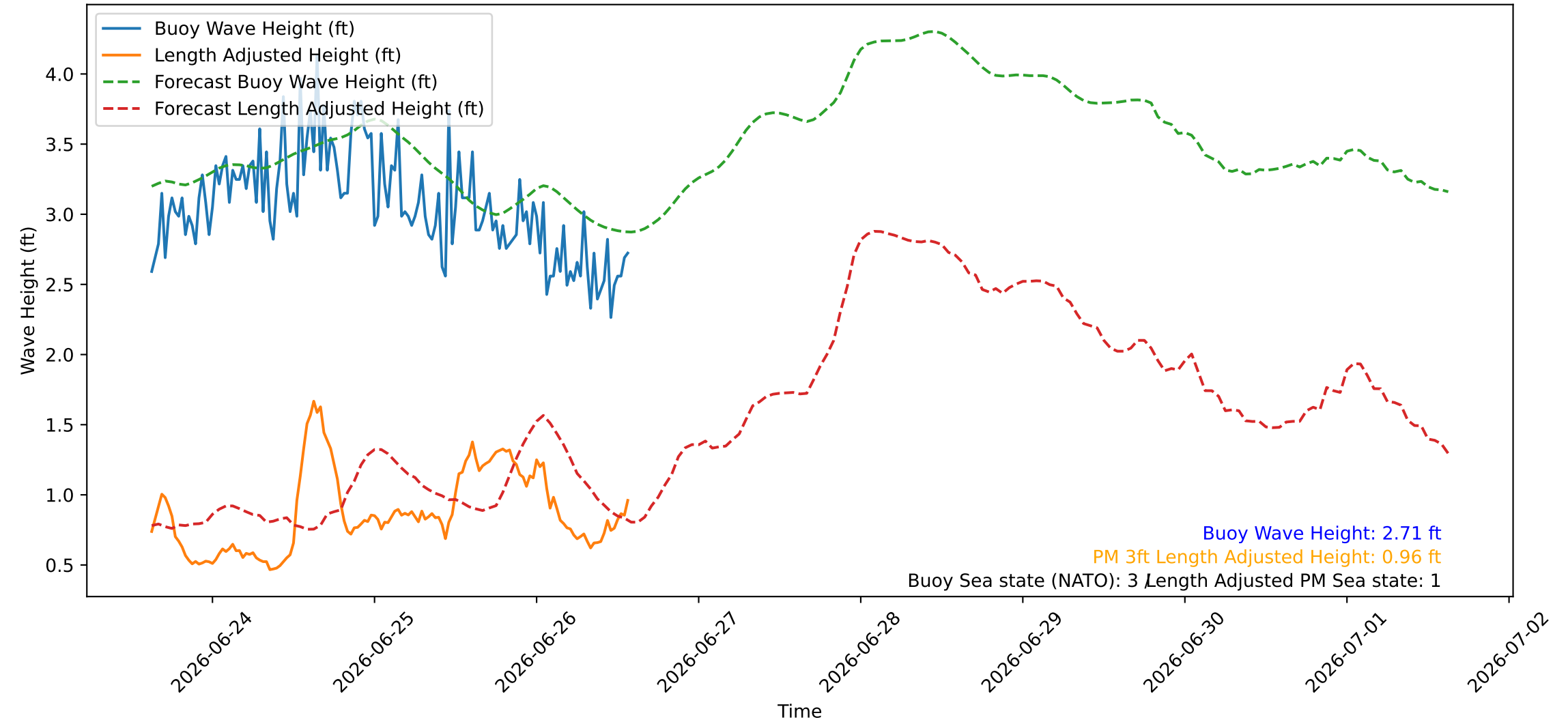
Wave Heights over Time for Red Beach at 2026-06-26 14:40:45
