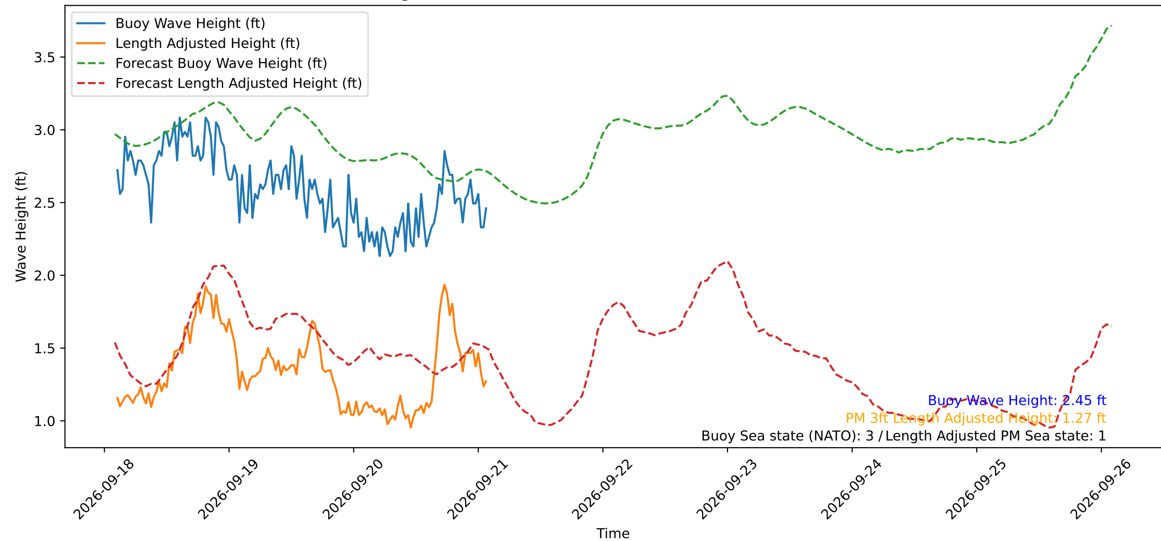
Wave Heights over Time for Oceanside Harbor at 2026-09-21 02:20:29
