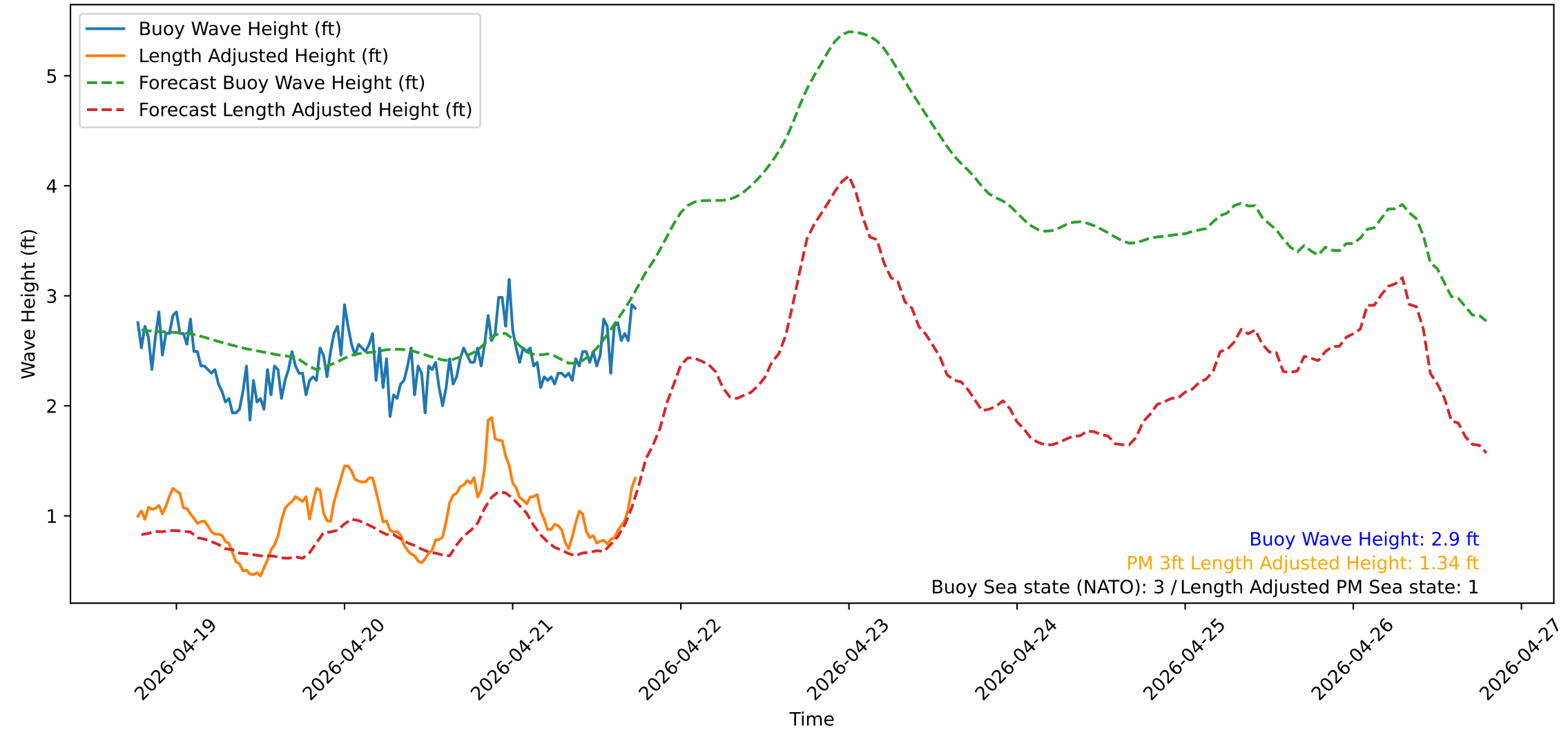
Wave Heights over Time for Green Beach at 2026-04-21 18:31:14
