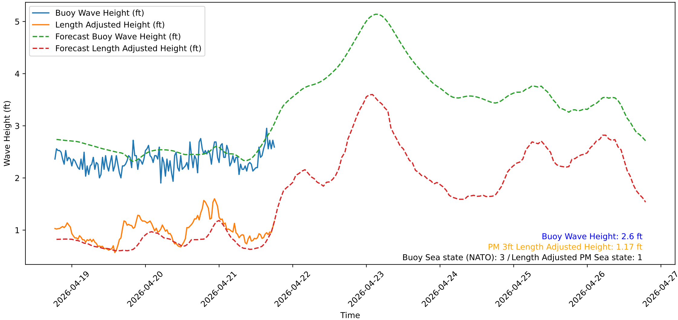
Wave Heights over Time for Oceanside Harbor at 2026-04-21 18:30:32
