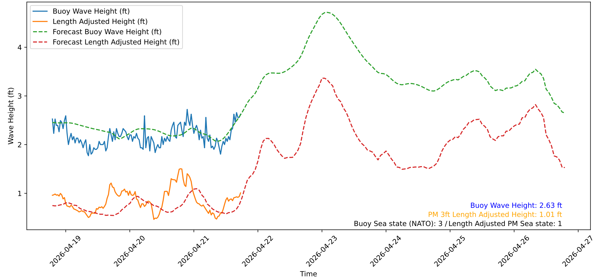
Wave Heights over Time for Red Beach at 2026-04-21 18:30:51
