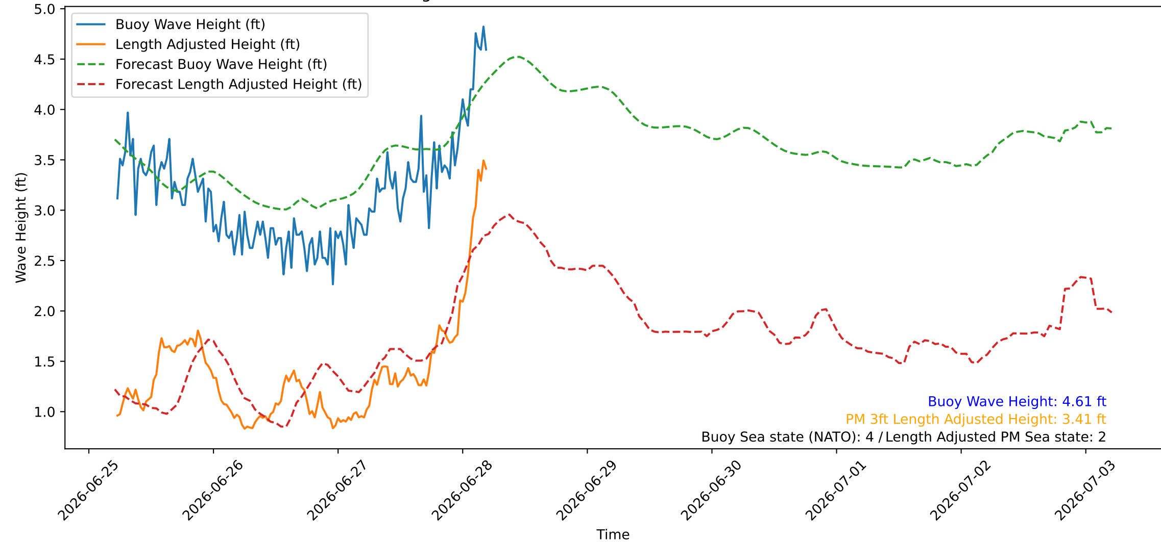
Wave Heights over Time for Green Beach at 2026-06-28 05:21:09
