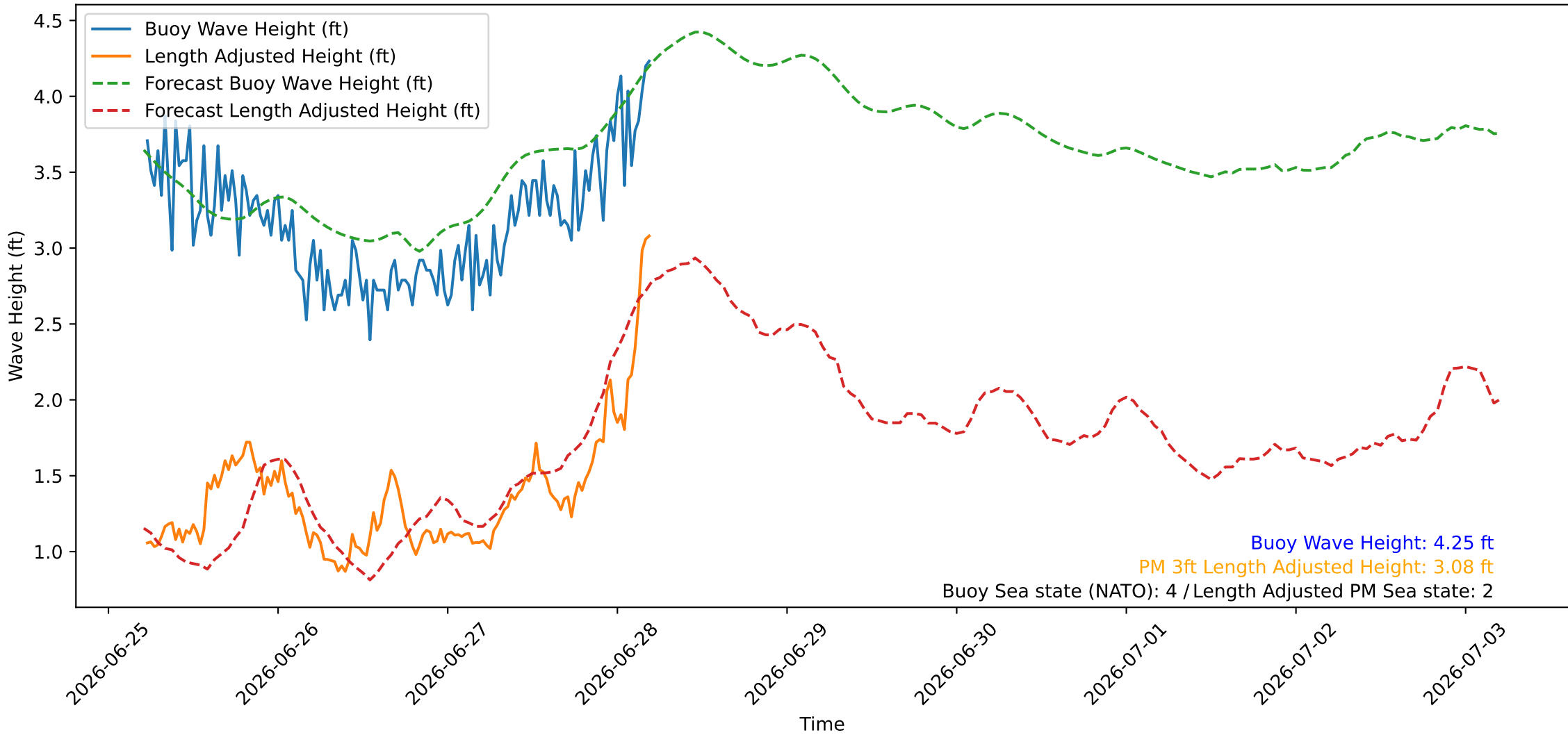
Wave Heights over Time for Oceanside Harbor at 2026-06-28 05:20:26
