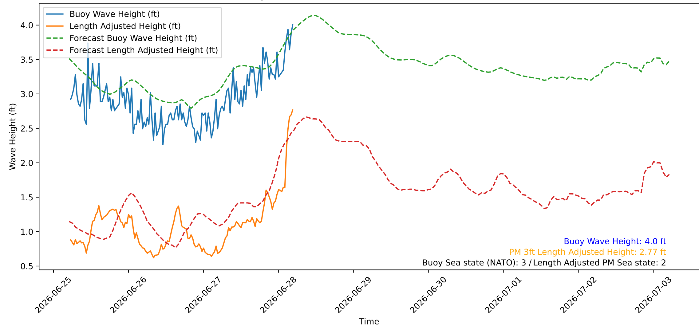
Wave Heights over Time for Red Beach at 2026-06-28 05:20:46
