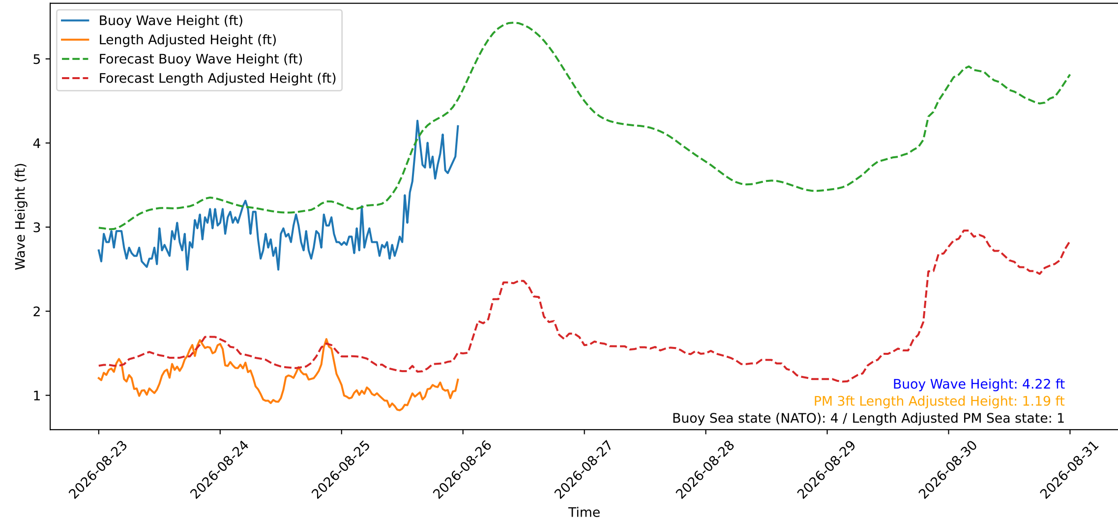
Wave Heights over Time for Green Beach at 2026-08-25 23:51:14
