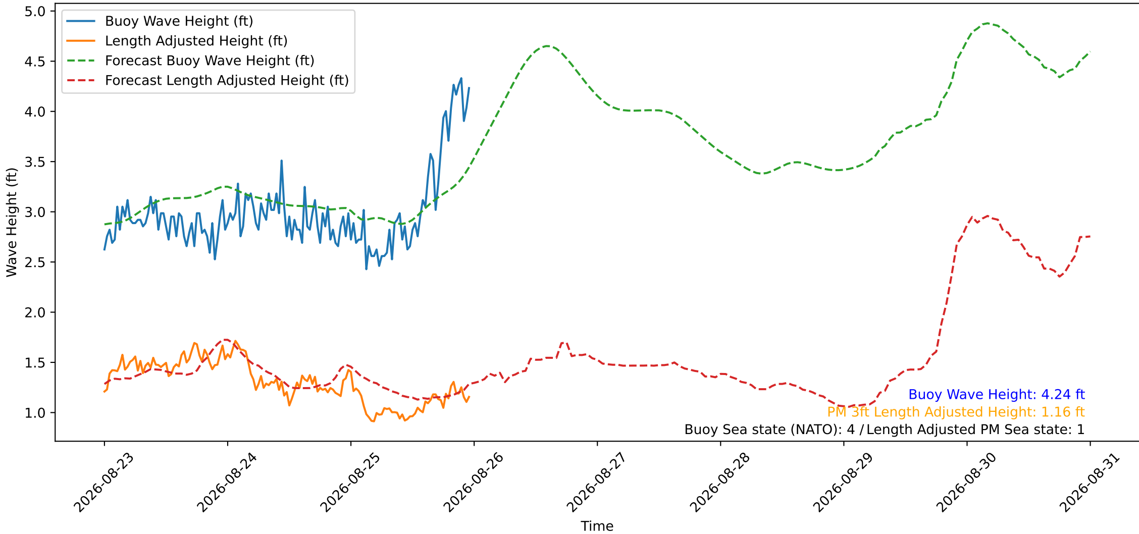
Wave Heights over Time for Oceanside Harbor at 2026-08-25 23:50:29
