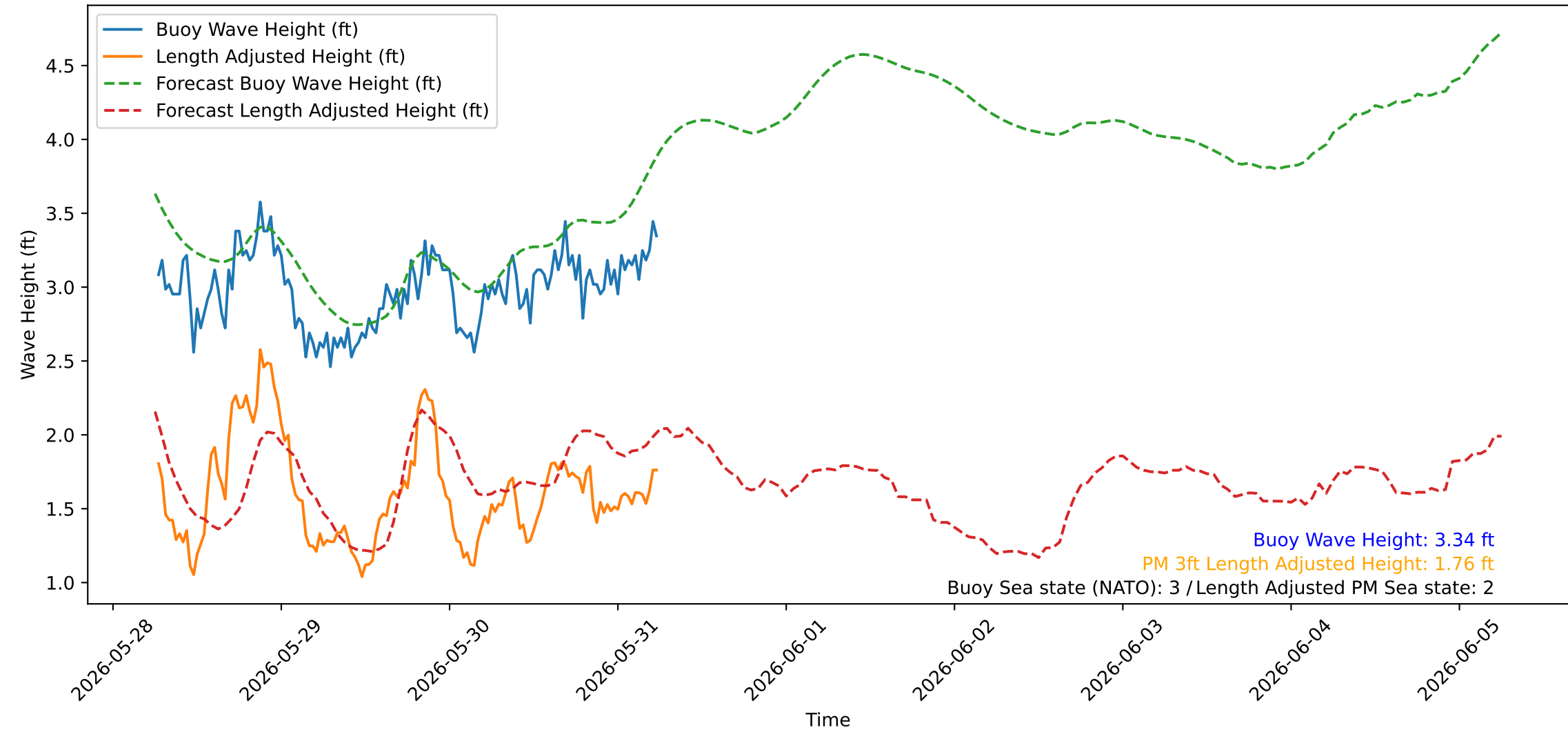
Wave Heights over Time for Green Beach at 2026-05-31 06:21:08
