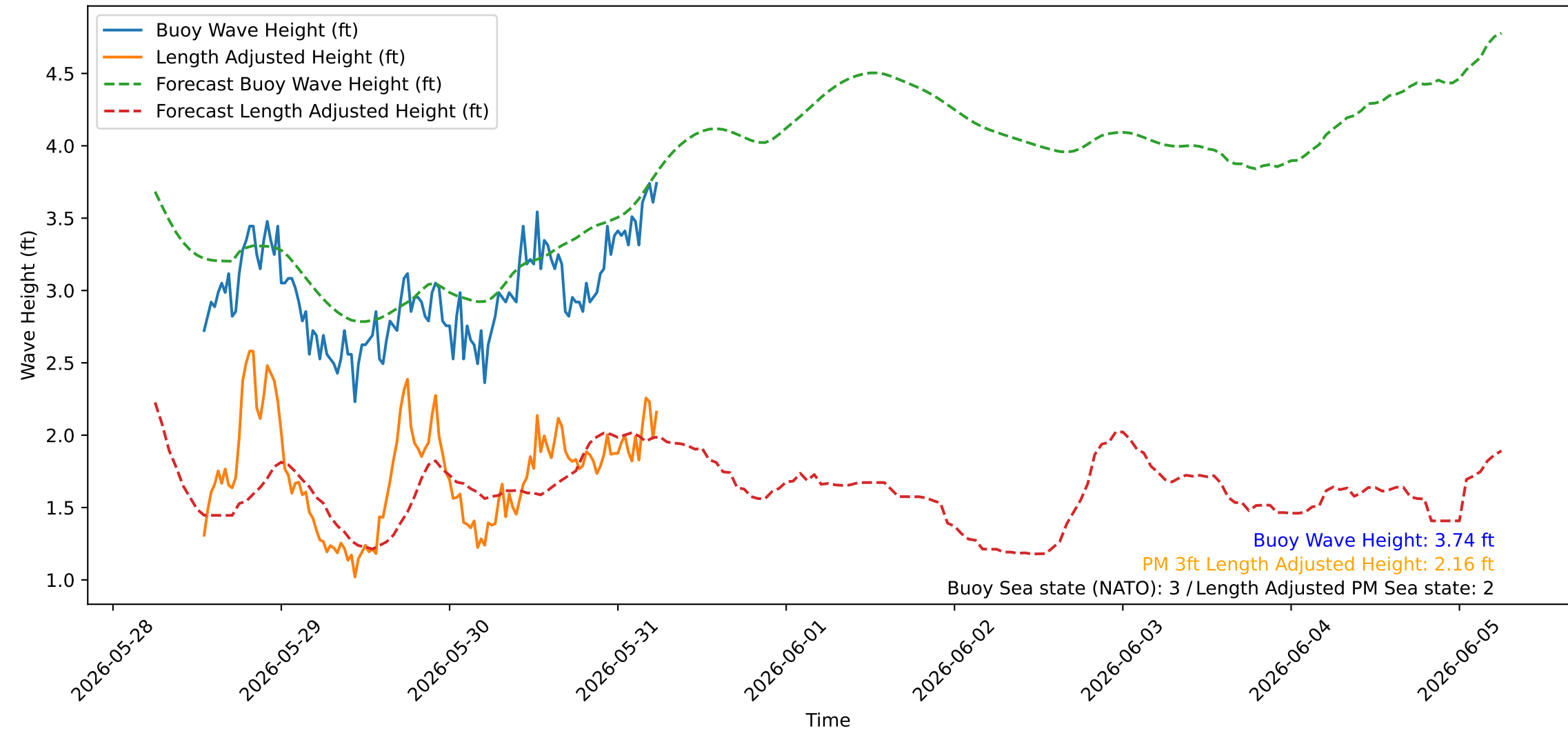
Wave Heights over Time for Oceanside Harbor at 2026-05-31 06:20:25
