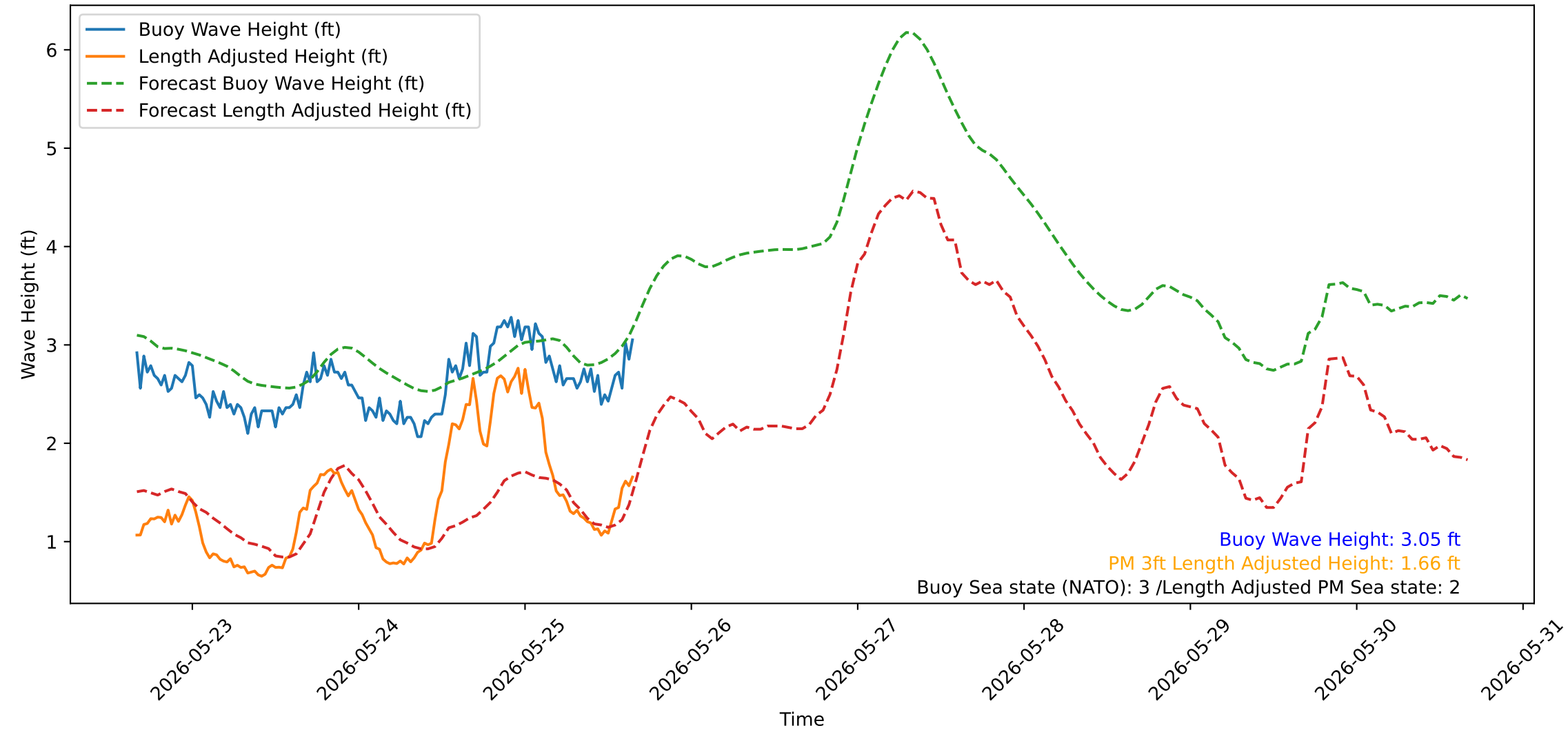
Wave Heights over Time for Green Beach at 2026-05-25 16:11:11
