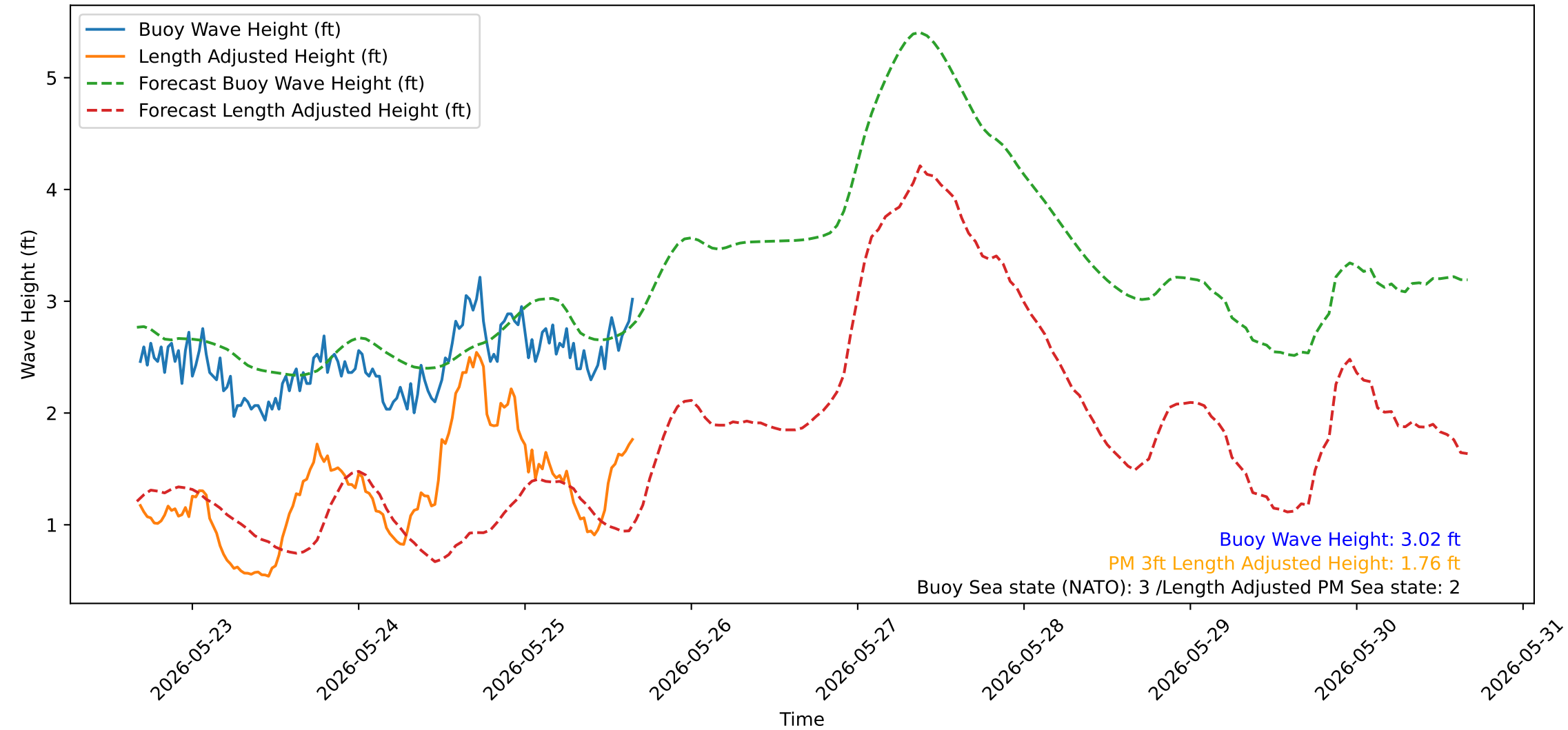
Wave Heights over Time for Red Beach at 2026-05-25 16:10:49
