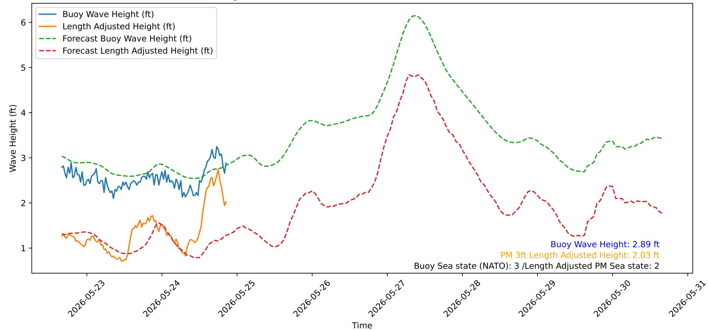
Wave Heights over Time for Oceanside Harbor at 2026-05-25 16:10:29
