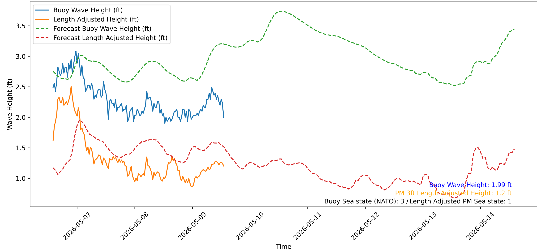
Wave Heights over Time for Red Beach at 2026-05-09 13:50:52
