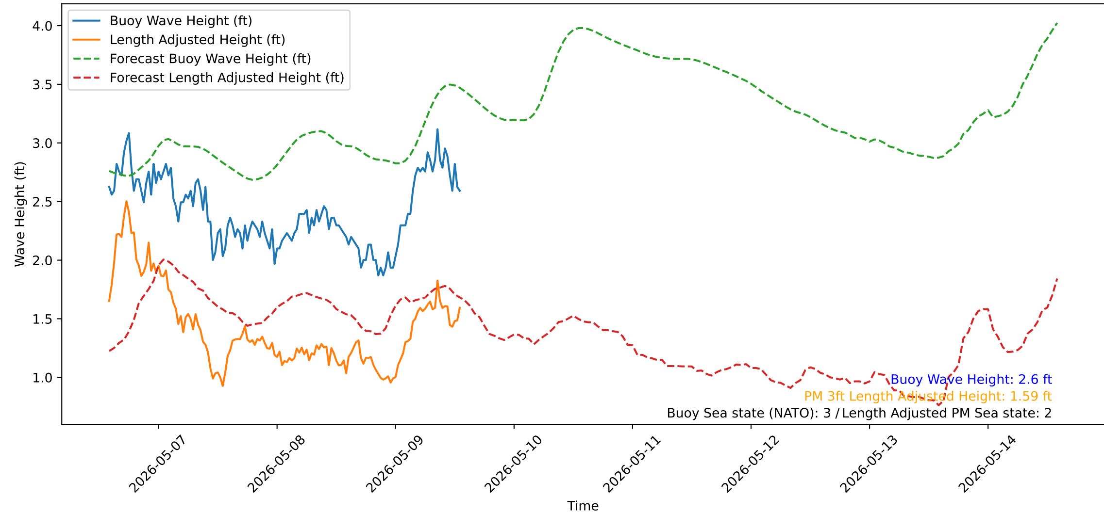
Wave Heights over Time for Oceanside Harbor at 2026-05-09 13:50:32
