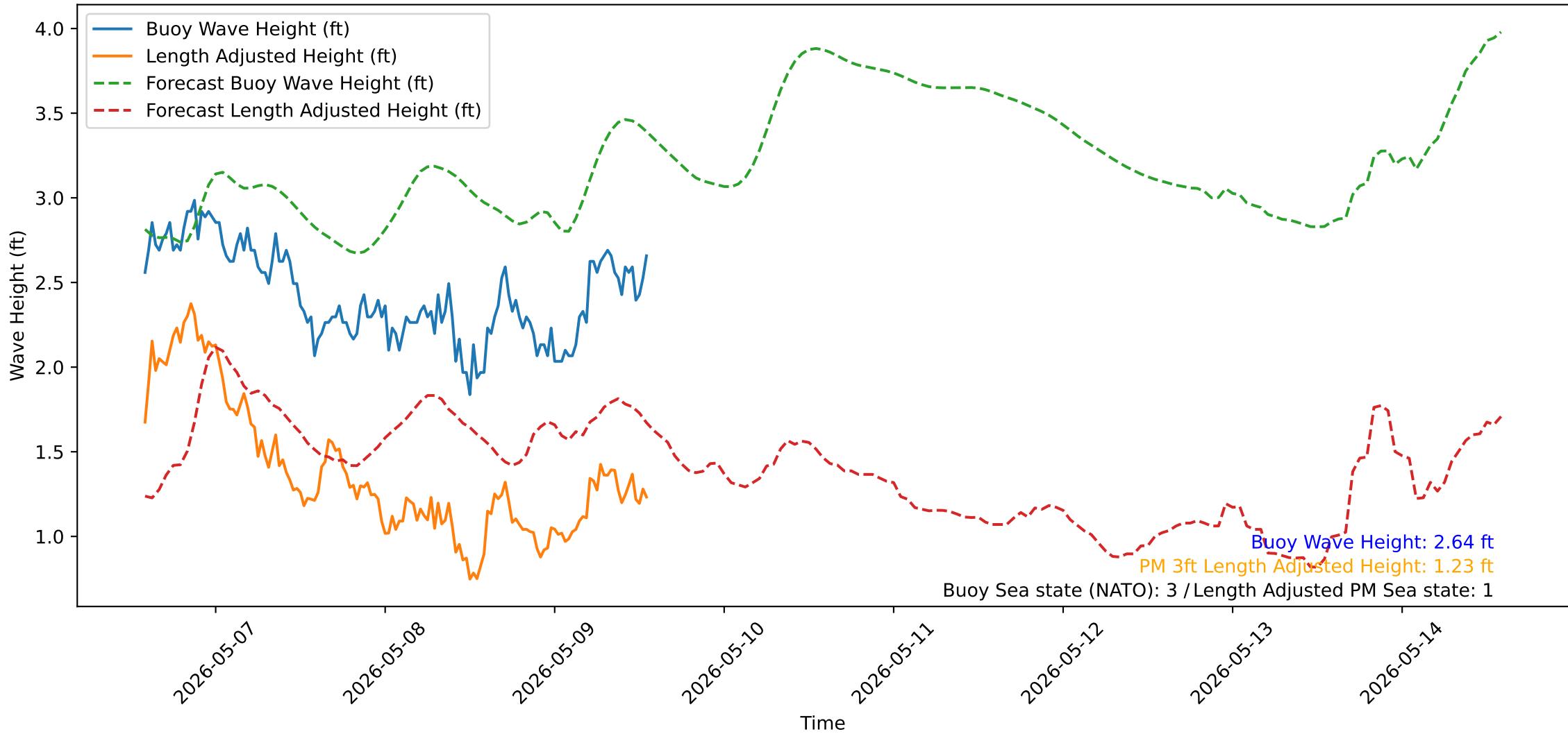
Wave Heights over Time for Green Beach at 2026-05-09 13:51:14
