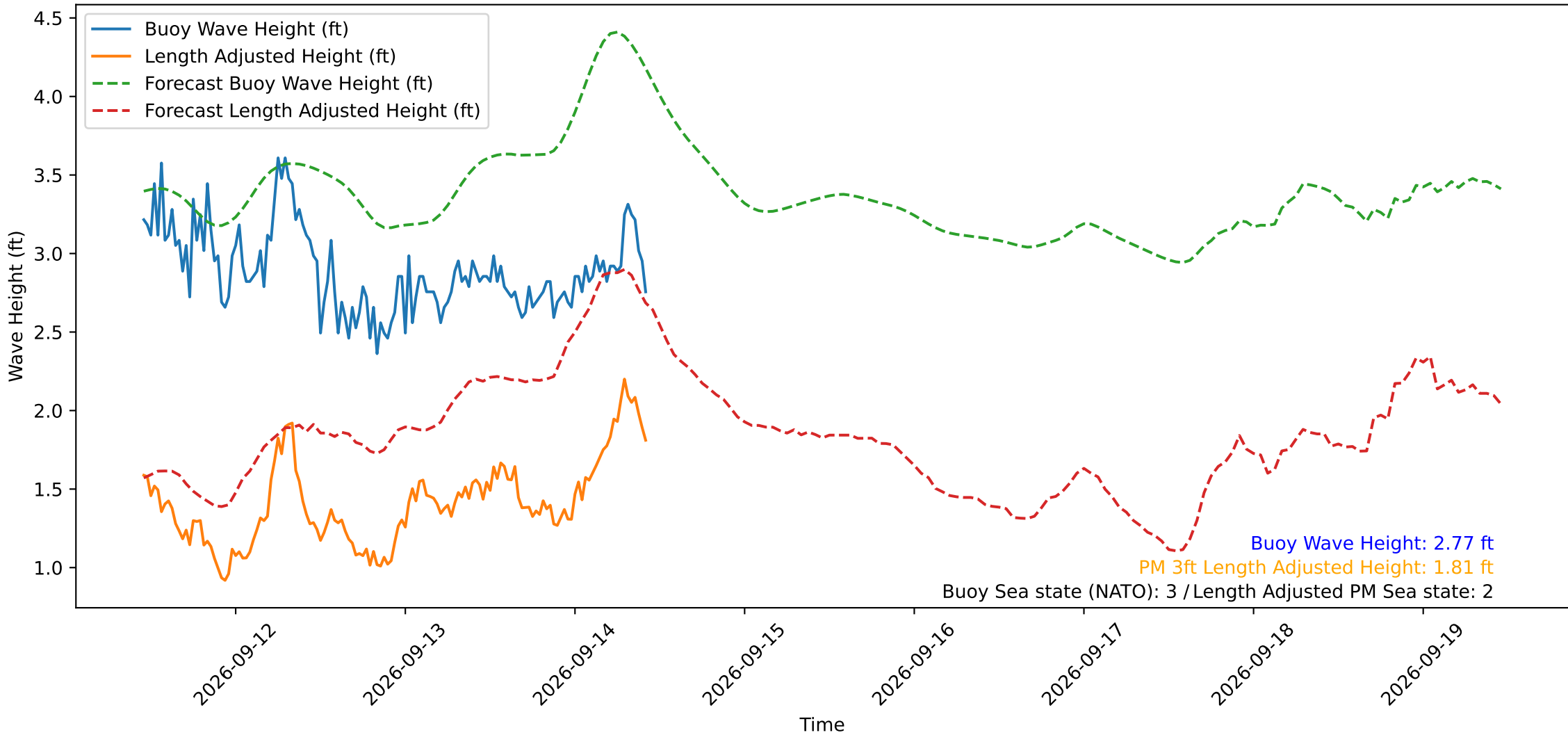
Wave Heights over Time for Green Beach at 2026-09-14 10:41:12
