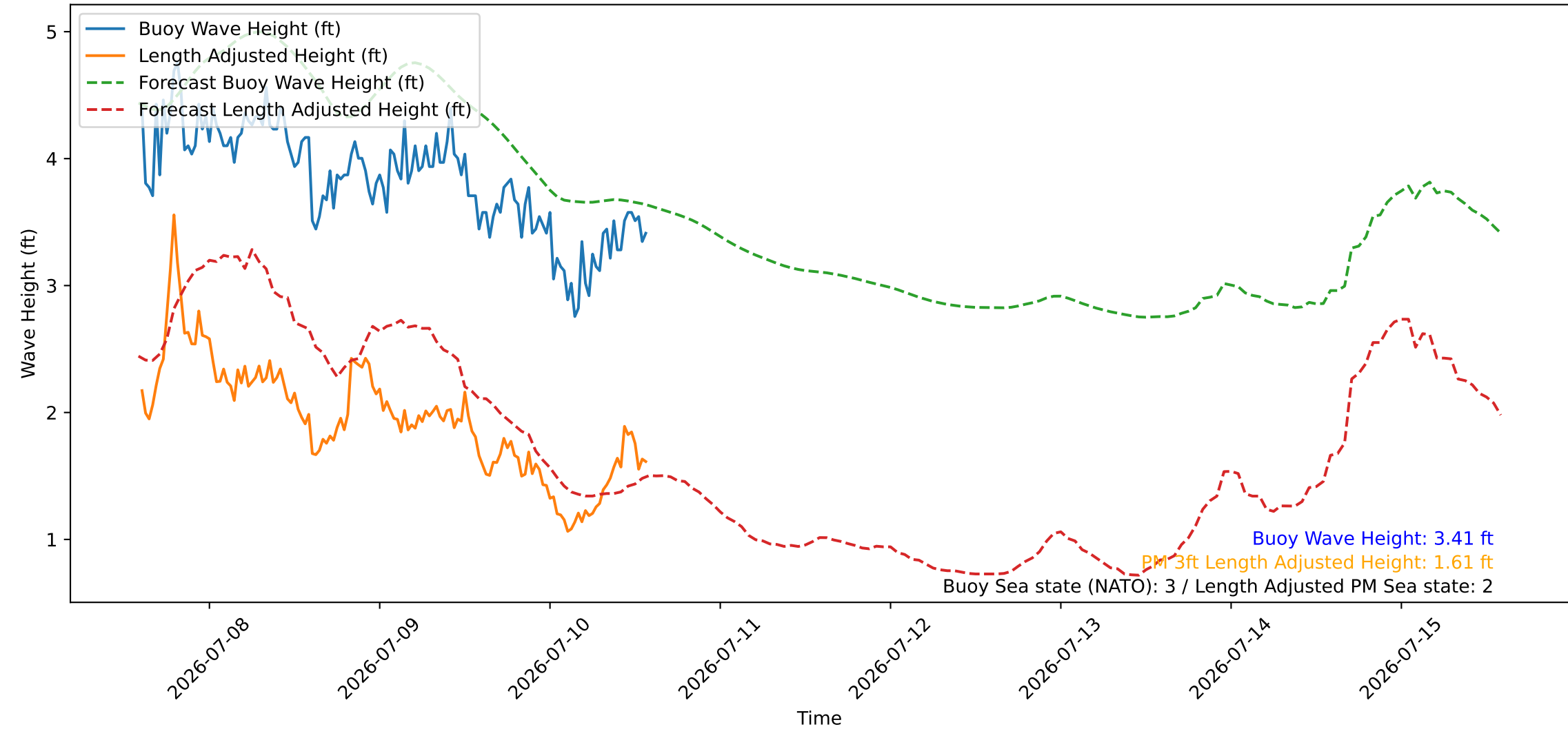
Wave Heights over Time for Green Beach at 2026-07-10 14:21:08
