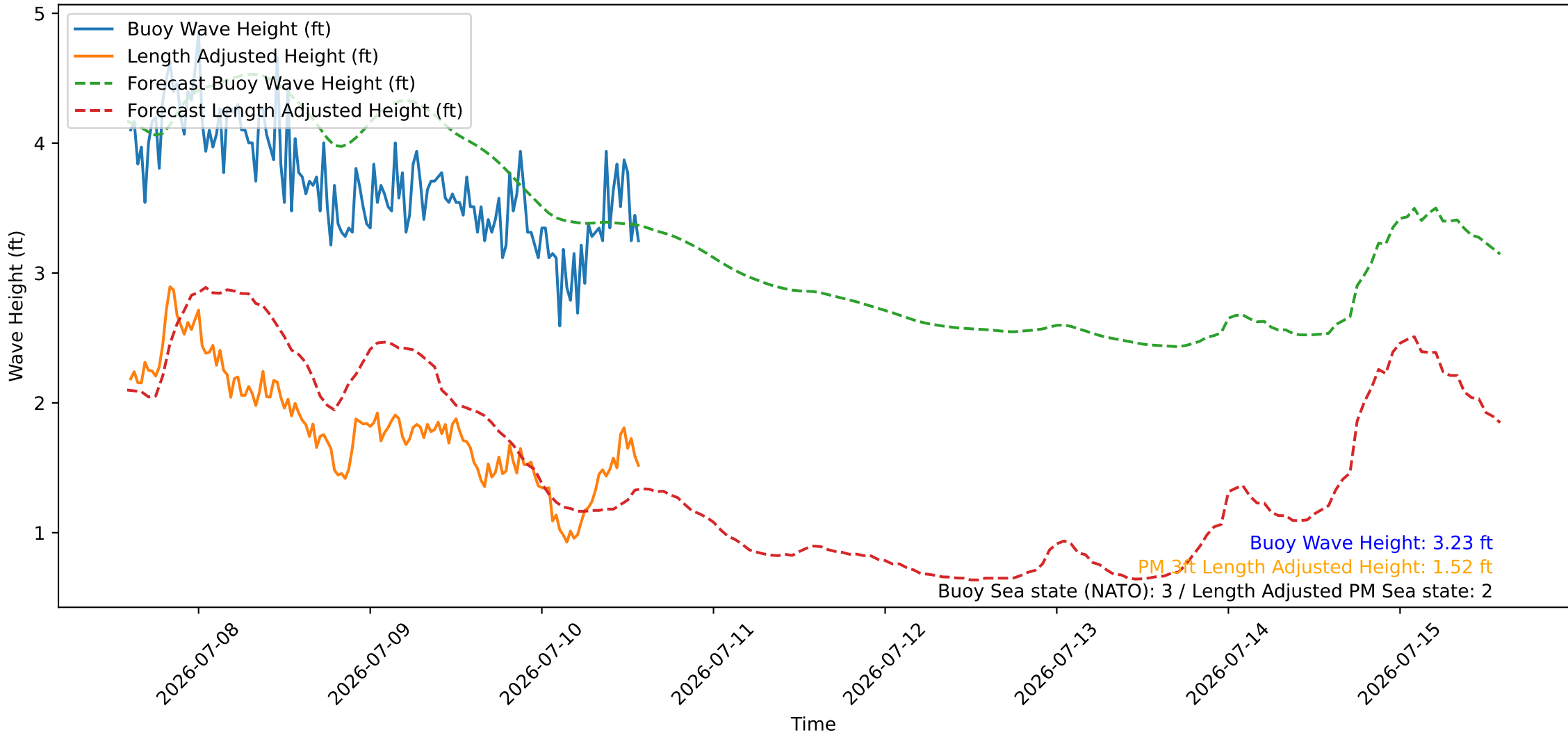
Wave Heights over Time for Red Beach at 2026-07-10 14:20:46
