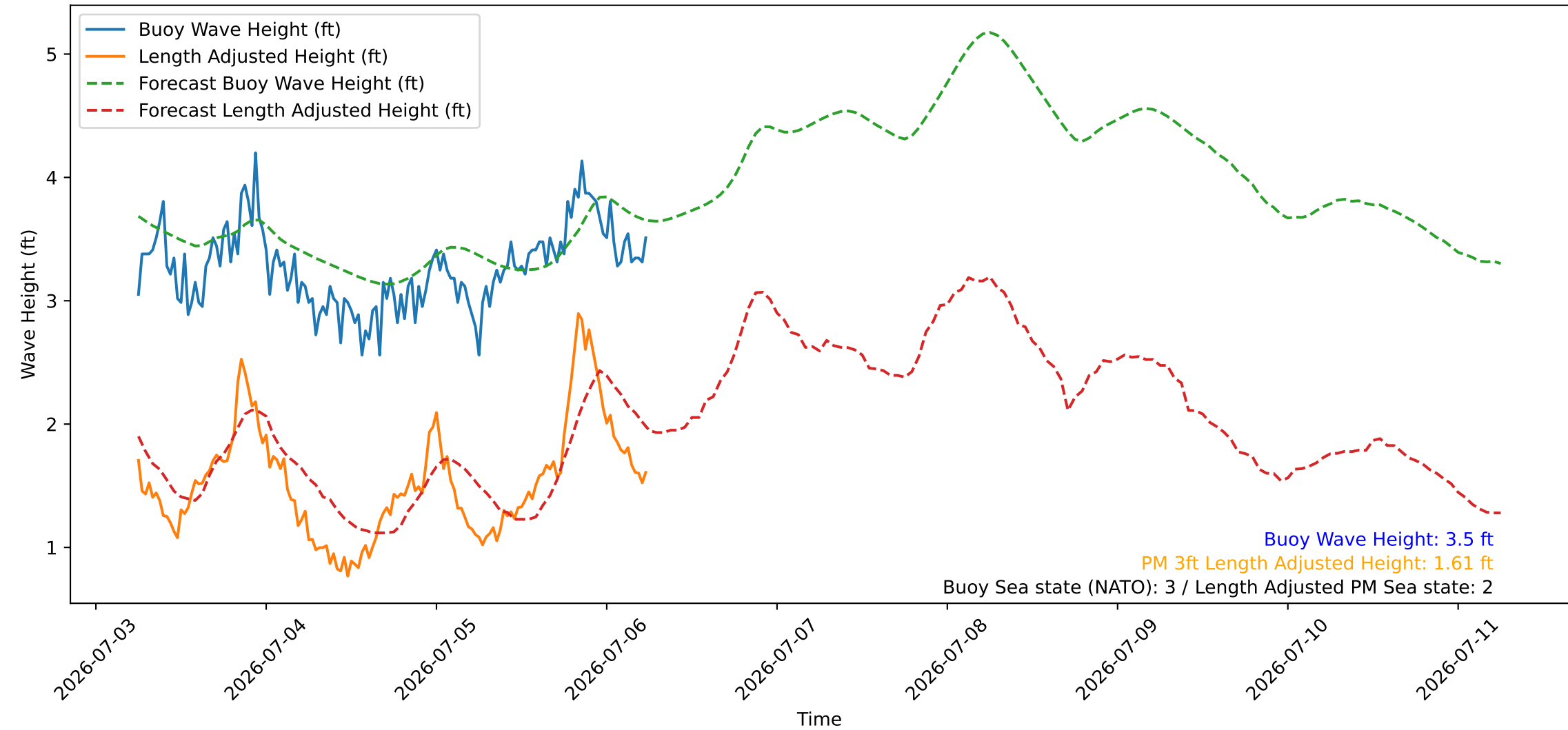
Wave Heights over Time for Green Beach at 2026-07-06 06:11:09
