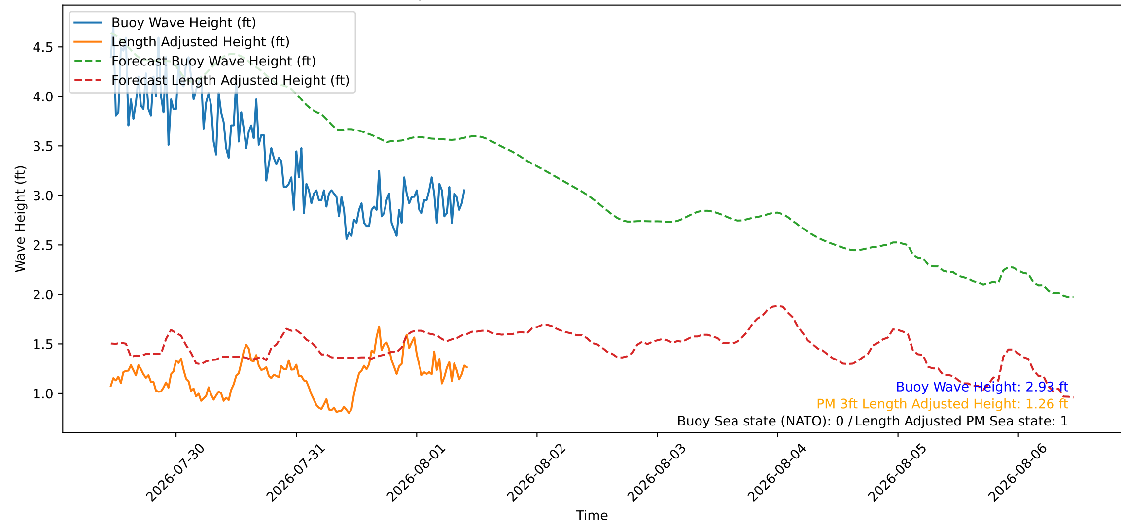
Wave Heights over Time for Red Beach at 2026-08-01 10:40:49
