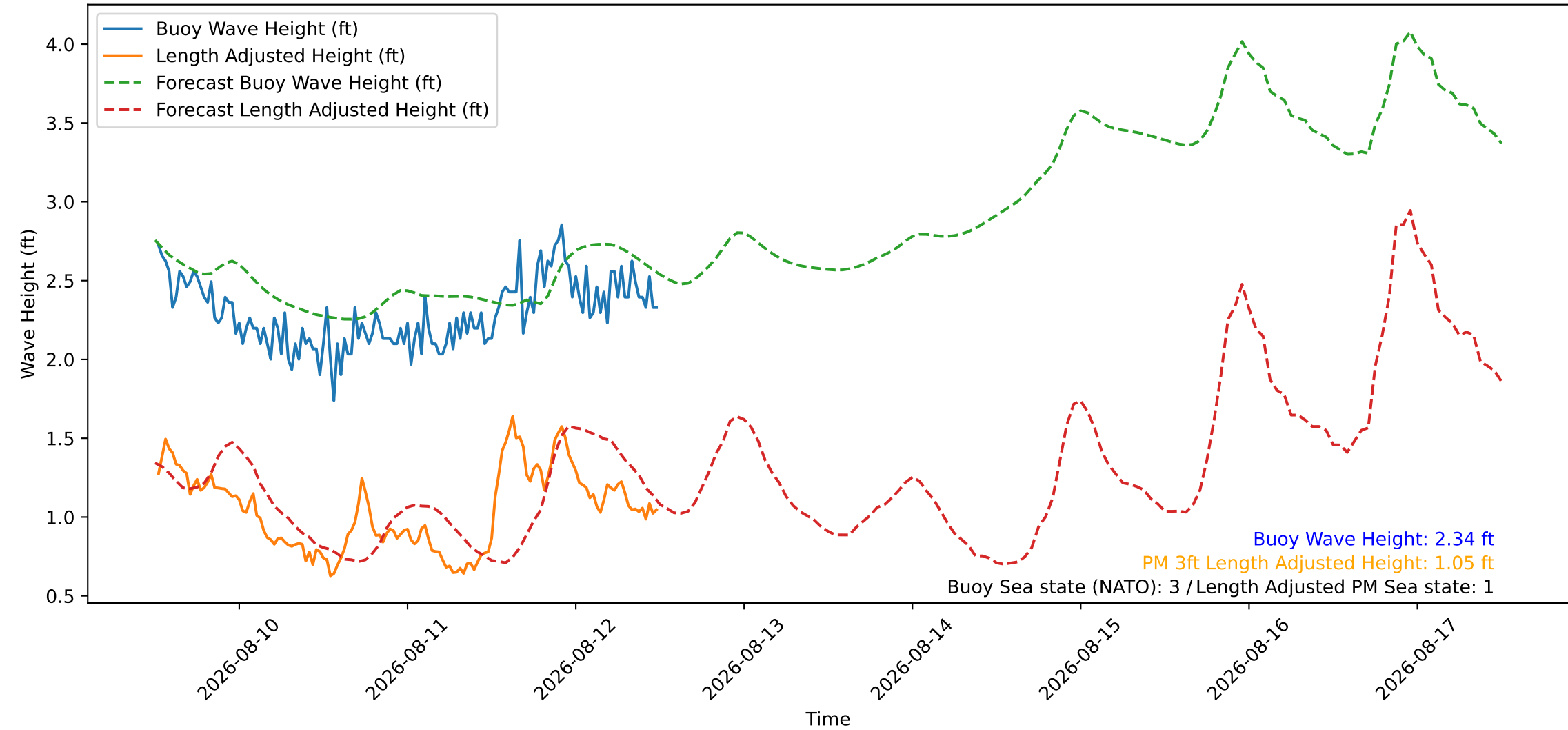
Wave Heights over Time for Red Beach at 2026-08-12 12:20:47
