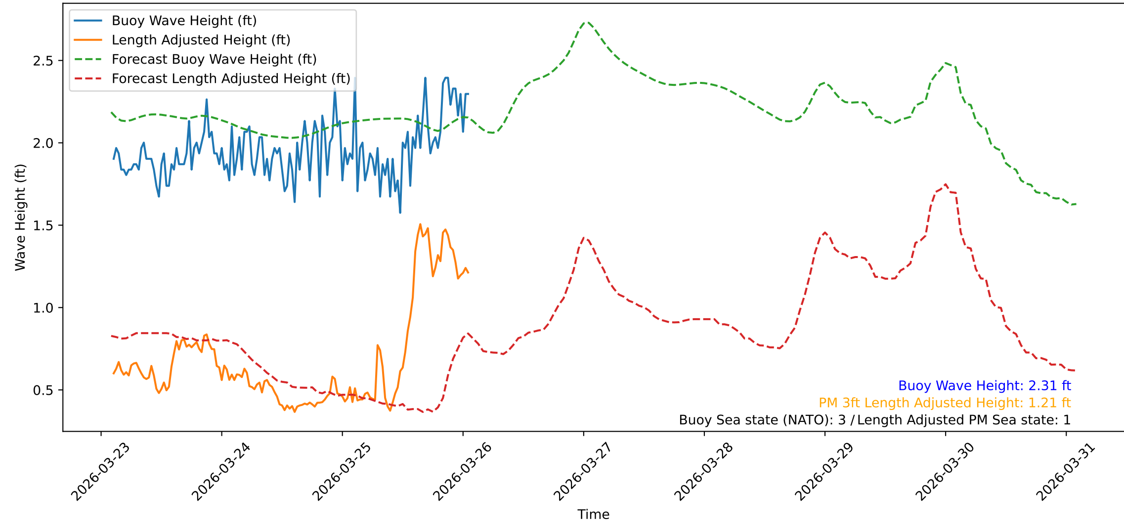
Wave Heights over Time for Red Beach at 2026-03-26 02:00:47
