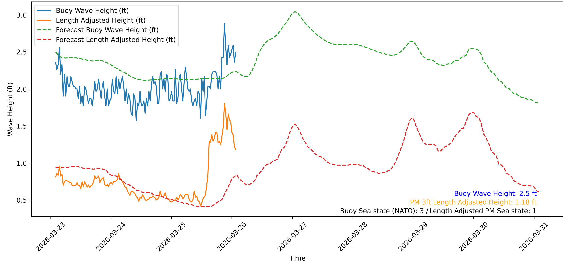
Wave Heights over Time for Oceanside Harbor at 2026-03-26 02:00:31
