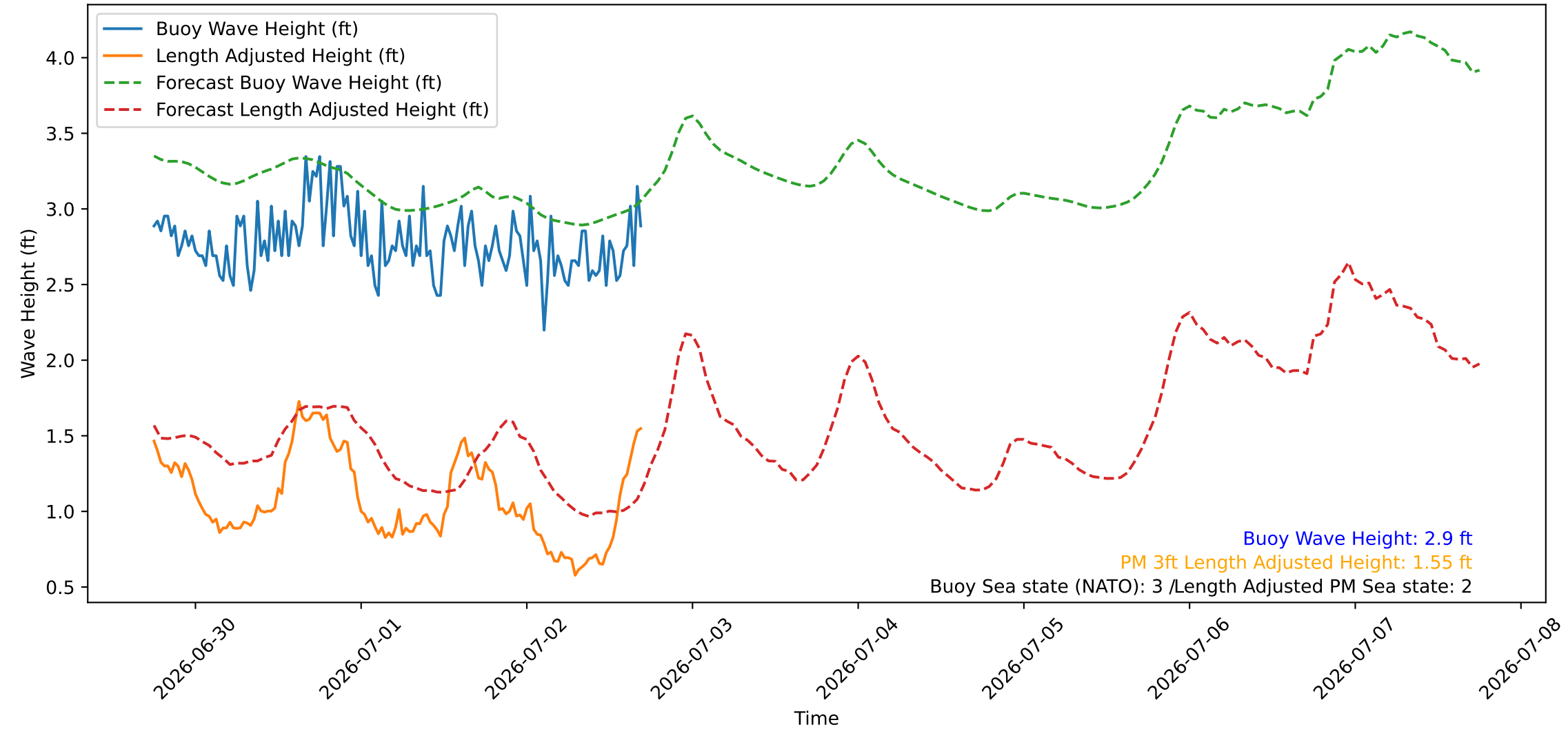
Wave Heights over Time for Red Beach at 2026-07-02 17:30:46
