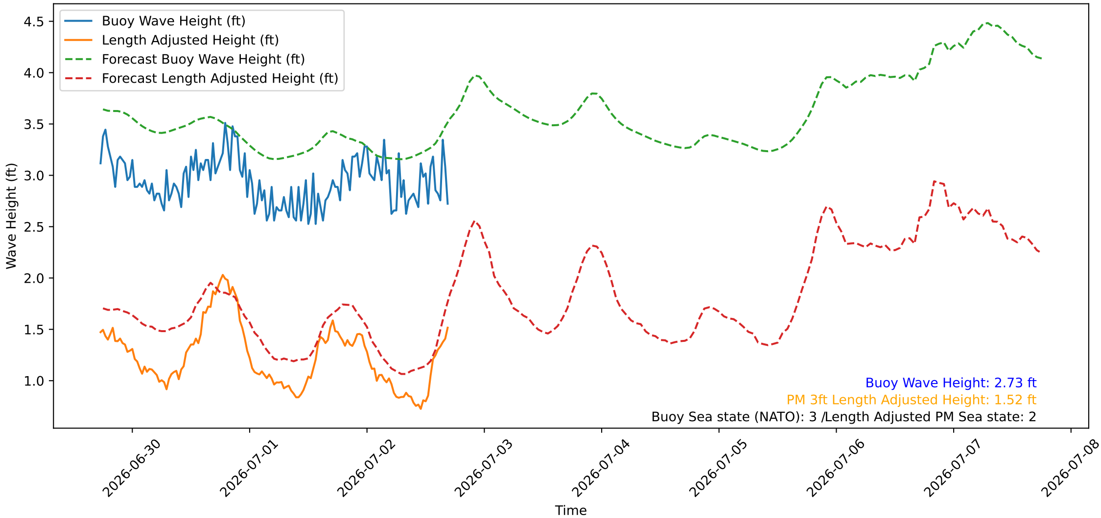
Wave Heights over Time for Green Beach at 2026-07-02 17:31:08
