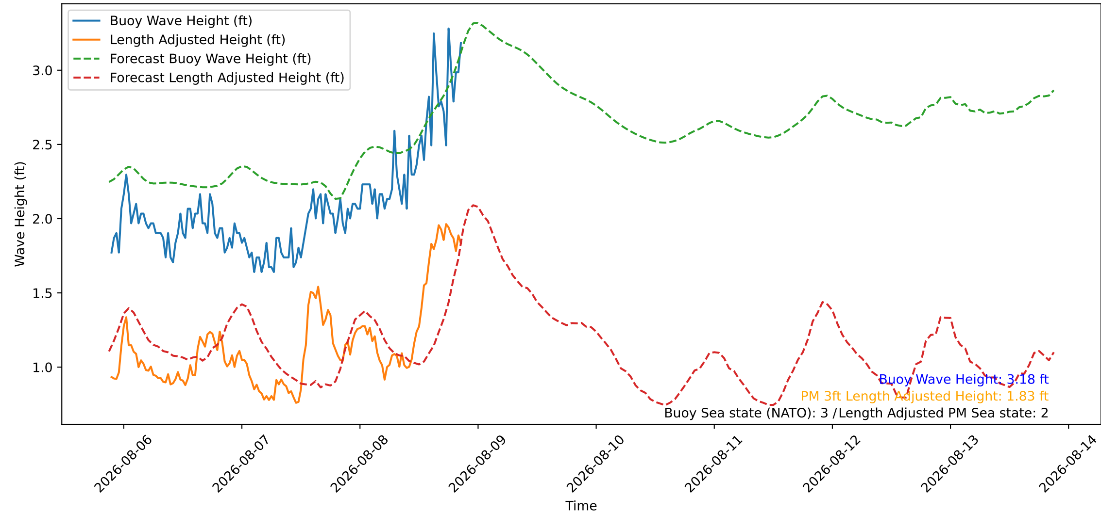
Wave Heights over Time for Oceanside Harbor at 2026-08-08 21:20:26
