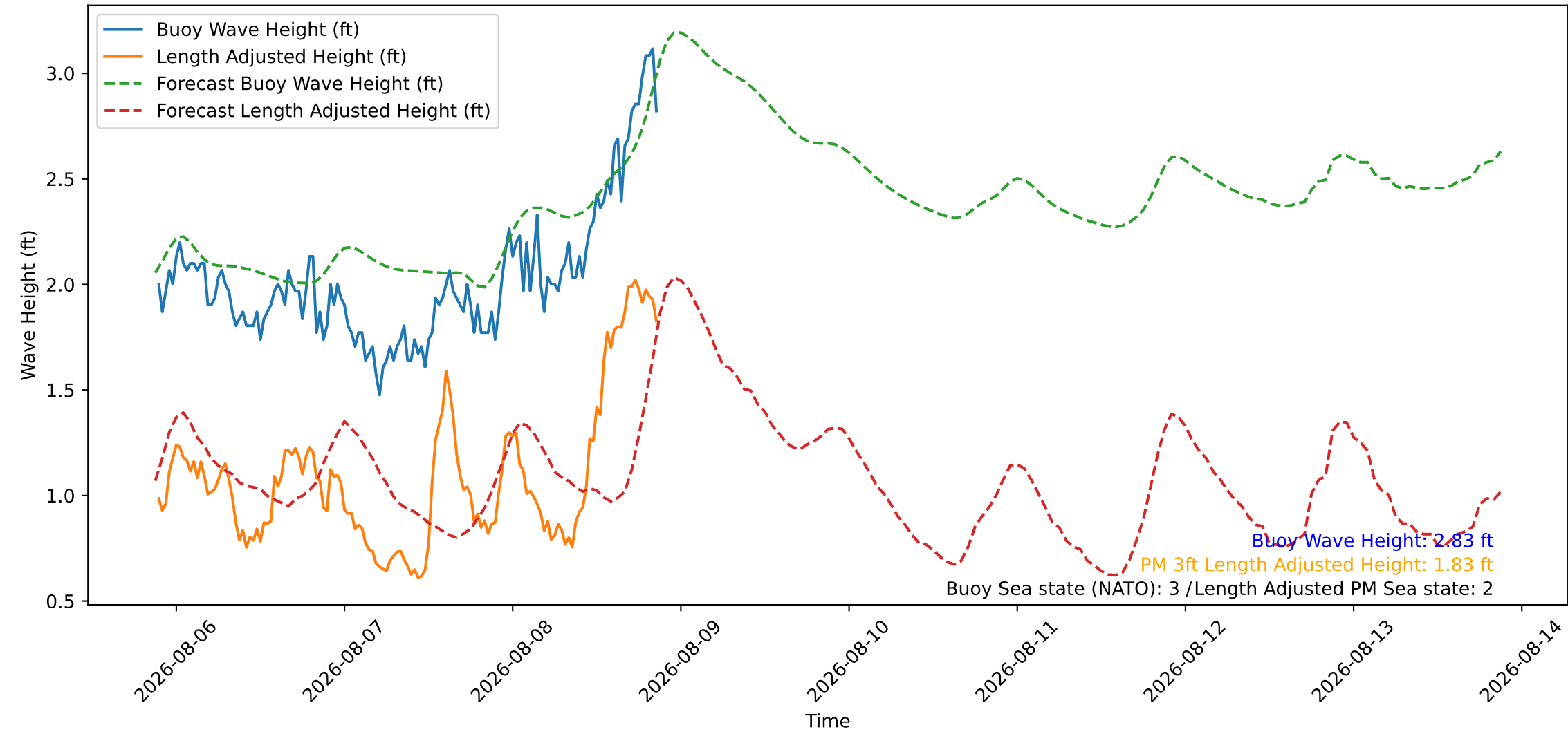
Wave Heights over Time for Red Beach at 2026-08-08 21:20:47
