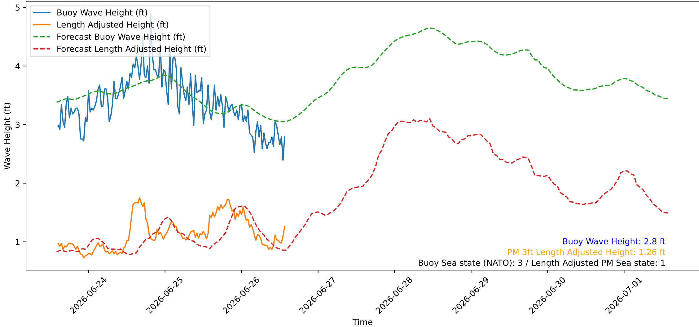
Wave Heights over Time for Oceanside Harbor at 2026-06-26 14:20:26
